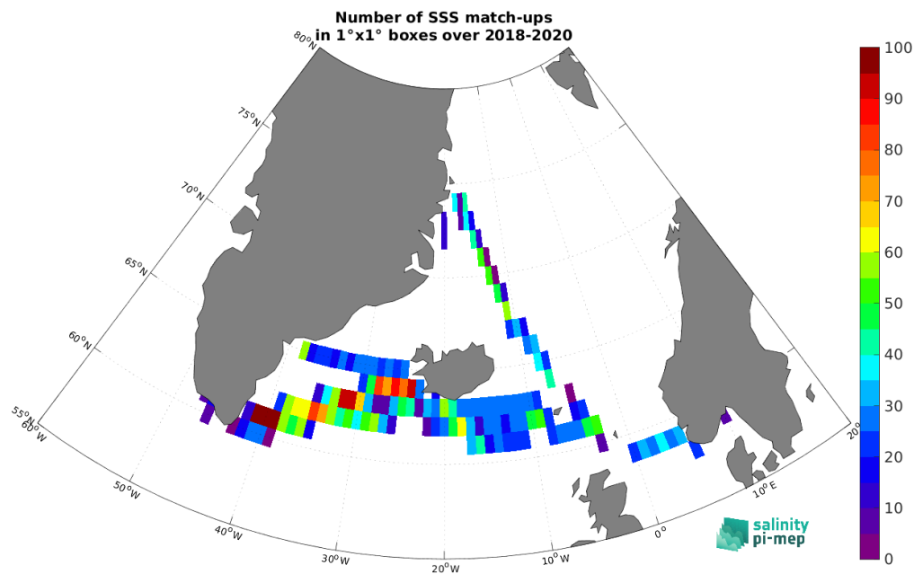
Figure 5: Number of SSS match-ups between TSG (Lauge-Koch) SSS and the CCI SSS L4 Merged-OI v5.5 - 30-day running (ESA) SSS product for the Global Ocean Pi-MEP region over 1^\circ \times 1^\circ boxes and for the full satellite product period.
