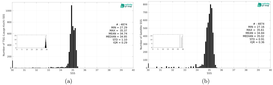
Figure 3: Histograms of SSS from TSG (Lauge-Koch) (a) and CCI SSS L4 Merged-OI v5.5 - 30-day running (ESA) (b) considering all match-up pairs per bins of 0.1 over the Global Ocean Pi-MEP region and for the full satellite product period.
