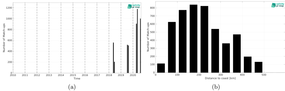
Figure 2: Number of match-ups between TSG (Lauge-Koch) and CCI SSS L4 Merged-OI v5.5 - 30-day running (ESA) SSS as a function of time (a) and as function of the distance to coast (b) over the Global Ocean Pi-MEP region and for the full satellite product period.
