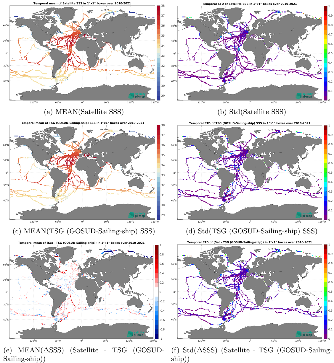
Figure 7: Temporal mean (left) and Std (right) of SSS from CCI SSS L4 Merged-OI v5.5 - 30-day running (ESA) (top), TSG (GOSUD-Sailing-ship) (middle), and of \Delta SSS (Satellite - TSG (GOSUD-Sailing-ship)). Only match-up pairs are used to generate these maps.
