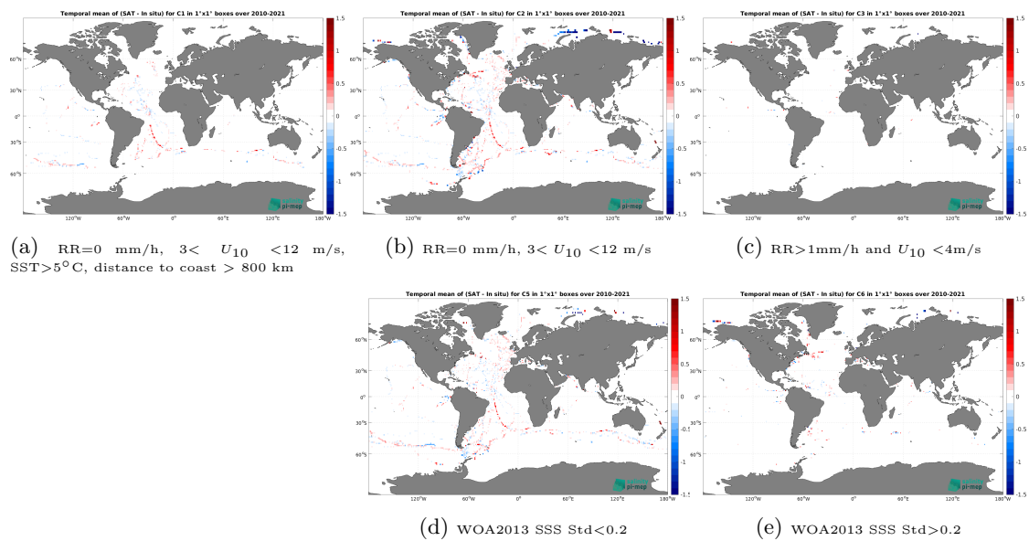
Figure 14: Temporal mean gridded over spatial boxes of size 1^\circ \times 1^\circ of \Delta SSS (CCI SSS L4 Merged-OI v5.5 - 30-day running (ESA) - TSG (GOSUD-Sailing-ship)) for 5 different subdatasets corresponding to: RR=0 mm/h, 3 < U_{10} < 12 m/s, SST > 5^\circ\text{C} , distance to coast > 800 km (a), RR=0 mm/h, 3 < U_{10} < 12 m/s (b), RR > 1 mm/h and U_{10} < 4 m/s (c), WOA2013 SSS Std < 0.2 (d), WOA2013 SSS Std > 0.2 (e).
