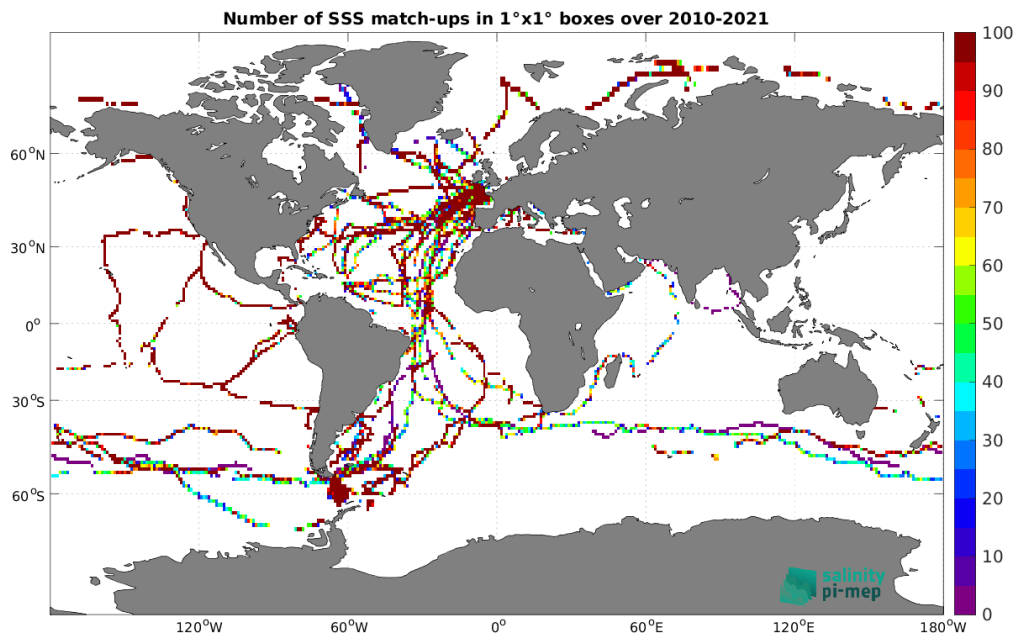
Figure 5: Number of SSS match-ups between TSG (GOSUD-Sailing-ship) SSS and the CCI SSS L4 Merged-OI v5.5 - 30-day running (ESA) SSS product for the Global Ocean Pi-MEP region over 1^\circ \times 1^\circ boxes and for the full satellite product period.
