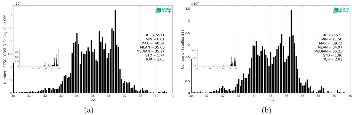
Figure 3: Histograms of SSS from TSG (GOSUD-Sailing-ship) (a) and CCI SSS L4 Merged-OI v5.5 - 30-day running (ESA) (b) considering all match-up pairs per bins of 0.1 over the Global Ocean Pi-MEP region and for the full satellite product period.
