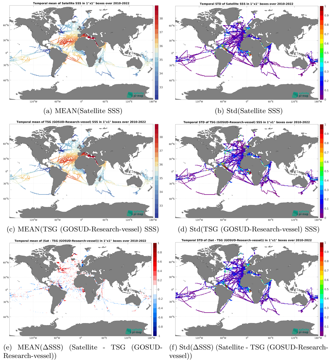
Figure 7: Temporal mean (left) and Std (right) of SSS from CCI SSS L4 Merged-OI v5.5 - 30-day running (ESA) (top), TSG (GOSUD-Research-vessel) (middle), and of \Delta SSS (Satellite - TSG (GOSUD-Research-vessel)). Only match-up pairs are used to generate these maps.
