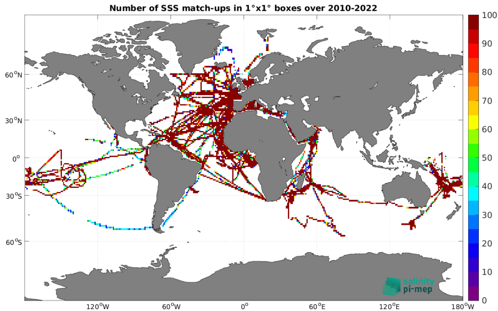
Figure 5: Number of SSS match-ups between TSG (GOSUD-Research-vessel) SSS and the CCI SSS L4 Merged-OI v5.5 - 30-day running (ESA) SSS product for the Global Ocean Pi-MEP region over 1^\circ \times 1^\circ boxes and for the full satellite product period.
