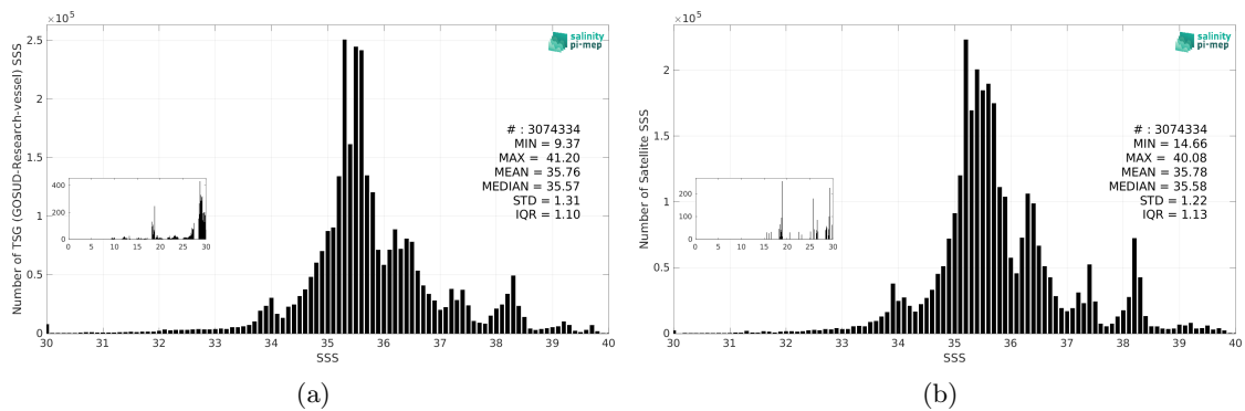
Figure 3: Histograms of SSS from TSG (GOSUD-Research-vessel) (a) and CCI SSS L4 Merged-OI v5.5 - 30-day running (ESA) (b) considering all match-up pairs per bins of 0.1 over the Global Ocean Pi-MEP region and for the full satellite product period.
