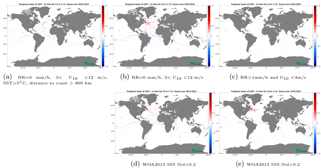
Figure 14: Temporal mean gridded over spatial boxes of size 1^\circ \times 1^\circ of \Delta SSS (CCI SSS L4 Merged-OI v5.5 - 30-day running (ESA) - TSG (GOSUD-Research-vessel)) for 5 different subdatasets corresponding to:RR=0 mm/h, 3 < U_{10} < 12 m/s, SST > 5^\circ\text{C} , distance to coast > 800 km (a), RR=0 mm/h, 3 < U_{10} < 12 m/s (b), RR > 1 mm/h and U_{10} < 4 m/s (c), WOA2013 SSS Std < 0.2 (d), WOA2013 SSS Std > 0.2 (e).
