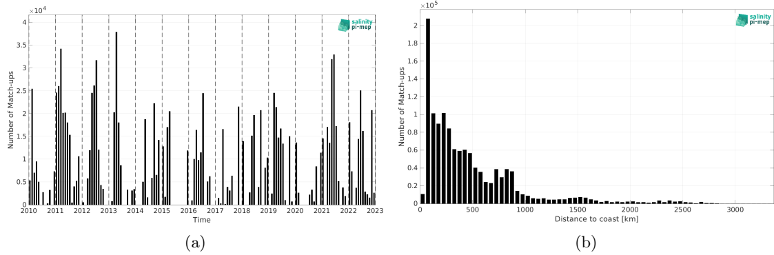
Figure 2: Number of match-ups between TSG (CSIC-UTM) and CCI SSS L4 Merged-OI v5.5 - 30-day running (ESA) SSS as a function of time (a) and as function of the distance to coast (b) over the Global Ocean Pi-MEP region and for the full satellite product period.
