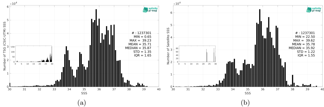
Figure 3: Histograms of SSS from TSG (CSIC-UTM) (a) and CCI SSS L4 Merged-OI v5.5 - 30-day running (ESA) (b) considering all match-up pairs per bins of 0.1 over the Global Ocean Pi-MEP region and for the full satellite product period.
