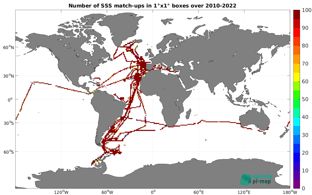
Figure 5: Number of SSS match-ups between TSG (CSIC-UTM) SSS and the CCI SSS L4 Merged-OI v5.5 - 30-day running (ESA) SSS product for the Global Ocean Pi-MEP region over 1^\circ \times 1^\circ boxes and for the full satellite product period.
