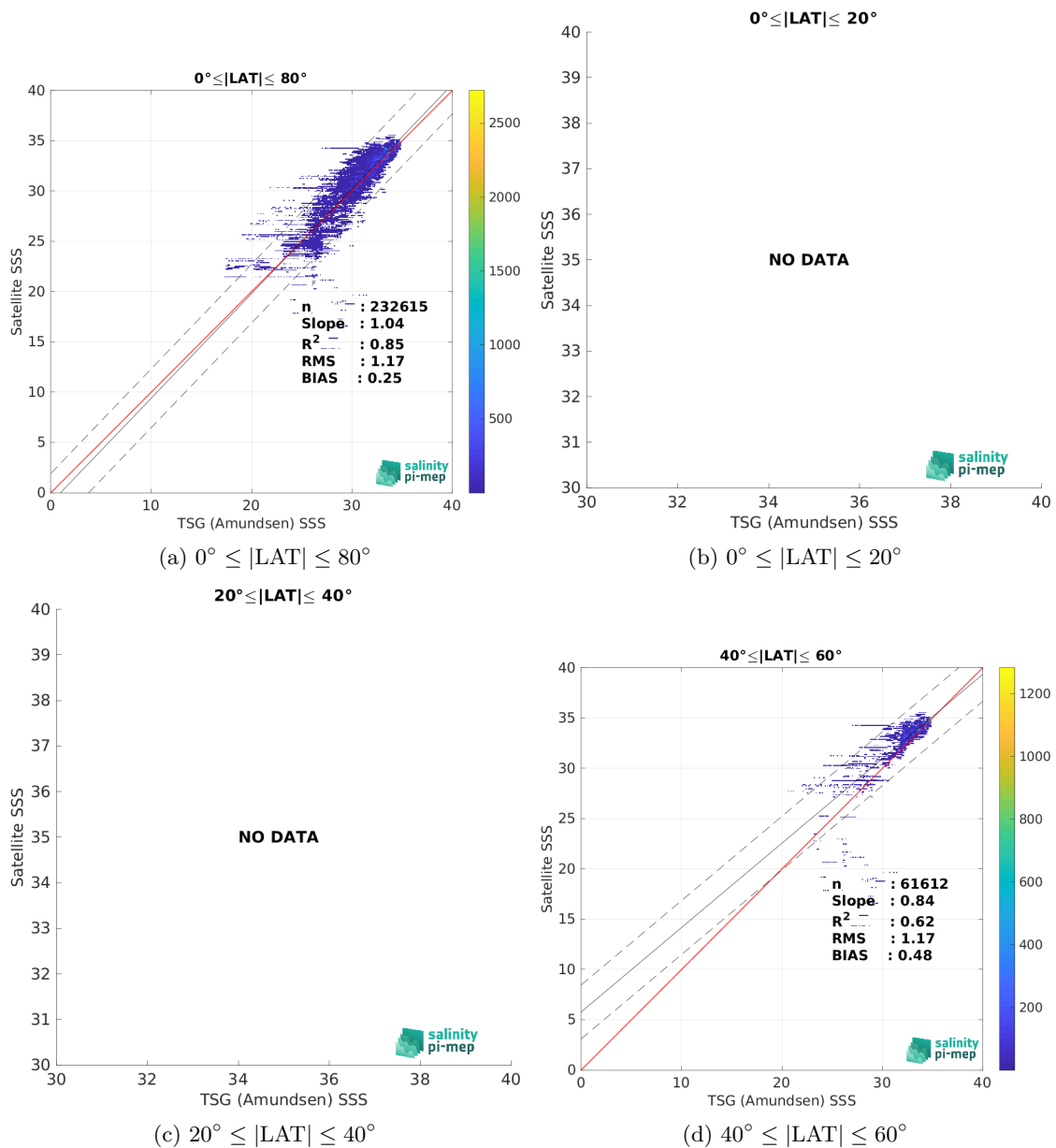
Figure 10: Contour maps of the concentration of CCI SSS L4 Merged-OI v5.5 - 30-day running (ESA) SSS (y-axis) versus TSG (Amundsen) SSS (x-axis) at match-up pairs for different latitude bands. For each plot, the red line shows x=y . The black thin and dashed lines indicate a linear fit through the data cloud and the \pm 95\% confidence levels, respectively. The number match-up pairs n , the slope and R^2 coefficient of the linear fit, the root mean square (RMS) and the mean bias between satellite and in situ data are indicated for each latitude band in each plots.
