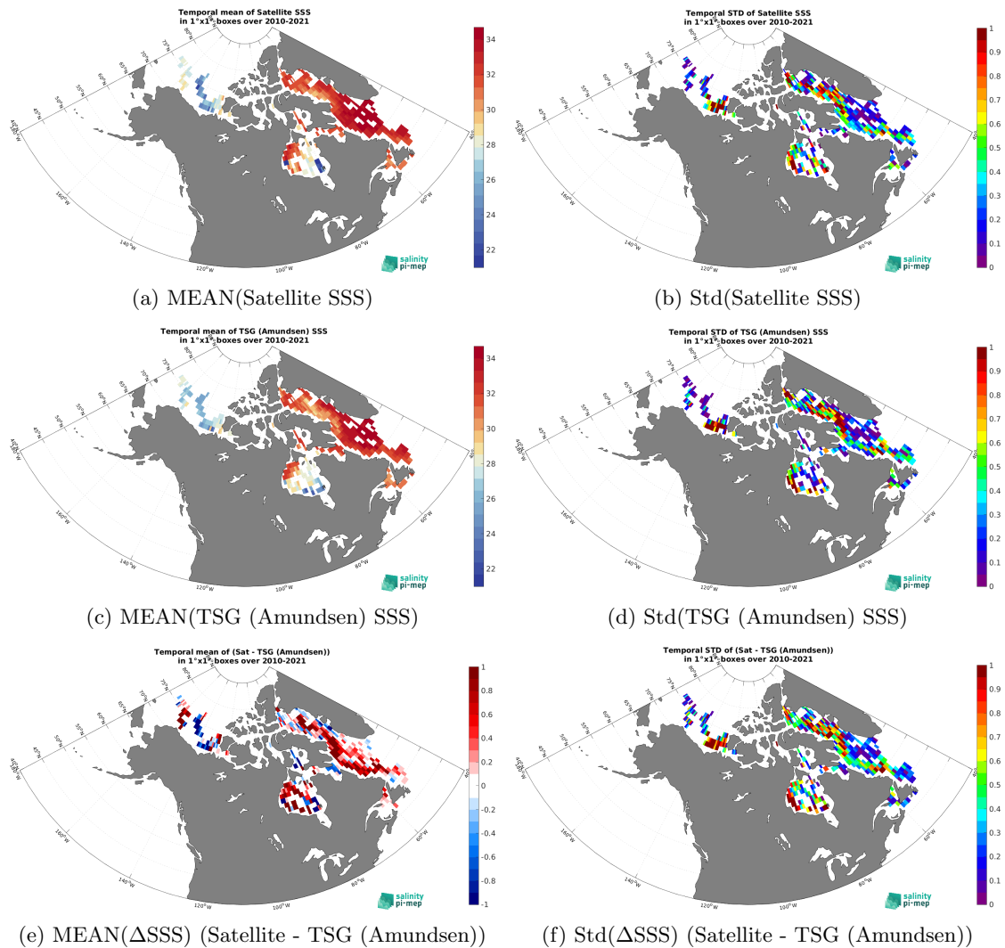
Figure 7: Temporal mean (left) and Std (right) of SSS from CCI SSS L4 Merged-OI v5.5 - 30-day running (ESA) (top), TSG (Amundsen) (middle), and of \Delta SSS (Satellite - TSG (Amundsen)). Only match-up pairs are used to generate these maps.
