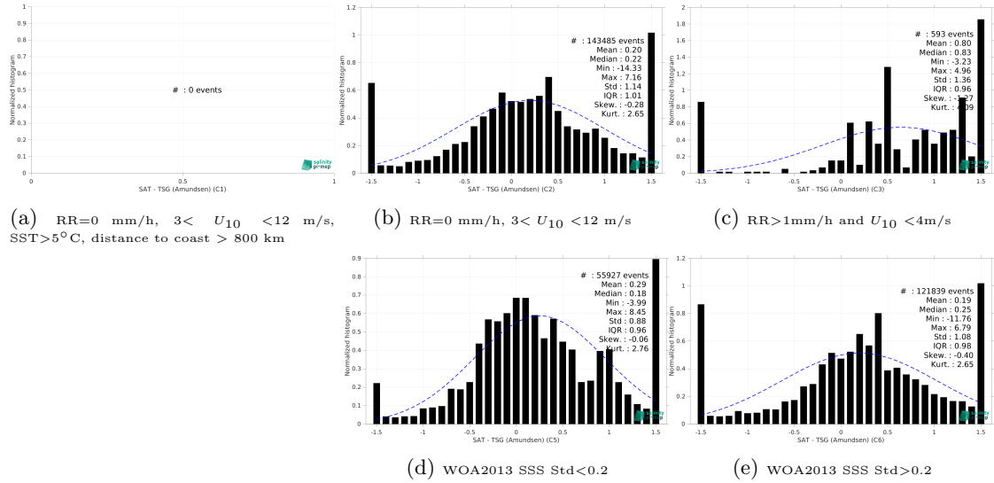
Figure 15: Normalized histogram of \Delta SSS (CCI SSS L4 Merged-OI v5.5 - 30-day running (ESA) - TSG (Amundsen)) for 5 different subdatasets corresponding to: RR=0 mm/h, 3 < U_{10} < 12 m/s, SST > 5°C, distance to coast > 800 km (a), RR=0 mm/h, 3 < U_{10} < 12 m/s (b), RR > 1mm/h and U_{10} < 4 m/s (c), WOA2013 SSS Std < 0.2 (d), WOA2013 SSS Std > 0.2 (e).
