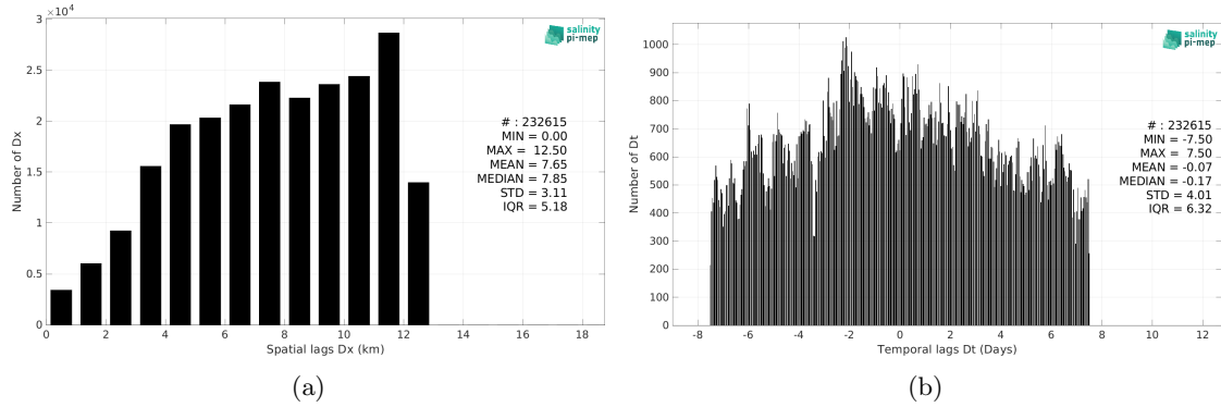
Figure 6: Histograms of the spatial (a) and temporal (b) lags between the location/time of the TSG (Amundsen) measurement and the date of the corresponding CCI SSS L4 Merged-OI v5.5 - 30-day running (ESA) SSS pixel.
