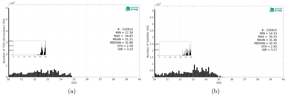
Figure 3: Histograms of SSS from TSG (Amundsen) (a) and CCI SSS L4 Merged-OI v5.5 - 30-day running (ESA) (b) considering all match-up pairs per bins of 0.1 over the Global Ocean Pi-MEP region and for the full satellite product period.
