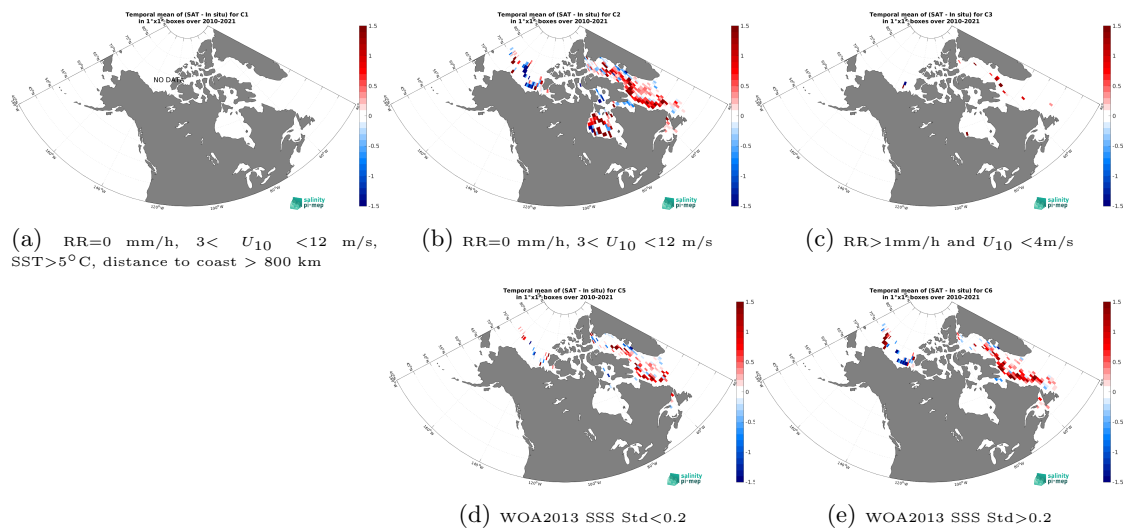
Figure 14: Temporal mean gridded over spatial boxes of size 1^\circ \times 1^\circ of \Delta\text{SSS} (CCI SSS L4 Merged-OI v5.5 - 30-day running (ESA) - TSG (Amundsen)) for 5 different subdatasets corresponding to: RR=0 mm/h, 3 < U_{10} < 12 m/s, SST > 5°C, distance to coast > 800 km (a), RR=0 mm/h, 3 < U_{10} < 12 m/s (b), RR > 1mm/h and U_{10} < 4 m/s (c), WOA2013 SSS Std < 0.2 (d), WOA2013 SSS Std > 0.2 (e).
