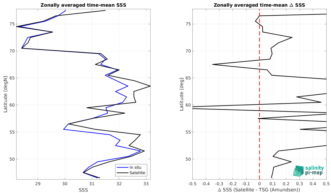
Figure 9: Left panel: Zonal mean SSS from CCI SSS L4 Merged-OI v5.5 - 30-day running (ESA) satellite product (black) and from TSG (Amundsen) (blue). Right panel: Zonal mean of \Delta SSS (Satellite - TSG (Amundsen)) for all the collected Pi-MEP match-up pairs estimated over the full satellite product period.
