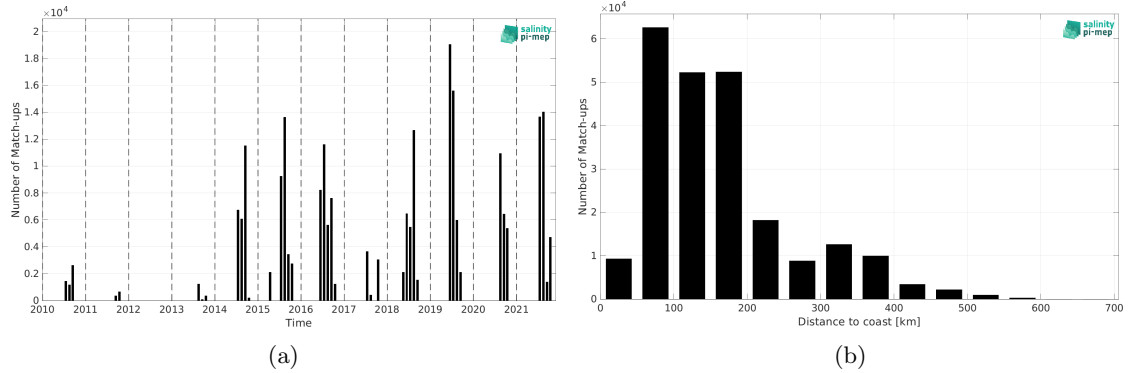
Figure 2: Number of match-ups between TSG (Amundsen) and CCI SSS L4 Merged-OI v5.5 - 30-day running (ESA) SSS as a function of time (a) and as function of the distance to coast (b) over the Global Ocean Pi-MEP region and for the full satellite product period.
