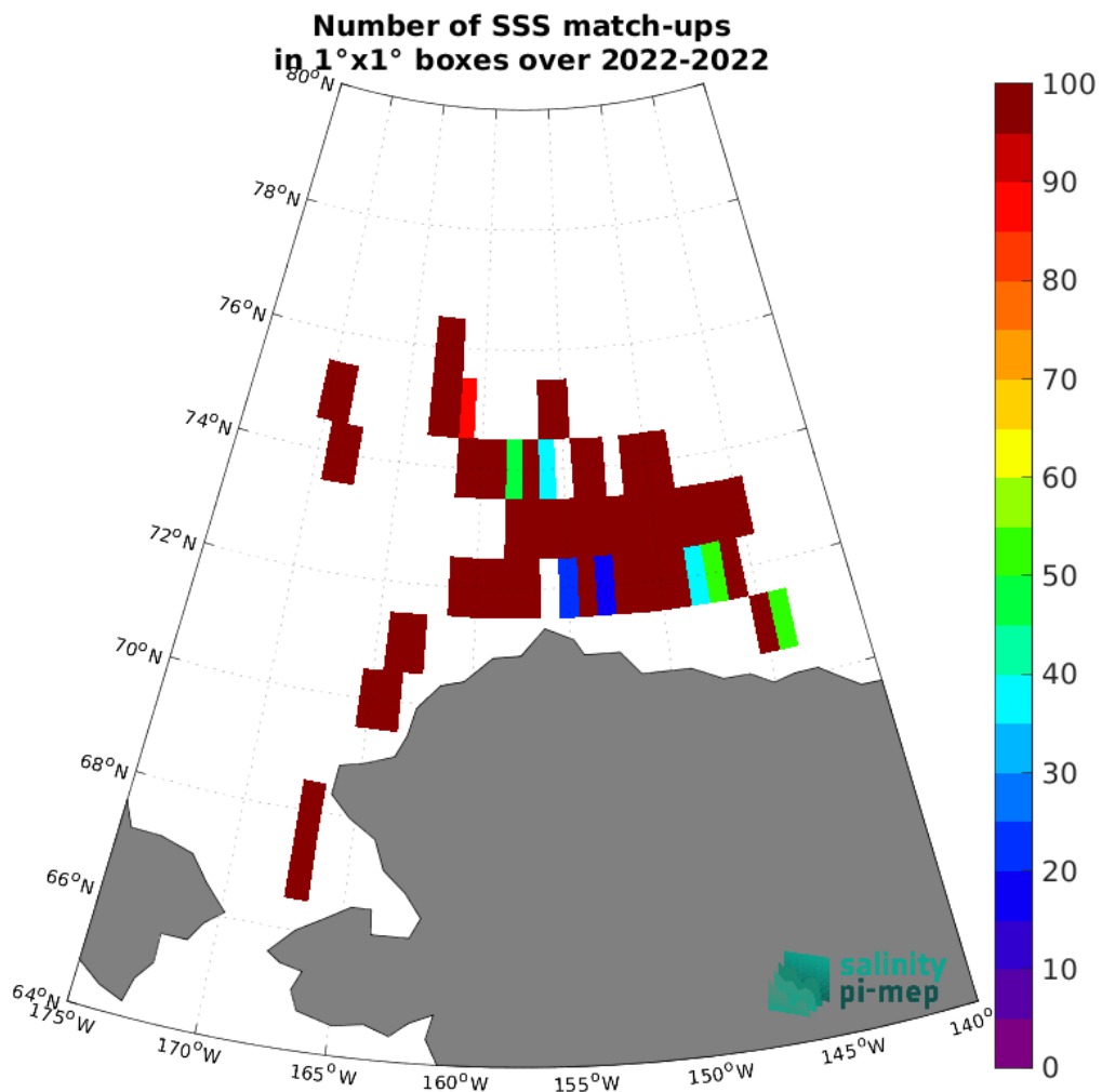
Figure 5: Number of SSS match-ups between SASSIE SSS and the CCI SSS L4 Merged-OI v5.5 - 30-day running (ESA) SSS product for the Global Ocean Pi-MEP region over 1^\circ \times 1^\circ boxes and for the full satellite product period.
