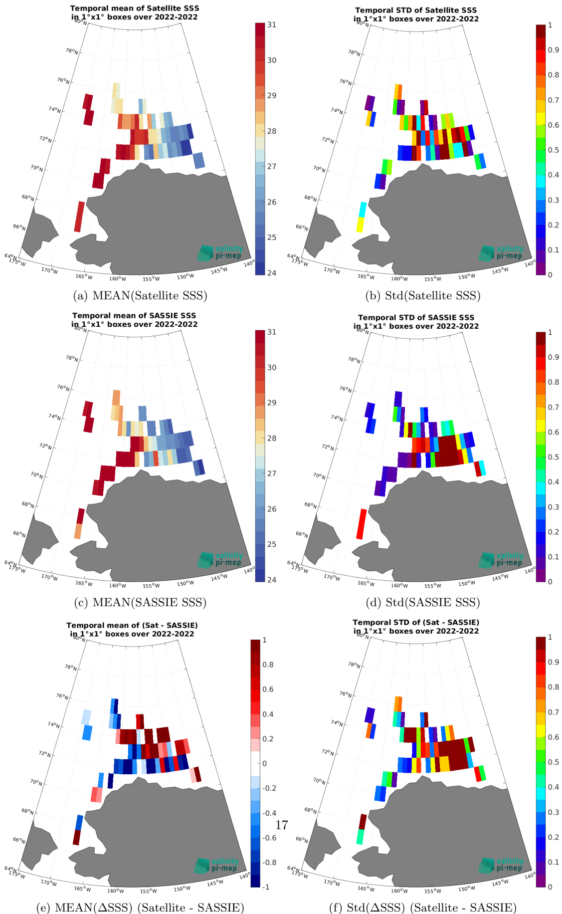
Figure 7: Temporal mean (left) and Std (right) of SSS from CCI SSS L4 Merged-OI v5.5 - 30-day running (ESA) (top), SASSIE (middle), and of \Delta SSS (Satellite - SASSIE). Only match-up pairs are used to generate these maps.
