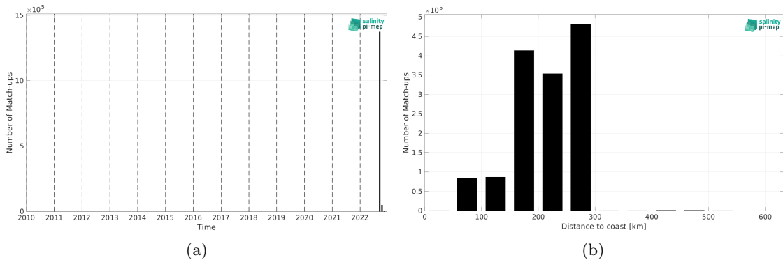
Figure 2: Number of match-ups between SASSIE and CCI SSS L4 Merged-OI v5.5 - 30-day running (ESA) SSS as a function of time (a) and as function of the distance to coast (b) over the Global Ocean Pi-MEP region and for the full satellite product period.
