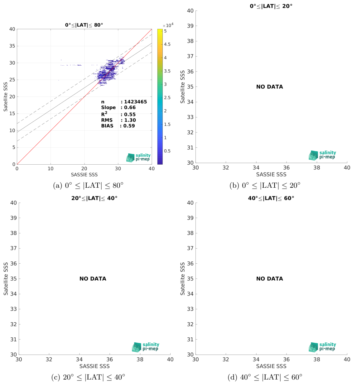
Figure 10: Contour maps of the concentration of CCI SSS L4 Merged-OI v5.5 - 30-day running (ESA) SSS (y-axis) versus SASSIE SSS (x-axis) at match-up pairs for different latitude bands. For each plot, the red line shows x=y . The black thin and dashed lines indicate a linear fit through the data cloud and the \pm 95\% confidence levels, respectively. The number match-up pairs n , the slope and R^2 coefficient of the linear fit, the root mean square (RMS) and the mean bias between satellite and in situ data are indicated for each latitude band in each plots.
