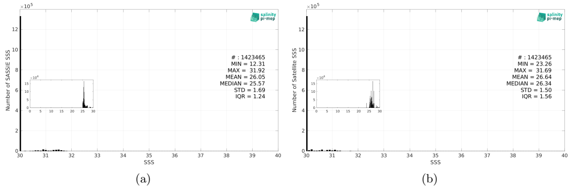
Figure 3: Histograms of SSS from SASSIE (a) and CCI SSS L4 Merged-OI v5.5 - 30-day running (ESA) (b) considering all match-up pairs per bins of 0.1 over the Global Ocean Pi-MEP region and for the full satellite product period.
