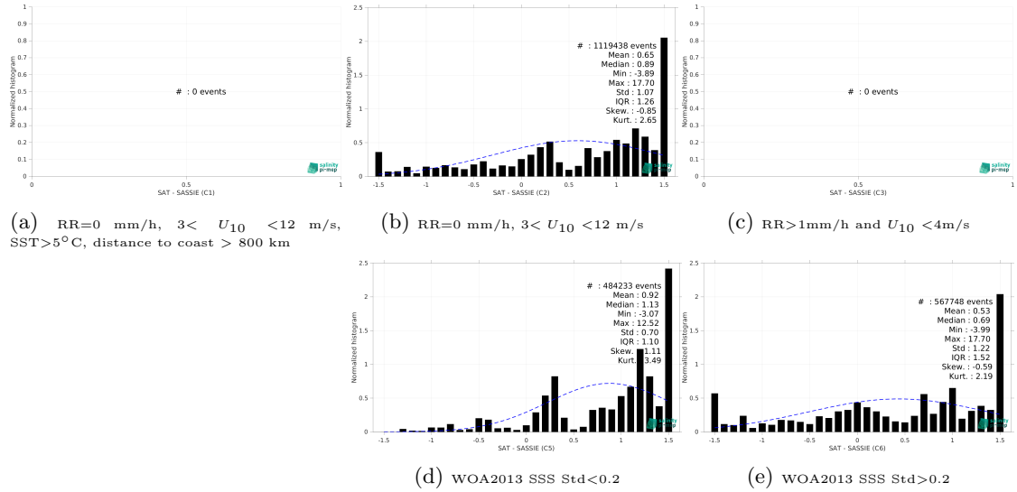
Figure 15: Normalized histogram of \Delta SSS (CCI SSS L4 Merged-OI v5.5 - 30-day running (ESA) - SASSIE) for 5 different subdatasets corresponding to: RR=0 mm/h, 3 < U_{10} < 12 m/s, SST > 5°C, distance to coast > 800 km (a), RR=0 mm/h, 3 < U_{10} < 12 m/s (b), RR > 1mm/h and U_{10} < 4 m/s (c), WOA2013 SSS Std < 0.2 (d), WOA2013 SSS Std > 0.2 (e).
