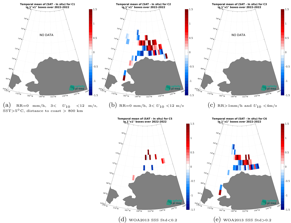
Figure 14: Temporal mean gridded over spatial boxes of size 1^\circ \times 1^\circ of \Delta SSS (CCI SSS L4 Merged-OI v5.5 - 30-day running (ESA) - SASSIE) for 5 different subdatasets corresponding to:RR=0 mm/h, 3 < U_{10} < 12 m/s, SST >5^\circ C, distance to coast > 800 km (a), RR=0 mm/h, 3 < U_{10} < 12 m/s (b), RR >1 mm/h and U_{10} < 4 m/s (c), WOA2013 SSS Std <0.2 (d), WOA2013 SSS Std >0.2 (e).
