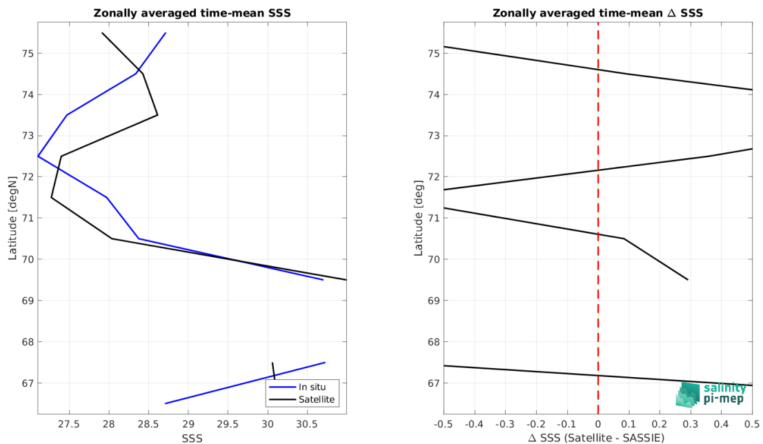
Figure 9: Left panel: Zonal mean SSS from CCI SSS L4 Merged-OI v5.5 - 30-day running (ESA) satellite product (black) and from SASSIE (blue). Right panel: Zonal mean of \Delta SSS (Satellite - SASSIE) for all the collected Pi-MEP match-up pairs estimated over the full satellite product period.
