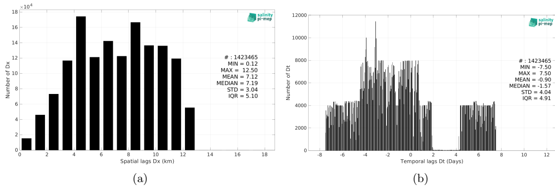
Figure 6: Histograms of the spatial (a) and temporal (b) lags between the location/time of the SASSIE measurement and the date of the corresponding CCI SSS L4 Merged-OI v5.5 - 30-day running (ESA) SSS pixel.
