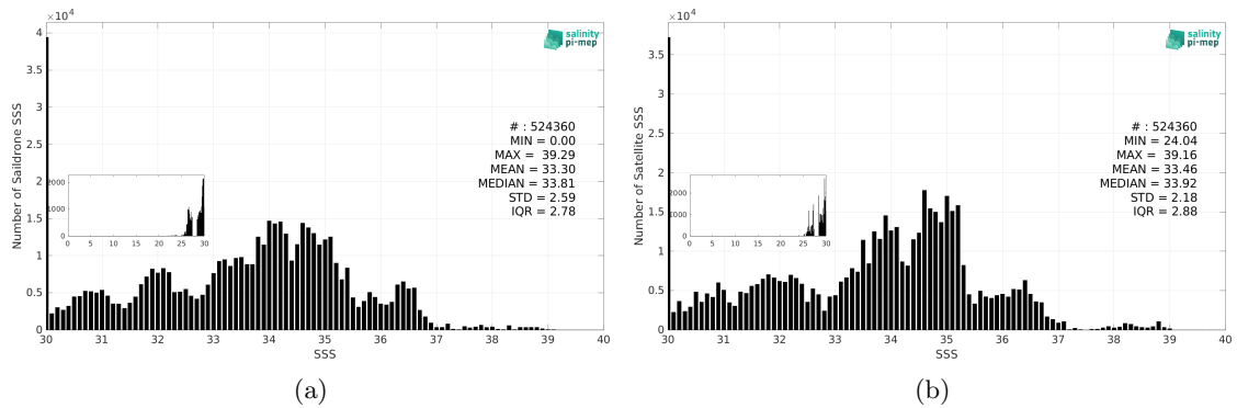
Figure 3: Histograms of SSS from Saildrone (a) and CCI SSS L4 Merged-OI v5.5 - 30-day running (ESA) (b) considering all match-up pairs per bins of 0.1 over the Global Ocean Pi-MEP region and for the full satellite product period.
