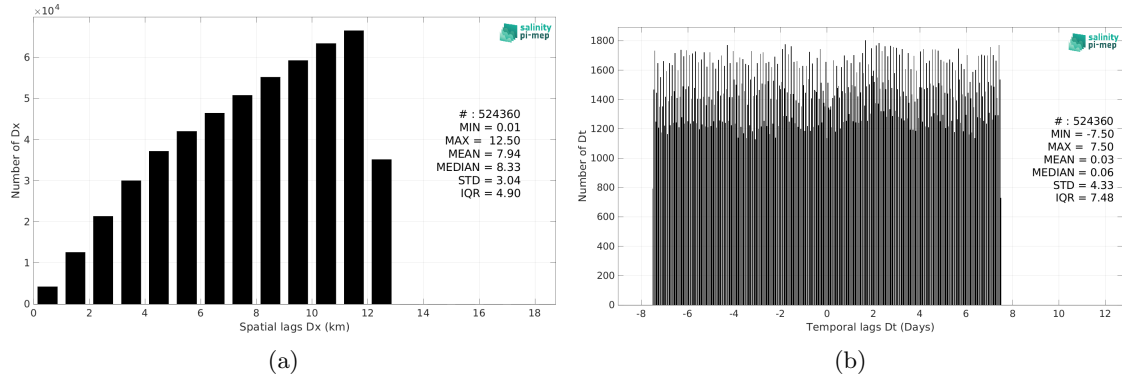
Figure 6: Histograms of the spatial (a) and temporal (b) lags between the location/time of the Sairdrone measurement and the date of the corresponding CCI SSS L4 Merged-OI v5.5 - 30-day running (ESA) SSS pixel.
