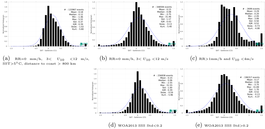
Figure 15: Normalized histogram of \Delta SSS (CCI SSS L4 Merged-OI v5.5 - 30-day running (ESA) - Saildrone) for 5 different subdatasets corresponding to: RR=0 mm/h, 3 < U_{10} < 12 m/s, SST>5°C, distance to coast > 800 km (a), RR=0 mm/h, 3 < U_{10} < 12 m/s (b), RR>1mm/h and U_{10} < 4 m/s (c), WOA2013 SSS Std<0.2 (d), WOA2013 SSS Std>0.2 (e).
