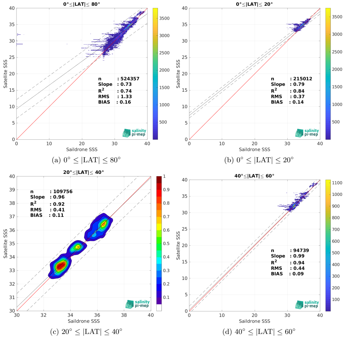
Figure 10: Contour maps of the concentration of CCI SSS L4 Merged-OI v5.5 - 30-day running (ESA) SSS (y-axis) versus Saildrone SSS (x-axis) at match-up pairs for different latitude bands. For each plot, the red line shows x=y . The black thin and dashed lines indicate a linear fit through the data cloud and the \pm 95\% confidence levels, respectively. The number match-up pairs n , the slope and R^2 coefficient of the linear fit, the root mean square (RMS) and the mean bias between satellite and in situ data are indicated for each latitude band in each plots.
