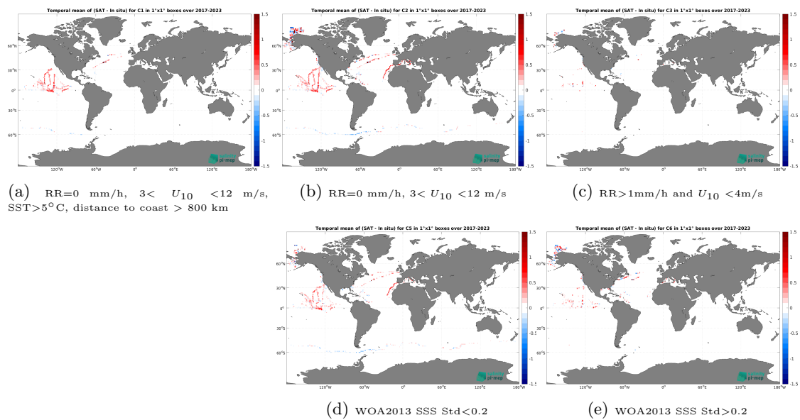
Figure 14: Temporal mean gridded over spatial boxes of size 1^\circ \times 1^\circ of \Delta\text{SSS} (CCI SSS L4 Merged-OI v5.5 - 30-day running (ESA) - Saildrone) for 5 different subdatasets corresponding to:RR=0 mm/h, 3 < U_{10} < 12 m/s, SST > 5^\circ\text{C} , distance to coast > 800 km (a), RR=0 mm/h, 3 < U_{10} < 12 m/s (b), RR > 1 mm/h and U_{10} < 4 m/s (c), WOA2013 SSS Std < 0.2 (d), WOA2013 SSS Std > 0.2 (e).
