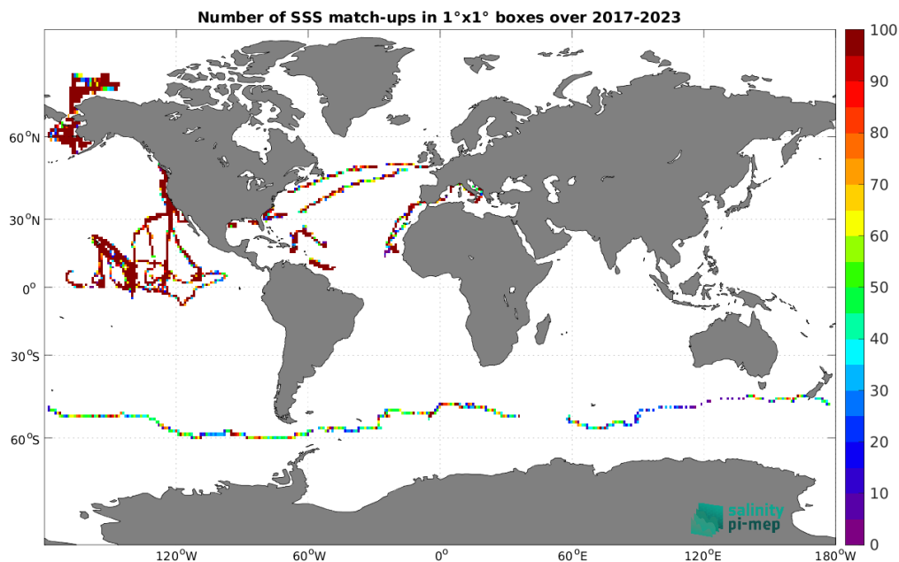
Figure 5: Number of SSS match-ups between Saildrone SSS and the CCI SSS L4 Merged-OI v5.5 - 30-day running (ESA) SSS product for the Global Ocean Pi-MEP region over 1^\circ \times 1^\circ boxes and for the full satellite product period.
