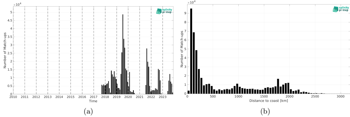
Figure 2: Number of match-ups between Saildrone and CCI SSS L4 Merged-OI v5.5 - 30-day running (ESA) SSS as a function of time (a) and as function of the distance to coast (b) over the Global Ocean Pi-MEP region and for the full satellite product period.
