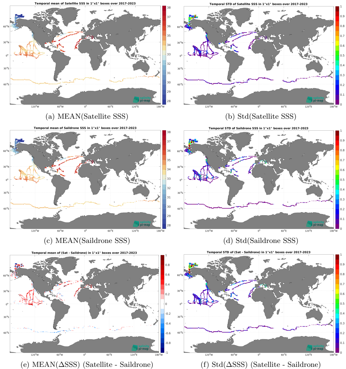
Figure 7: Temporal mean (left) and Std (right) of SSS from CCI SSS L4 Merged-OI v5.5 - 30-day running (ESA) (top), Saildrone (middle), and of \Delta SSS (Satellite - Saildrone ). Only match-up pairs are used to generate these maps.
