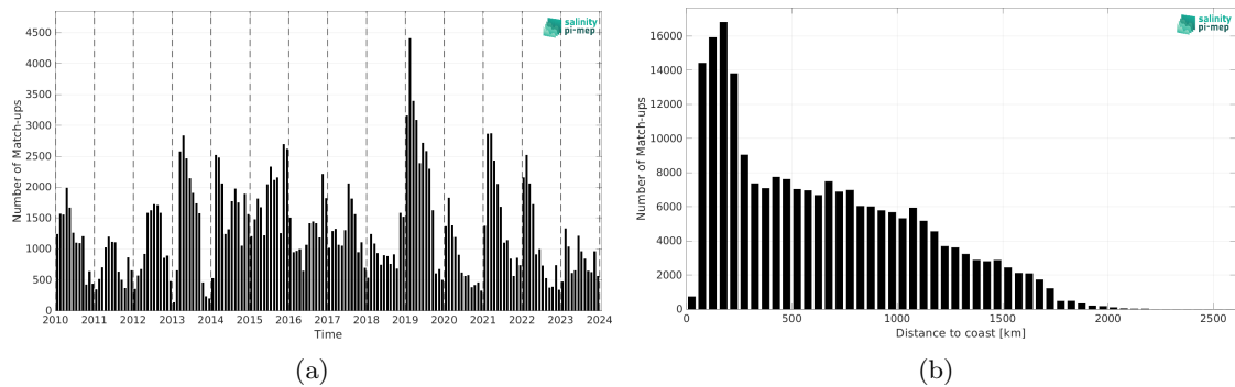
Figure 2: Number of match-ups between Marine mammals and CCI SSS L4 Merged-OI v5.5 - 30-day running (ESA) SSS as a function of time (a) and as function of the distance to coast (b) over the Global Ocean Pi-MEP region and for the full satellite product period.
