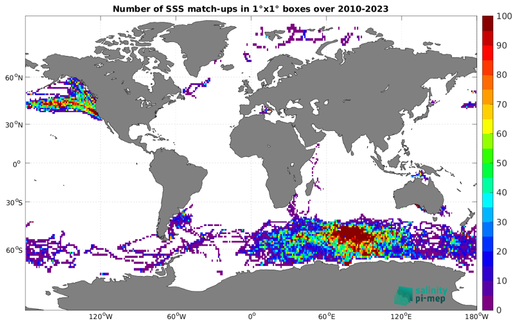
Figure 5: Number of SSS match-ups between Marine mammals SSS and the CCI SSS L4 Merged-OI v5.5 - 30-day running (ESA) SSS product for the Global Ocean Pi-MEP region over 1°×1° boxes and for the full satellite product period.
