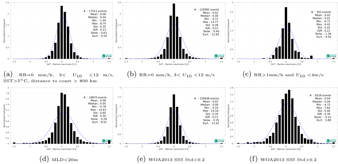
Figure 15: Normalized histogram of \Delta SSS (CCI SSS L4 Merged-OI v5.5 - 30-day running (ESA) - Marine mammals) for 6 different subdatasets corresponding to: RR=0 mm/h, 3 < U_{10} < 12 m/s, SST > 5°C, distance to coast > 800 km (a), RR=0 mm/h, 3 < U_{10} < 12 m/s (b), RR > 1mm/h and U_{10} < 4 m/s (c), MLD < 20m (d), WOA2013 SSS Std < 0.2 (e), WOA2013 SSS Std > 0.2 (f).
