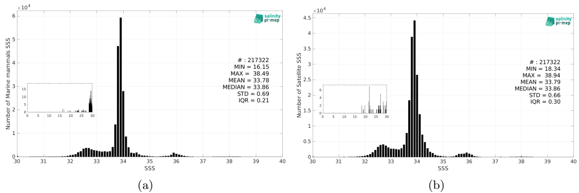
Figure 3: Histograms of SSS from Marine mammals (a) and CCI SSS L4 Merged-OI v5.5 - 30-day running (ESA) (b) considering all match-up pairs per bins of 0.1 over the Global Ocean Pi-MEP region and for the full satellite product period.
