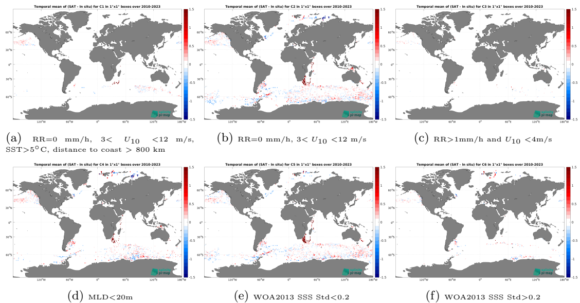
Figure 14: Temporal mean gridded over spatial boxes of size 1^\circ \times 1^\circ of \Delta SSS (CCI SSS L4 Merged-OI v5.5 - 30-day running (ESA) - Marine mammals) for 6 different subdatasets corresponding to:RR=0 mm/h, 3 < U_{10} < 12 m/s, SST >5^\circ C, distance to coast > 800 km (a), RR=0 mm/h, 3 < U_{10} < 12 m/s (b), RR >1 mm/h and U_{10} < 4 m/s (c),MLD <20 m (d),WOA2013 SSS Std <0.2 (e),WOA2013 SSS Std >0.2 (f).
