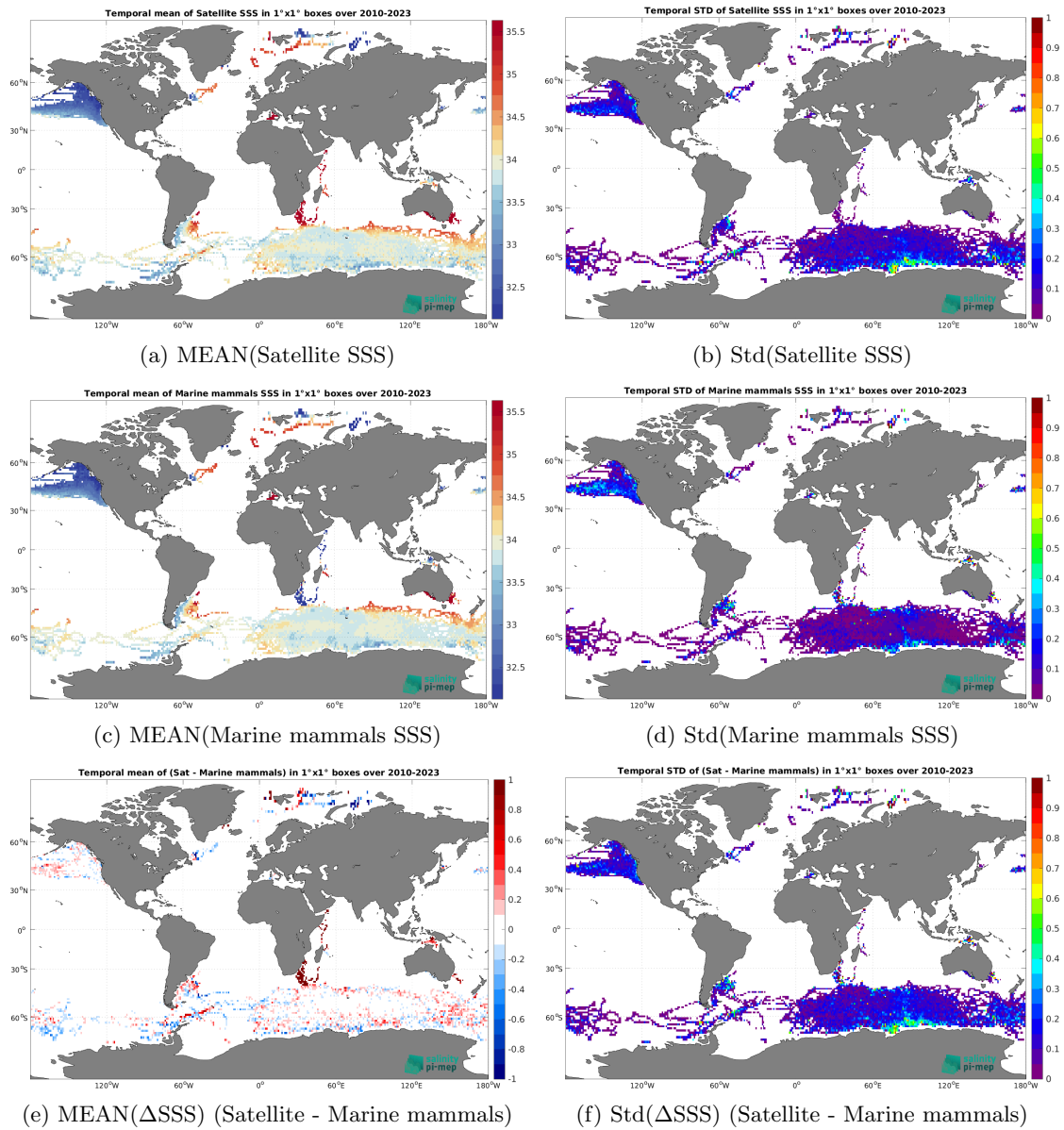
Figure 7: Temporal mean (left) and Std (right) of SSS from CCI SSS L4 Merged-OI v5.5 - 30-day running (ESA) (top), Marine mammals (middle), and of \Delta SSS (Satellite - Marine mammals). Only match-up pairs are used to generate these maps.
