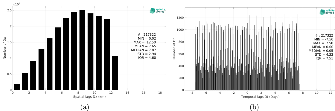
Figure 6: Histograms of the spatial (a) and temporal (b) lags between the location/time of the Marine mammals measurement and the date of the corresponding CCI SSS L4 Merged-OI v5.5 - 30-day running (ESA) SSS pixel.
