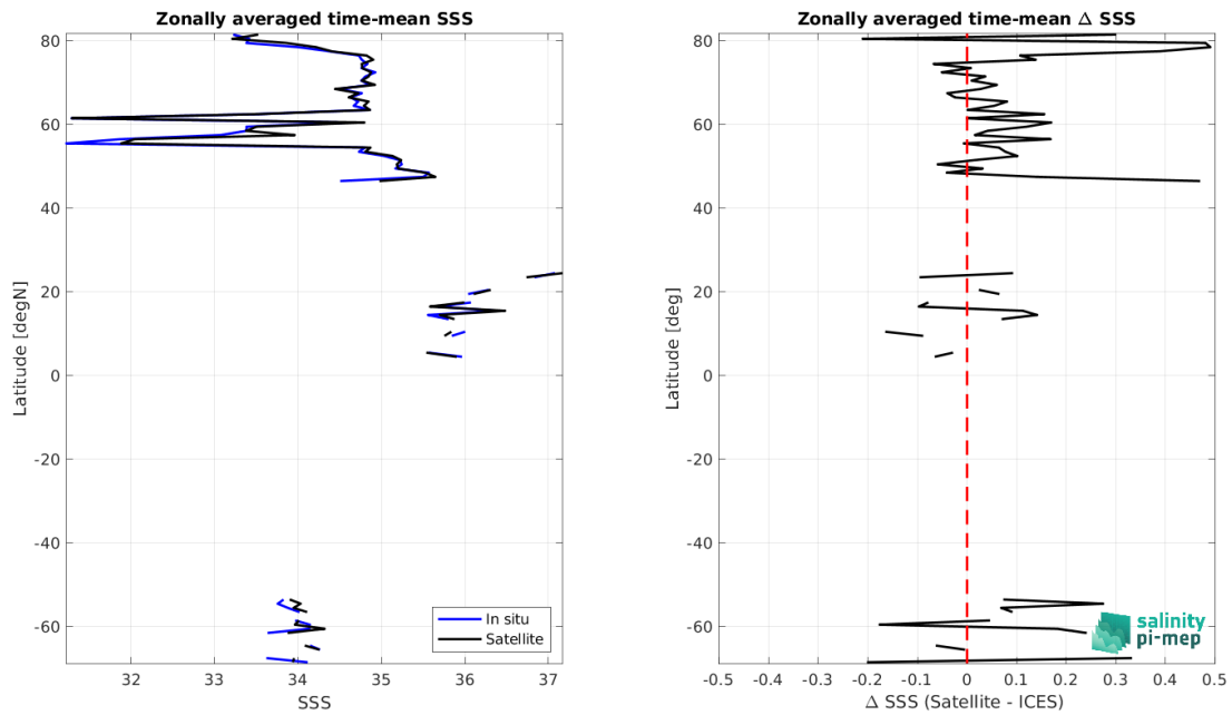
Figure 9: Left panel: Zonal mean SSS from CCI SSS L4 Merged-OI v5.5 - 30-day running (ESA) satellite product (black) and from ICES (blue). Right panel: Zonal mean of \Delta SSS (Satellite - ICES) for all the collected Pi-MEP match-up pairs estimated over the full satellite product period.
