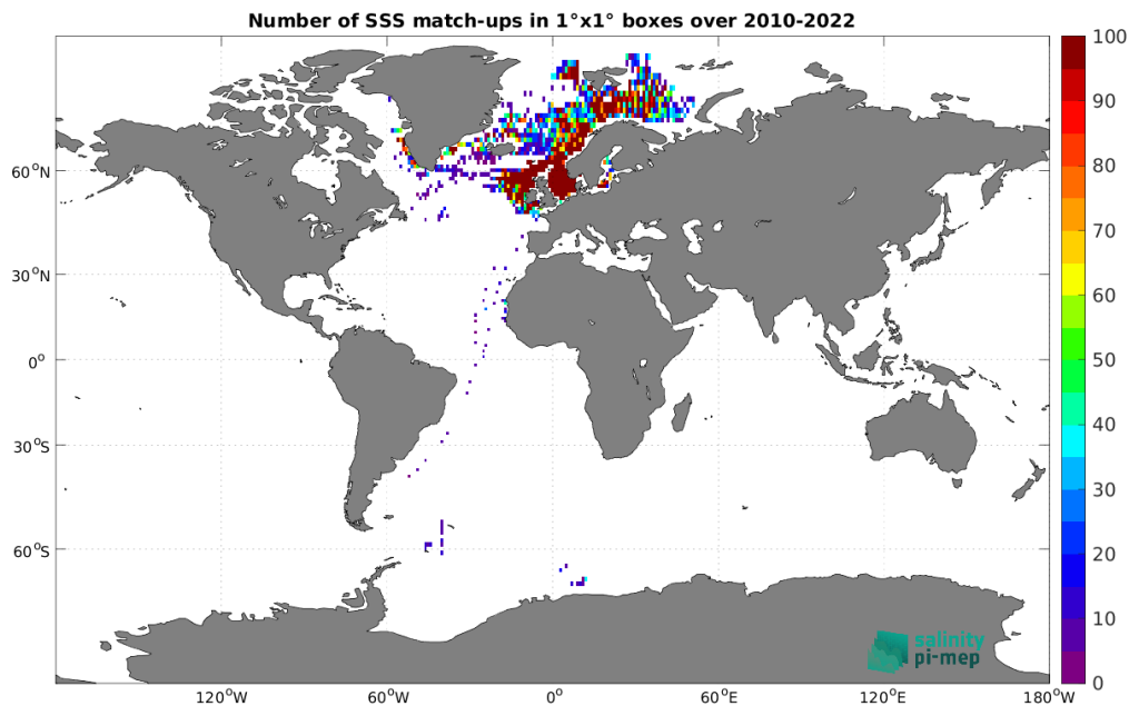
Figure 5: Number of SSS match-ups between ICES SSS and the CCI SSS L4 Merged-OI v5.5 - 30-day running (ESA) SSS product for the Global Ocean Pi-MEP region over 1^\circ \times 1^\circ boxes and for the full satellite product period.
