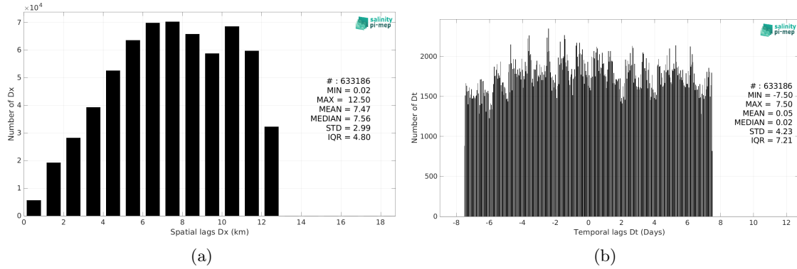
Figure 6: Histograms of the spatial (a) and temporal (b) lags between the location/time of the ICES measurement and the date of the corresponding CCI SSS L4 Merged-OI v5.5 - 30-day running (ESA) SSS pixel.
