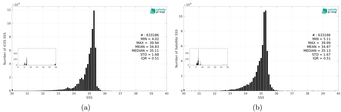
Figure 3: Histograms of SSS from ICES (a) and CCI SSS L4 Merged-OI v5.5 - 30-day running (ESA) (b) considering all match-up pairs per bins of 0.1 over the Global Ocean Pi-MEP region and for the full satellite product period.
