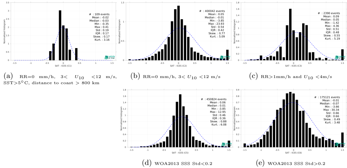
Figure 15: Normalized histogram of \Delta SSS (CCI SSS L4 Merged-OI v5.5 - 30-day running (ESA) - ICES) for 5 different subdatasets corresponding to: RR=0 mm/h, 3 < U_{10} < 12 m/s, SST > 5°C, distance to coast > 800 km (a), RR=0 mm/h, 3 < U_{10} < 12 m/s (b), RR > 1mm/h and U_{10} < 4 m/s (c), WOA2013 SSS Std < 0.2 (d), WOA2013 SSS Std > 0.2 (e).
