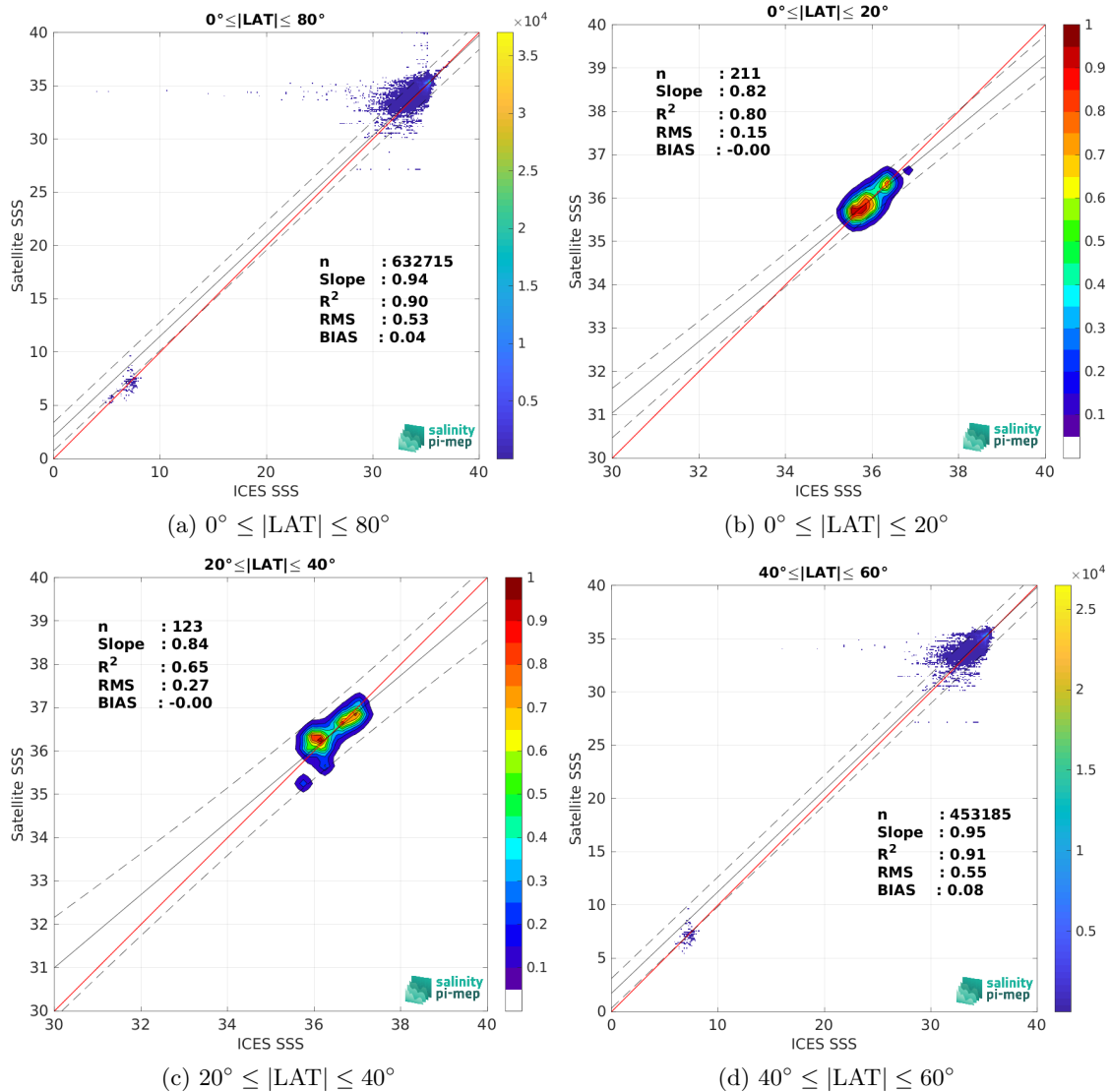
Figure 10: Contour maps of the concentration of CCI SSS L4 Merged-OI v5.5 - 30-day running (ESA) SSS (y-axis) versus ICES SSS (x-axis) at match-up pairs for different latitude bands. For each plot, the red line shows x=y . The black thin and dashed lines indicate a linear fit through the data cloud and the \pm 95\% confidence levels, respectively. The number match-up pairs n , the slope and R^2 coefficient of the linear fit, the root mean square (RMS) and the mean bias between satellite and in situ data are indicated for each latitude band in each plots.
