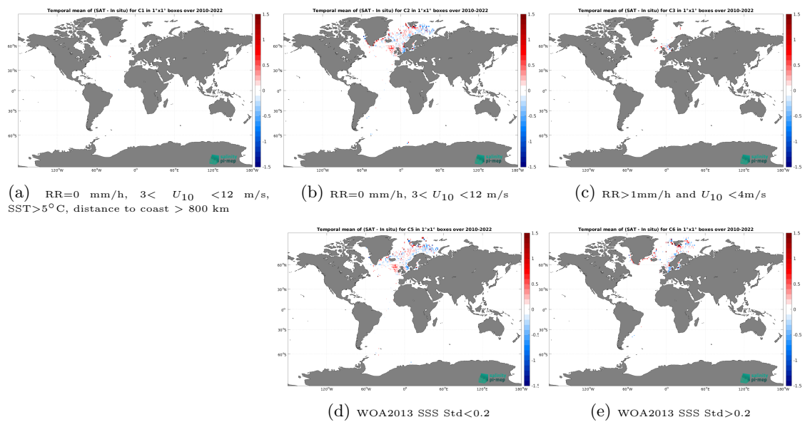
Figure 14: Temporal mean gridded over spatial boxes of size 1^\circ \times 1^\circ of \Delta SSS (CCI SSS L4 Merged-OI v5.5 - 30-day running (ESA) - ICES) for 5 different subdatasets corresponding to:RR=0 mm/h, 3 < U_{10} < 12 m/s, SST > 5^\circ\text{C} , distance to coast > 800 km (a), RR=0 mm/h, 3 < U_{10} < 12 m/s (b), RR > 1 mm/h and U_{10} < 4 m/s (c), WOA2013 SSS Std < 0.2 (d), WOA2013 SSS Std > 0.2 (e).
