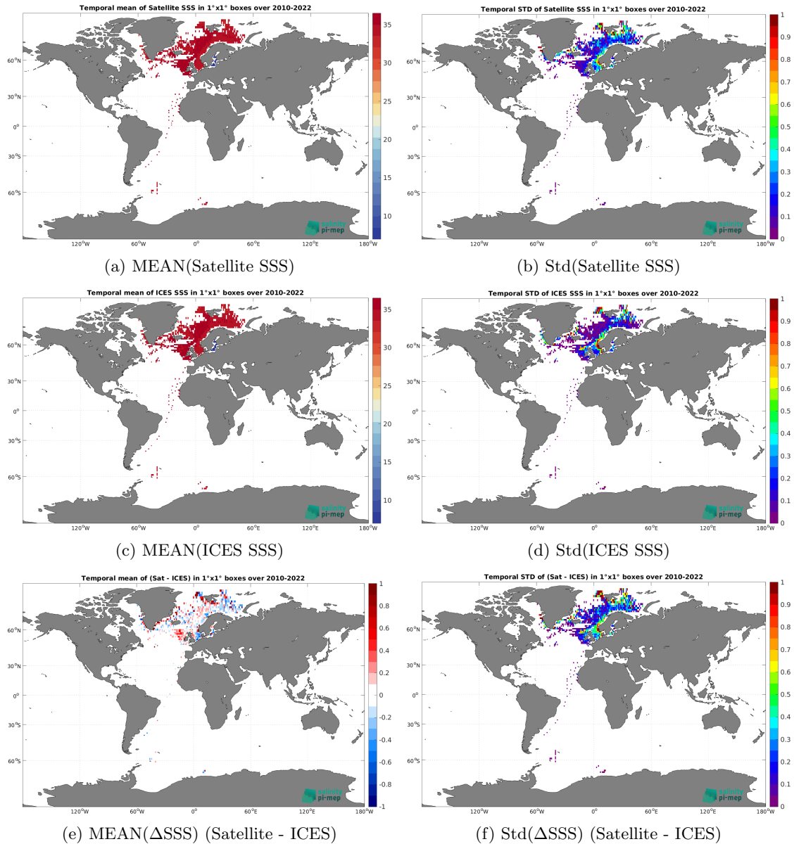
Figure 7: Temporal mean (left) and Std (right) of SSS from CCI SSS L4 Merged-OI v5.5 - 30-day running (ESA) (top), ICES (middle), and of \Delta SSS (Satellite - ICES). Only match-up pairs are used to generate these maps.
