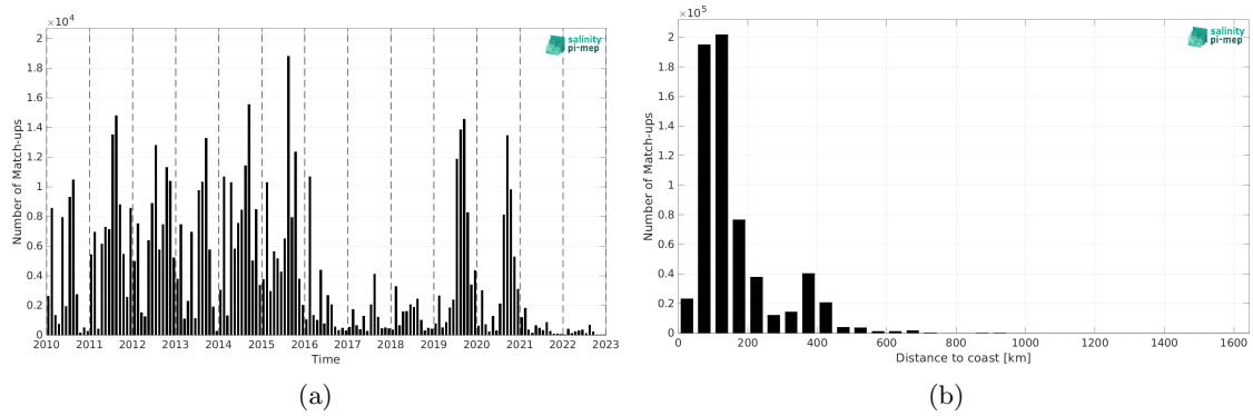
Figure 2: Number of match-ups between ICES and CCI SSS L4 Merged-OI v5.5 - 30-day running (ESA) SSS as a function of time (a) and as function of the distance to coast (b) over the Global Ocean Pi-MEP region and for the full satellite product period.
