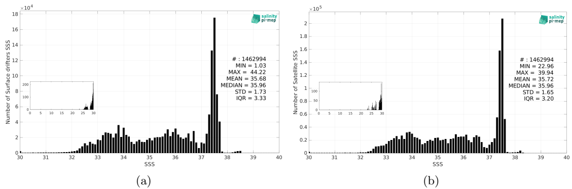
Figure 3: Histograms of SSS from Surface drifters (a) and CCI SSS L4 Merged-OI v5.5 - 30-day running (ESA) (b) considering all match-up pairs per bins of 0.1 over the Global Ocean Pi-MEP region and for the full satellite product period.
