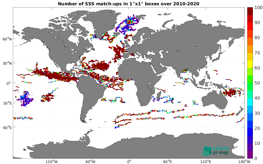
Figure 4: Number of SSS match-ups between Surface drifters SSS and the CCI SSS L4 Merged-OI v5.5 - 30-day running (ESA) SSS product for the Global Ocean Pi-MEP region over 1^\circ \times 1^\circ boxes and for the full satellite product period.
