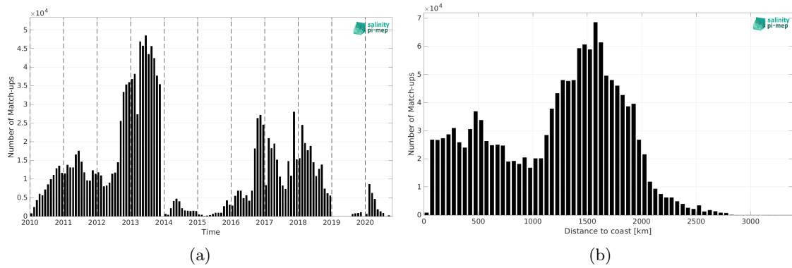
Figure 2: Number of match-ups between Surface drifters and CCI SSS L4 Merged-OI v5.5 - 30-day running (ESA) SSS as a function of time (a) and as function of the distance to coast (b) over the Global Ocean Pi-MEP region and for the full satellite product period.
