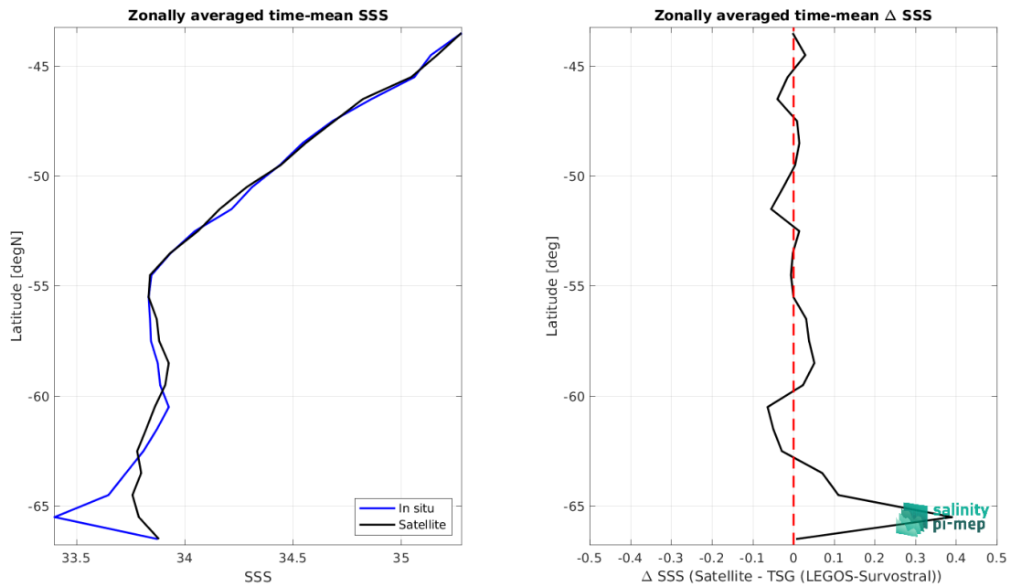
Figure 9: Left panel: Zonal mean SSS from CCI SSS L4 Merged-OI v4.41 - 7-day running (ESA) satellite product (black) and from TSG (LEGOS-Survostral) (blue). Right panel: Zonal mean of \Delta SSS (Satellite - TSG (LEGOS-Survostral)) for all the collected Pi-MEP match-up pairs estimated over the full satellite product period.
