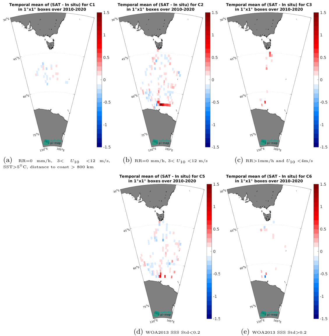
Figure 14: Temporal mean gridded over spatial boxes of size 1^\circ \times 1^\circ of \Delta\text{SSS} (CCI SSS L4 Merged-OI v4.41 - 7-day running (ESA) - TSG (LEGOS-Survostral)) for 5 different subdatasets corresponding to: RR=0 mm/h, 3 < U_{10} < 12 m/s, SST > 5^\circ\text{C} , distance to coast > 800 km (a), RR=0 mm/h, 3 < U_{10} < 12 m/s (b), RR > 1 mm/h and U_{10} < 4 m/s (c), WOA2013 SSS Std < 0.2 (d), WOA2013 SSS Std > 0.2 (e).
