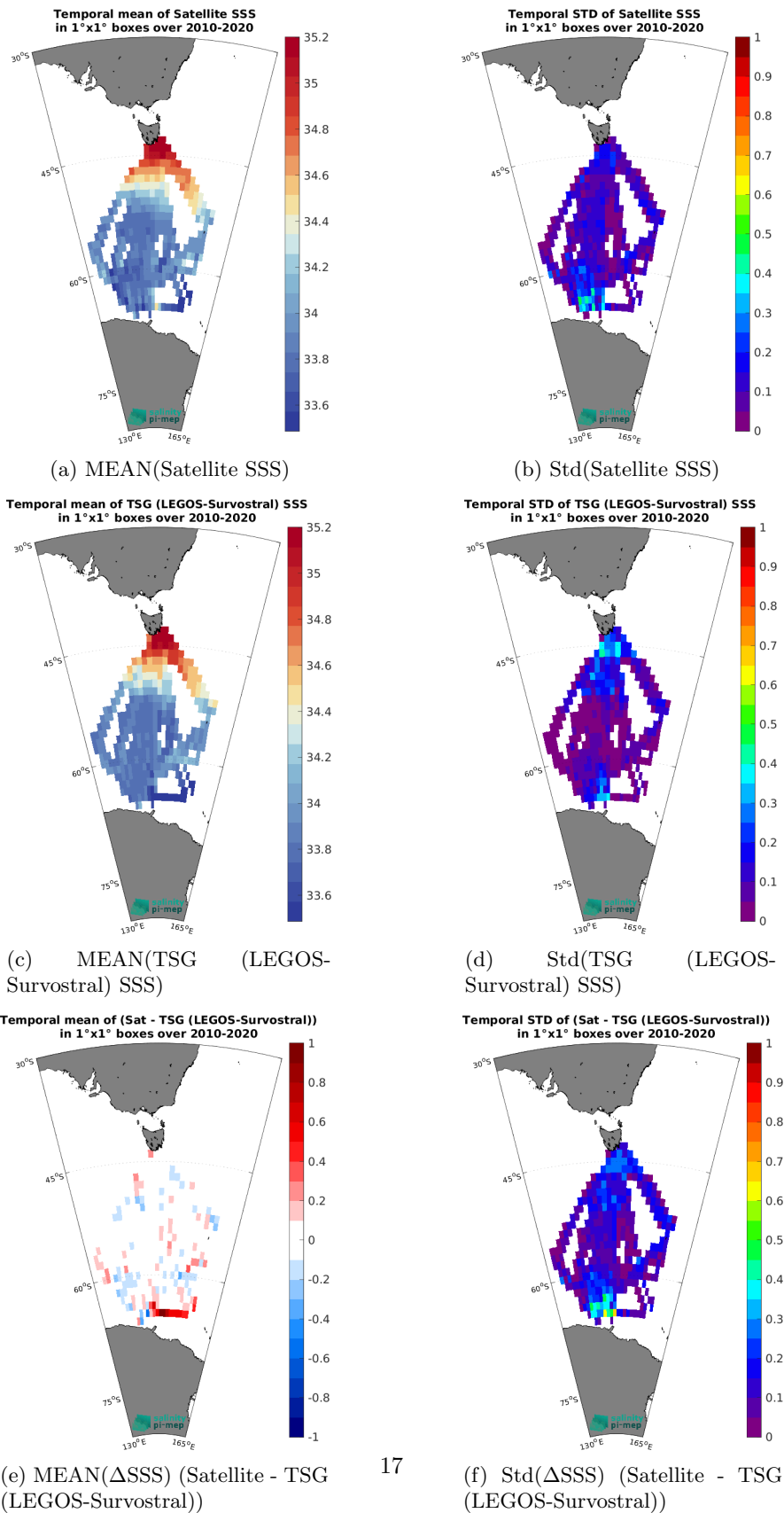
Figure 7: Temporal mean (left) and Std (right) of SSS from CCI SSS L4 Merged-OI v4.41 - 7-day running (ESA) (top), TSG (LEGOS-Survostral) (middle), and of \Delta SSS (Satellite - TSG (LEGOS-Survostral)). Only match-up pairs are used to generate these maps.
