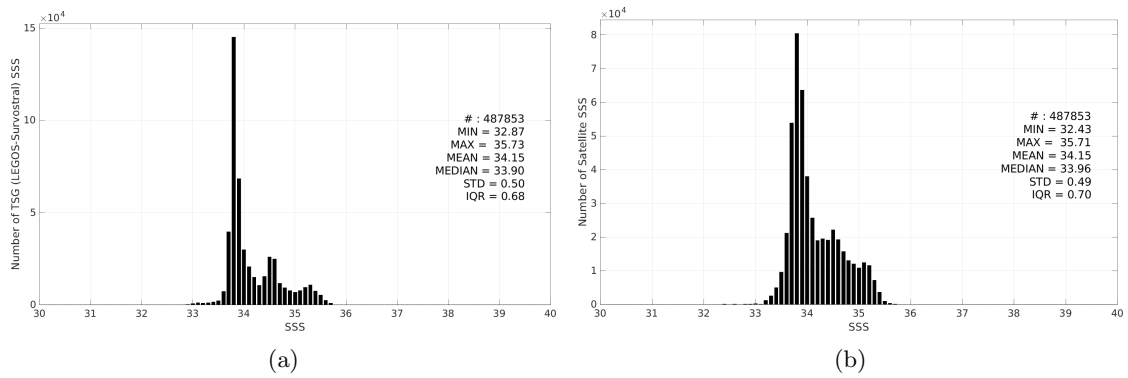
Figure 3: Histograms of SSS from TSG (LEGOS-Survostral) (a) and CCI SSS L4 Merged-OI v4.41 - 7-day running (ESA) (b) considering all match-up pairs per bins of 0.1 over the Global Ocean Pi-MEP region and for the full satellite product period.
