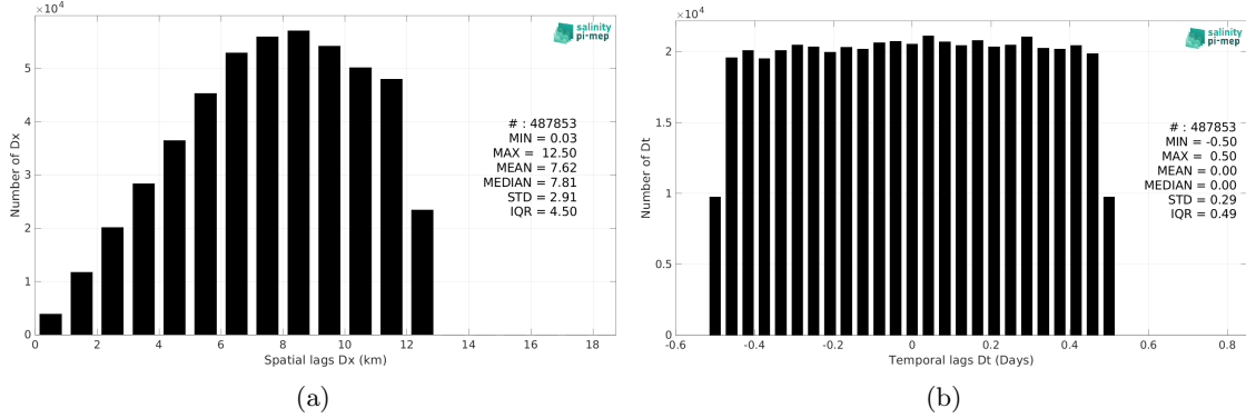
Figure 6: Histograms of the spatial (a) and temporal (b) lags between the location/time of the TSG (LEGOS-Survostral) measurement and the date of the corresponding CCI SSS L4 Merged-OI v4.41 - 7-day running (ESA) SSS pixel.
