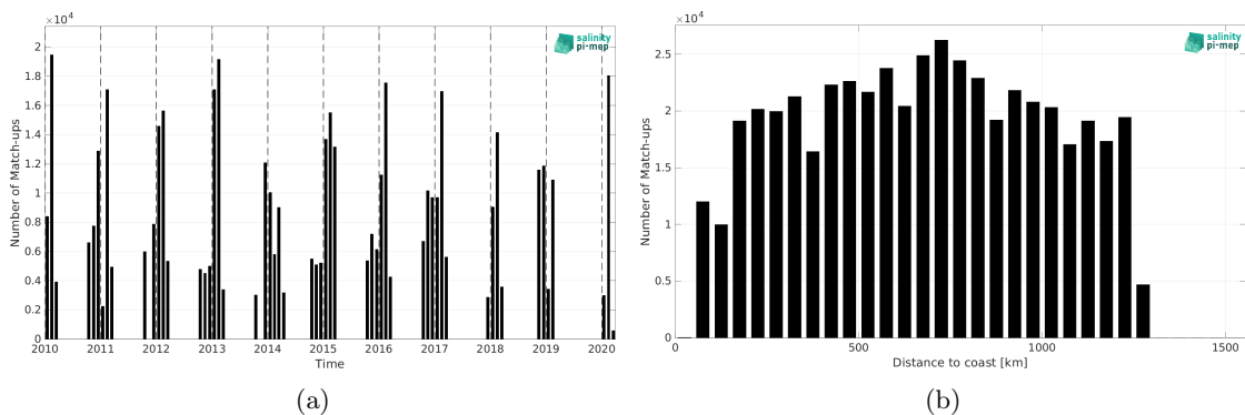
Figure 2: Number of match-ups between TSG (LEGOS-Survostral) and CCI SSS L4 Merged-OI v4.41 - 7-day running (ESA) SSS as a function of time (a) and as function of the distance to coast (b) over the Global Ocean Pi-MEP region and for the full satellite product period.
