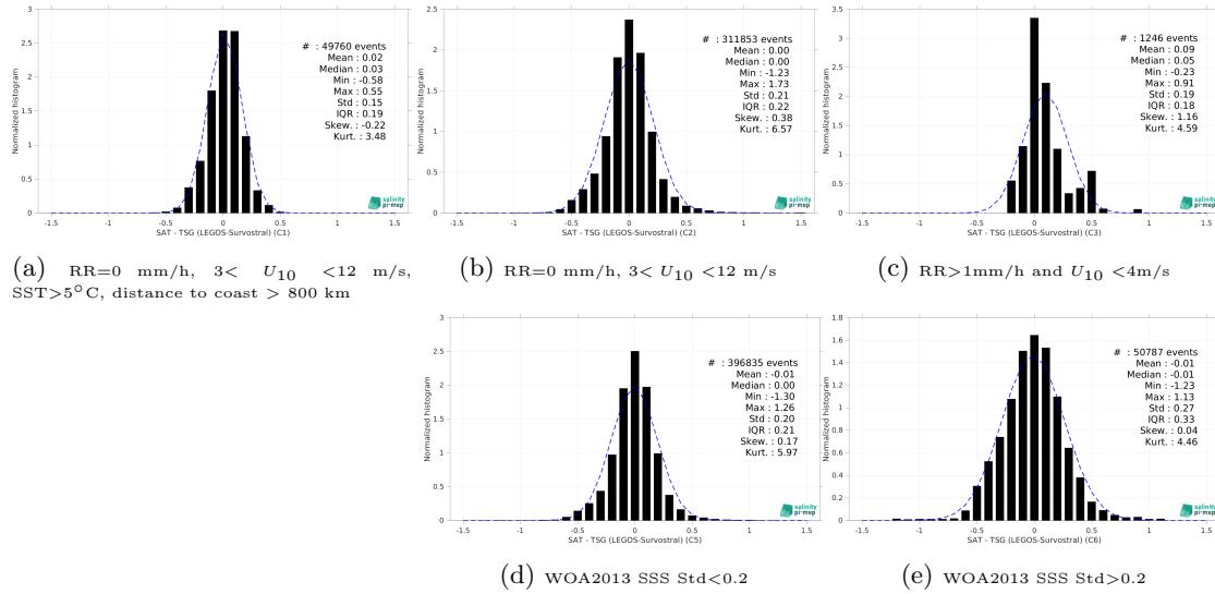
Figure 15: Normalized histogram of \Delta SSS (CCI SSS L4 Merged-OI v4.41 - 7-day running (ESA) - TSG (LEGOS-Survostral)) for 5 different subdatasets corresponding to: RR=0 mm/h, 3 < U_{10} < 12 m/s, SST>5°C, distance to coast > 800 km (a), RR=0 mm/h, 3 < U_{10} < 12 m/s (b), RR>1mm/h and U_{10} < 4 m/s (c), WOA2013 SSS Std<0.2 (d), WOA2013 SSS Std>0.2 (e).
