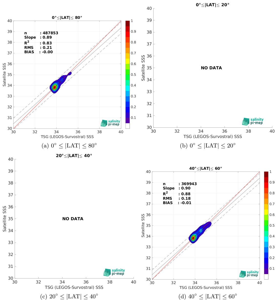
Figure 10: Contour maps of the concentration of CCI SSS L4 Merged-OI v4.41 - 7-day running (ESA) SSS (y-axis) versus TSG (LEGOS-Survostral) SSS (x-axis) at match-up pairs for different latitude bands. For each plot, the red line shows x=y . The black thin and dashed lines indicate a linear fit through the data cloud and the \pm 95\% confidence levels, respectively. The number match-up pairs n , the slope and R^2 coefficient of the linear fit, the root mean square (RMS) and the mean bias between satellite and in situ data are indicated for each latitude band in each plots.
