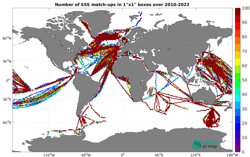
Figure 5: Number of SSS match-ups between TSG (LEGOS-DM) SSS and the CCI SSS L4 Merged-OI v4.41 - 7-day running (ESA) SSS product for the Global Ocean Pi-MEP region over 1^\circ \times 1^\circ boxes and for the full satellite product period.
