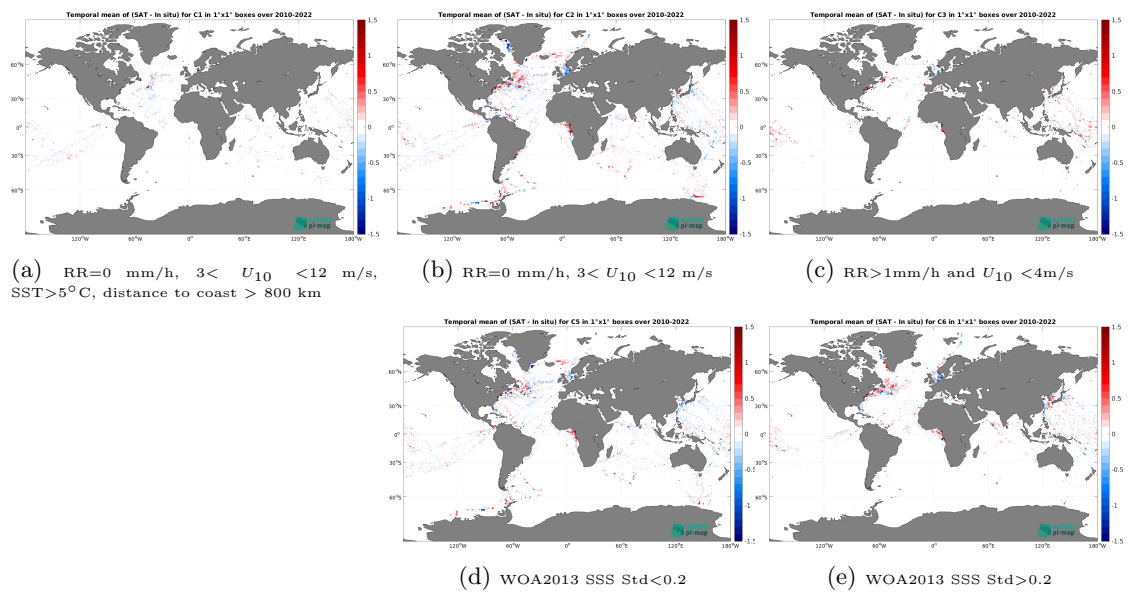
Figure 14: Temporal mean gridded over spatial boxes of size 1^\circ \times 1^\circ of \Delta SSS (CCI SSS L4 Merged-OI v4.41 - 7-day running (ESA) - TSG (LEGOS-DM)) for 5 different subdatasets corresponding to:RR=0 mm/h, 3 < U_{10} < 12 m/s, SST > 5^\circ\text{C} , distance to coast > 800 km (a), RR=0 mm/h, 3 < U_{10} < 12 m/s (b), RR > 1 mm/h and U_{10} < 4 m/s (c), WOA2013 SSS Std < 0.2 (d), WOA2013 SSS Std > 0.2 (e).
