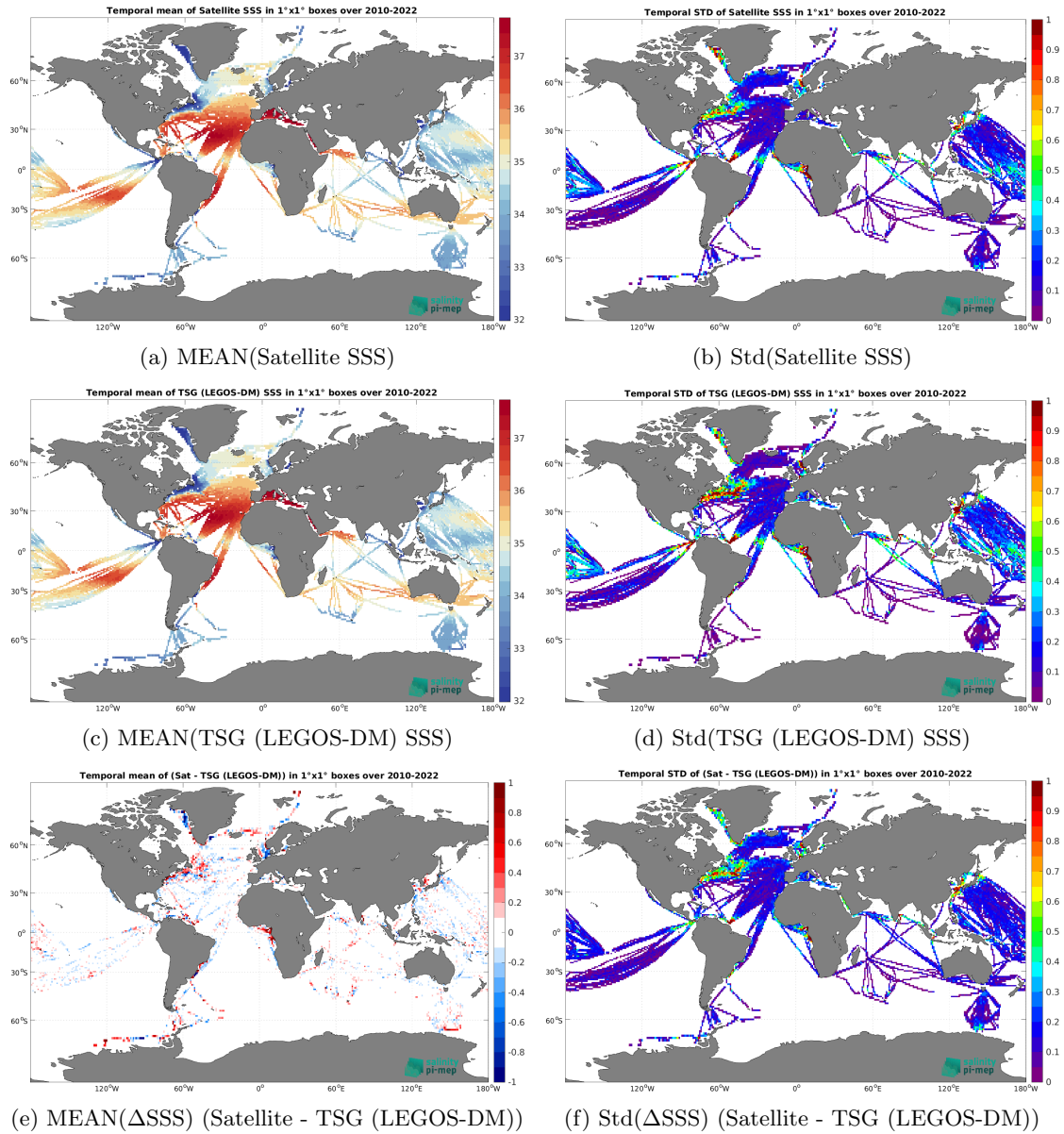
Figure 7: Temporal mean (left) and Std (right) of SSS from CCI SSS L4 Merged-OI v4.41 - 7-day running (ESA) (top), TSG (LEGOS-DM) (middle), and of \Delta SSS (Satellite - TSG (LEGOS-DM)). Only match-up pairs are used to generate these maps.
