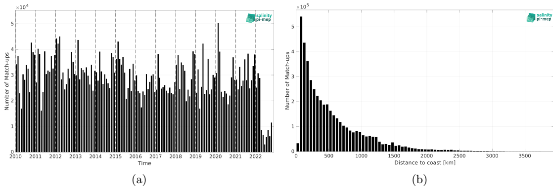
Figure 2: Number of match-ups between TSG (LEGOS-DM) and CCI SSS L4 Merged-OI v4.41 - 7-day running (ESA) SSS as a function of time (a) and as function of the distance to coast (b) over the Global Ocean Pi-MEP region and for the full satellite product period.
