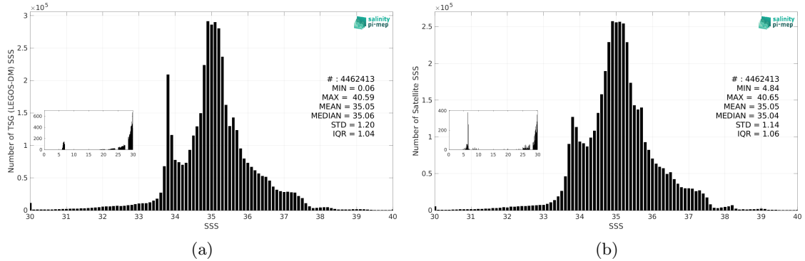
Figure 3: Histograms of SSS from TSG (LEGOS-DM) (a) and CCI SSS L4 Merged-OI v4.41 - 7-day running (ESA) (b) considering all match-up pairs per bins of 0.1 over the Global Ocean Pi-MEP region and for the full satellite product period.
