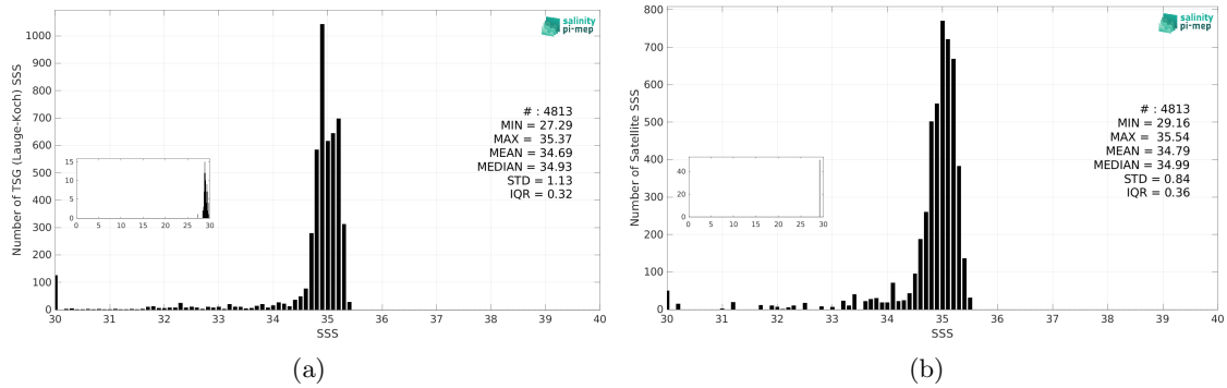
Figure 3: Histograms of SSS from TSG (Lauge-Koch) (a) and CCI SSS L4 Merged-OI v4.41 - 7-day running (ESA) (b) considering all match-up pairs per bins of 0.1 over the Global Ocean Pi-MEP region and for the full satellite product period.
