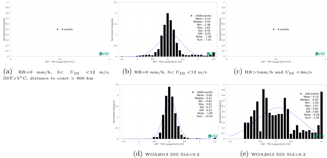
Figure 15: Normalized histogram of \Delta SSS (CCI SSS L4 Merged-OI v4.41 - 7-day running (ESA) - TSG (Lauge-Koch)) for 5 different subdatasets corresponding to: RR=0 mm/h, 3 < U_{10} < 12 m/s, SST>5°C, distance to coast > 800 km (a), RR=0 mm/h, 3 < U_{10} < 12 m/s (b), RR>1mm/h and U_{10} < 4 m/s (c), WOA2013 SSS Std<0.2 (d), WOA2013 SSS Std>0.2 (e).
