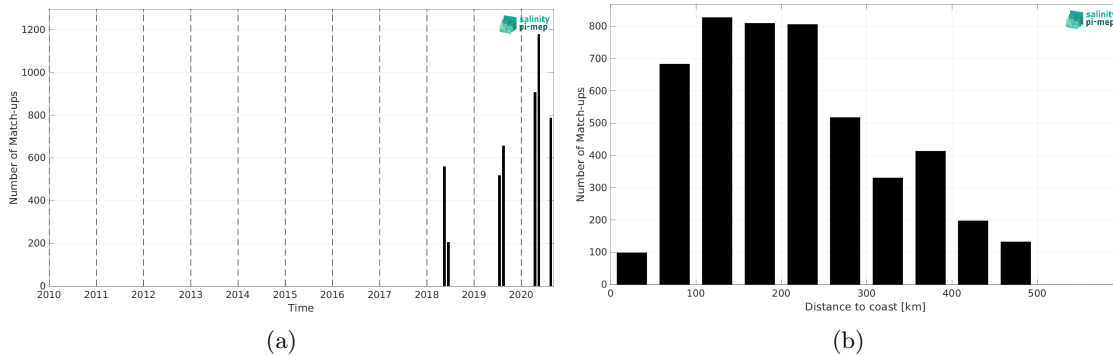
Figure 2: Number of match-ups between TSG (Lauge-Koch) and CCI SSS L4 Merged-OI v4.41 - 7-day running (ESA) SSS as a function of time (a) and as function of the distance to coast (b) over the Global Ocean Pi-MEP region and for the full satellite product period.
