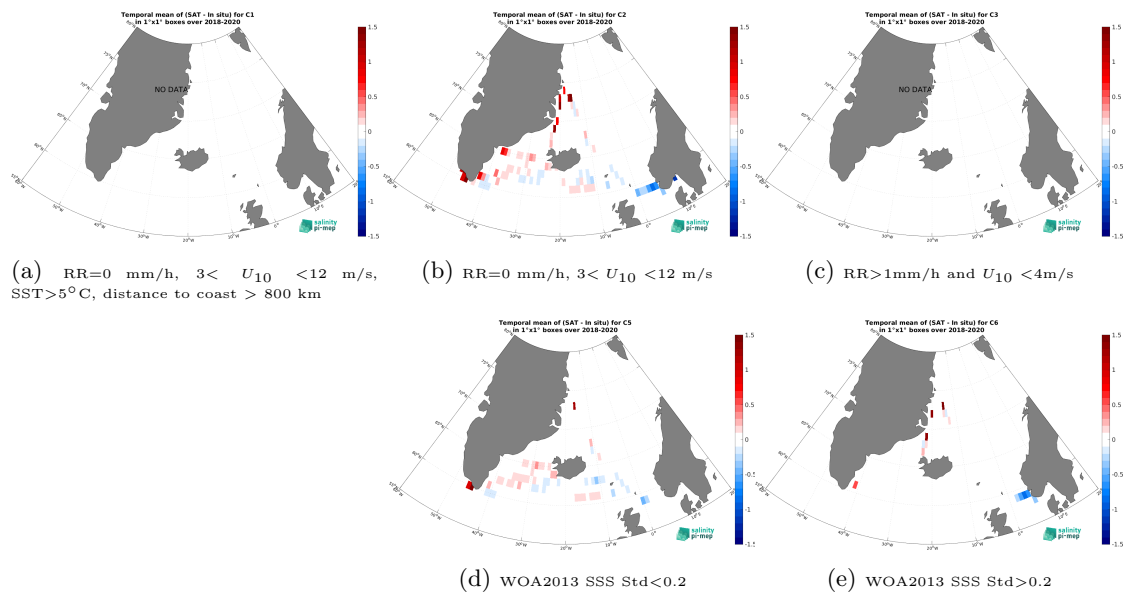
Figure 14: Temporal mean gridded over spatial boxes of size 1^\circ \times 1^\circ of \Delta SSS (CCI SSS L4 Merged-OI v4.41 - 7-day running (ESA) - TSG (Lauge-Koch)) for 5 different subdatasets corresponding to:RR=0 mm/h, 3 < U_{10} < 12 m/s, SST > 5^\circ\text{C} , distance to coast > 800 km (a), RR=0 mm/h, 3 < U_{10} < 12 m/s (b), RR > 1 mm/h and U_{10} < 4 m/s (c), WOA2013 SSS Std < 0.2 (d), WOA2013 SSS Std > 0.2 (e).
