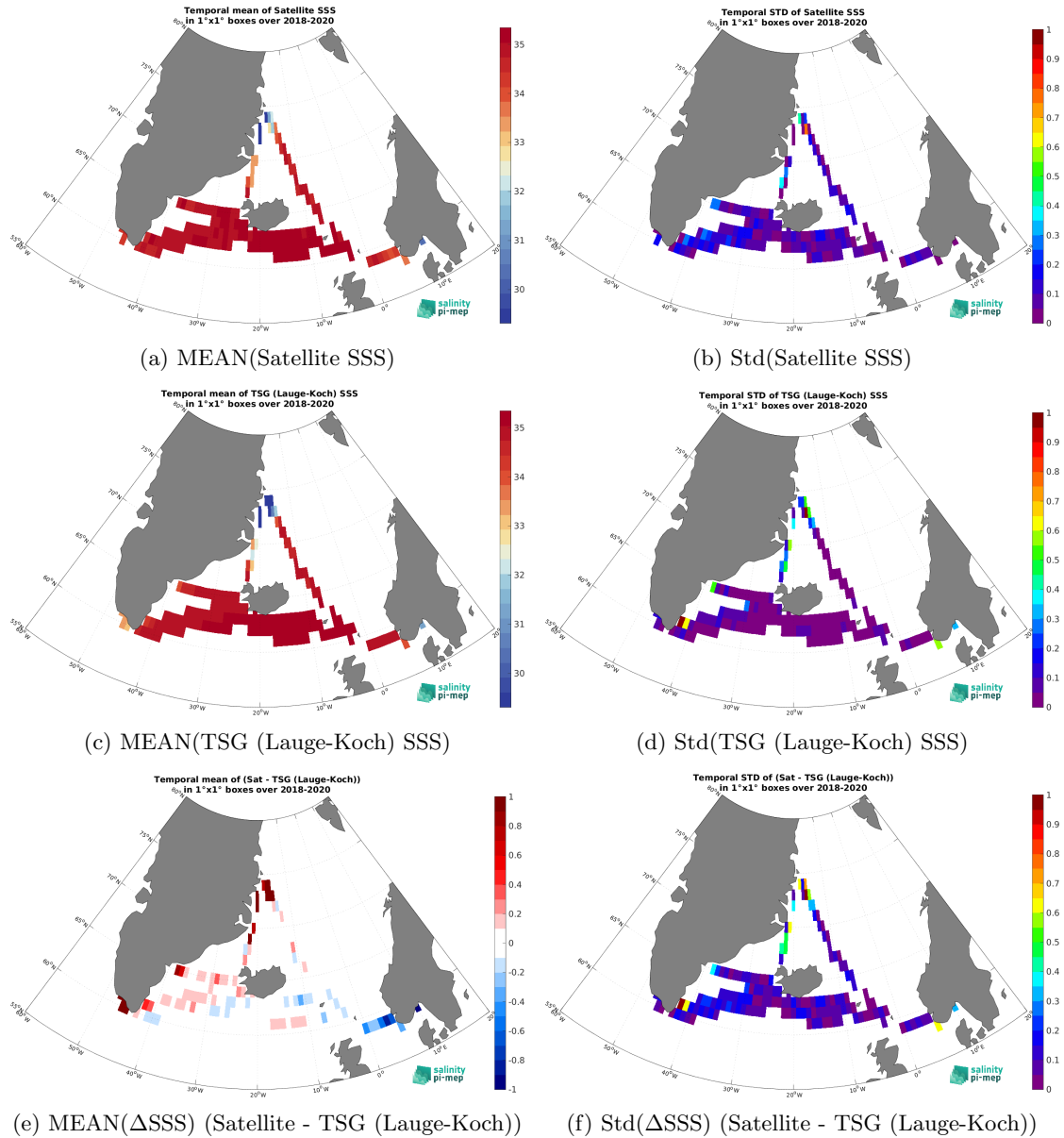
Figure 7: Temporal mean (left) and Std (right) of SSS from CCI SSS L4 Merged-OI v4.41 - 7-day running (ESA) (top), TSG (Lauge-Koch) (middle), and of \Delta SSS (Satellite - TSG (Lauge-Koch)). Only match-up pairs are used to generate these maps.
