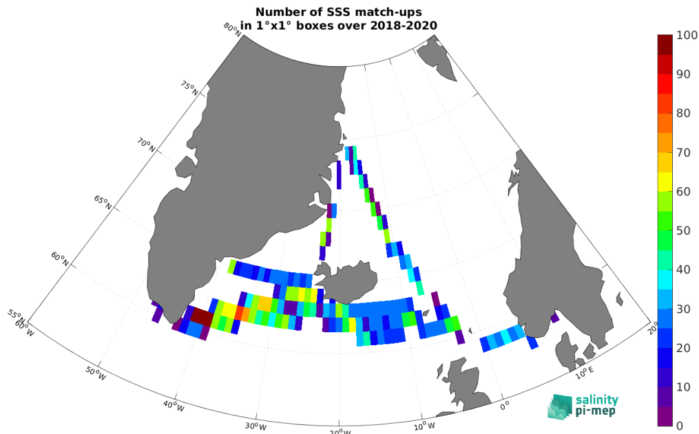
Figure 5: Number of SSS match-ups between TSG (Lauge-Koch) SSS and the CCI SSS L4 Merged-OI v4.41 - 7-day running (ESA) SSS product for the Global Ocean Pi-MEP region over 1^\circ \times 1^\circ boxes and for the full satellite product period.
