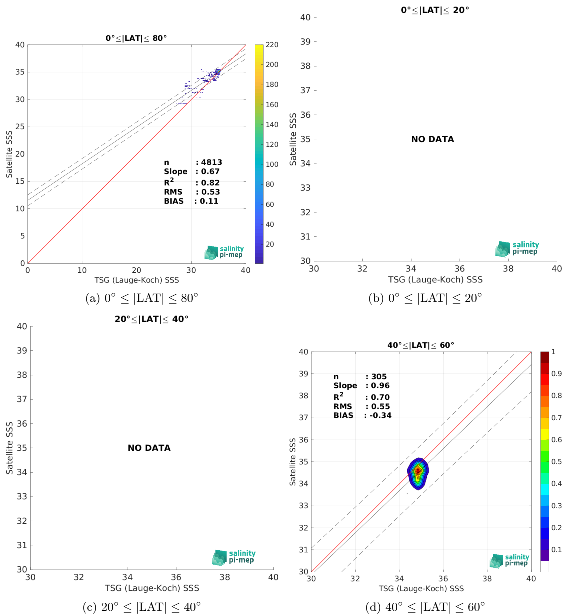
Figure 10: Contour maps of the concentration of CCI SSS L4 Merged-OI v4.41 - 7-day running (ESA) SSS (y-axis) versus TSG (Lauge-Koch) SSS (x-axis) at match-up pairs for different latitude bands. For each plot, the red line shows x=y . The black thin and dashed lines indicate a linear fit through the data cloud and the \pm 95\% confidence levels, respectively. The number match-up pairs n , the slope and R^2 coefficient of the linear fit, the root mean square (RMS) and the mean bias between satellite and in situ data are indicated for each latitude band in each plots.
