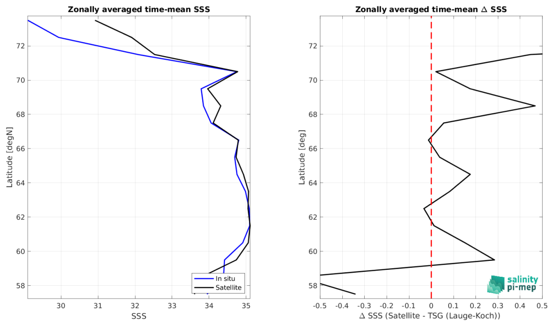
Figure 9: Left panel: Zonal mean SSS from CCI SSS L4 Merged-OI v4.41 - 7-day running (ESA) satellite product (black) and from TSG (Lauge-Koch) (blue). Right panel: Zonal mean of \Delta SSS (Satellite - TSG (Lauge-Koch)) for all the collected Pi-MEP match-up pairs estimated over the full satellite product period.
