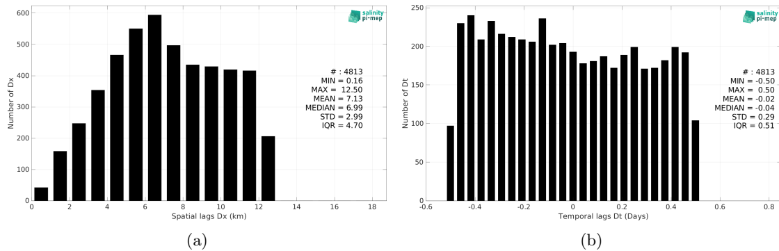
Figure 6: Histograms of the spatial (a) and temporal (b) lags between the location/time of the TSG (Lauge-Koch) measurement and the date of the corresponding CCI SSS L4 Merged-OI v4.41 - 7-day running (ESA) SSS pixel.
