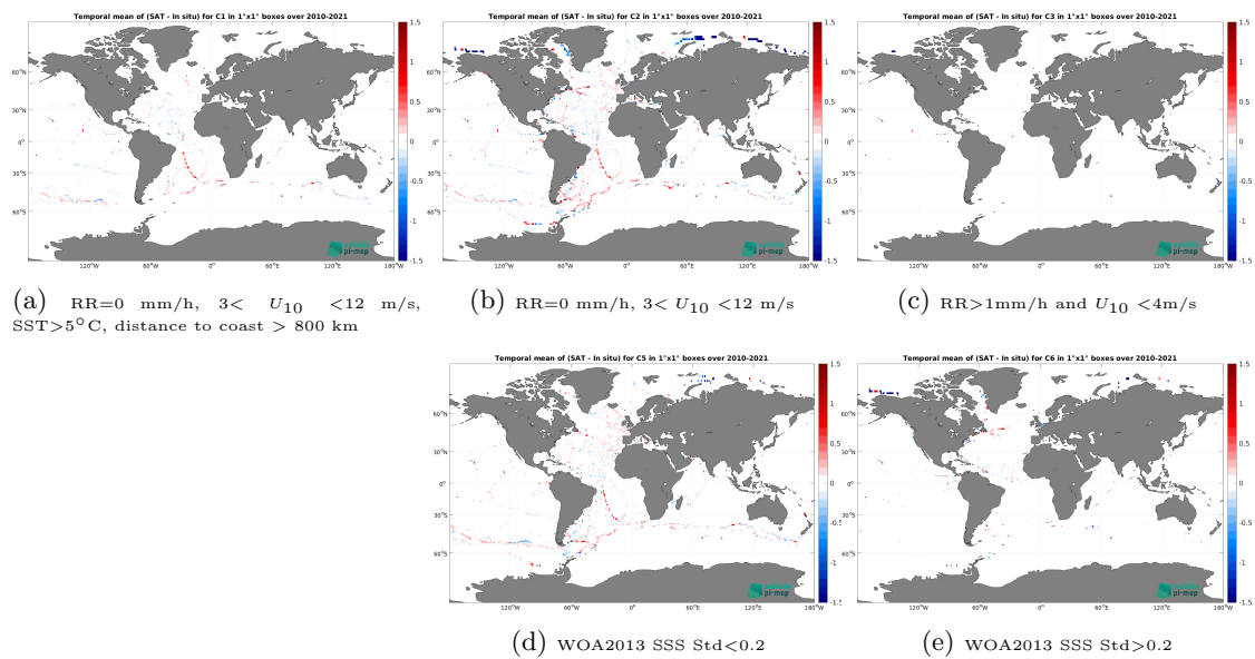
Figure 14: Temporal mean gridded over spatial boxes of size 1^\circ \times 1^\circ of \Delta SSS (CCI SSS L4 Merged-OI v4.41 - 7-day running (ESA) - TSG (GOSUD-Sailing-ship)) for 5 different subdatasets corresponding to: RR=0 mm/h, 3 < U_{10} < 12 m/s, SST > 5^\circ\text{C} , distance to coast > 800 km (a), RR=0 mm/h, 3 < U_{10} < 12 m/s (b), RR > 1 mm/h and U_{10} < 4 m/s (c), WOA2013 SSS Std < 0.2 (d), WOA2013 SSS Std > 0.2 (e).
