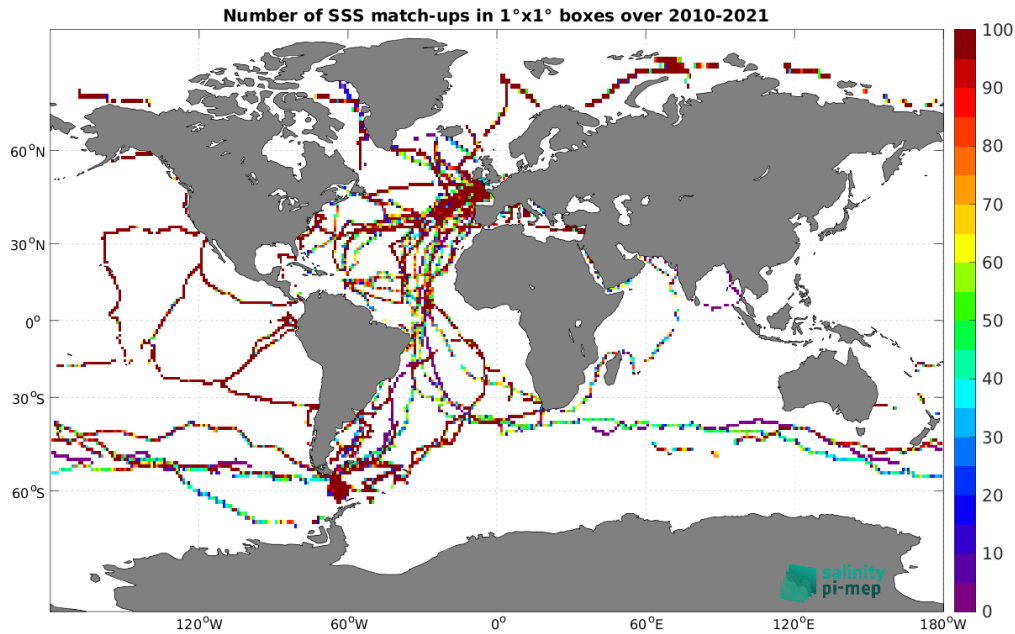
Figure 5: Number of SSS match-ups between TSG (GOSUD-Sailing-ship) SSS and the CCI SSS L4 Merged-OI v4.41 - 7-day running (ESA) SSS product for the Global Ocean Pi-MEP region over 1^\circ \times 1^\circ boxes and for the full satellite product period.
