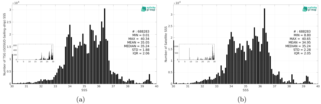
Figure 3: Histograms of SSS from TSG (GOSUD-Sailing-ship) (a) and CCI SSS L4 Merged-OI v4.41 - 7-day running (ESA) (b) considering all match-up pairs per bins of 0.1 over the Global Ocean Pi-MEP region and for the full satellite product period.
