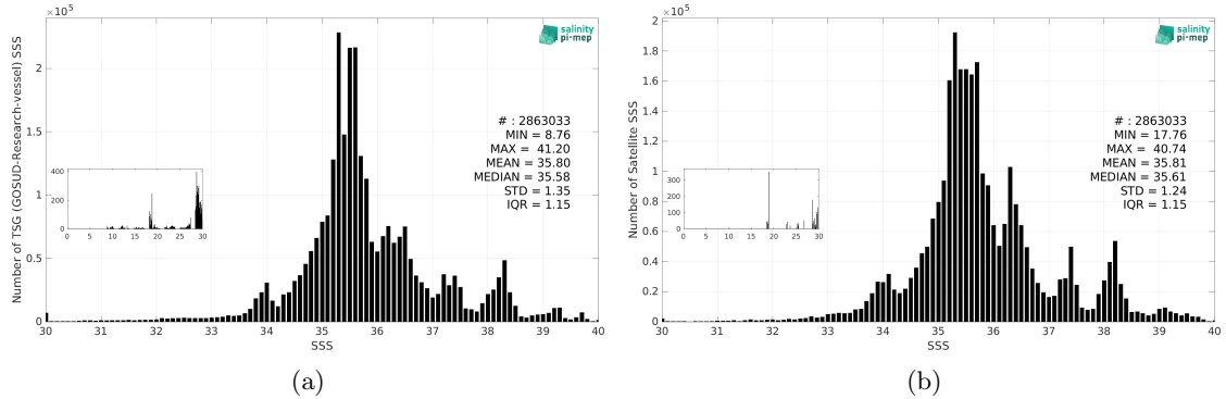
Figure 3: Histograms of SSS from TSG (GOSUD-Research-vessel) (a) and CCI SSS L4 Merged-OI v4.41 - 7-day running (ESA) (b) considering all match-up pairs per bins of 0.1 over the Global Ocean Pi-MEP region and for the full satellite product period.
