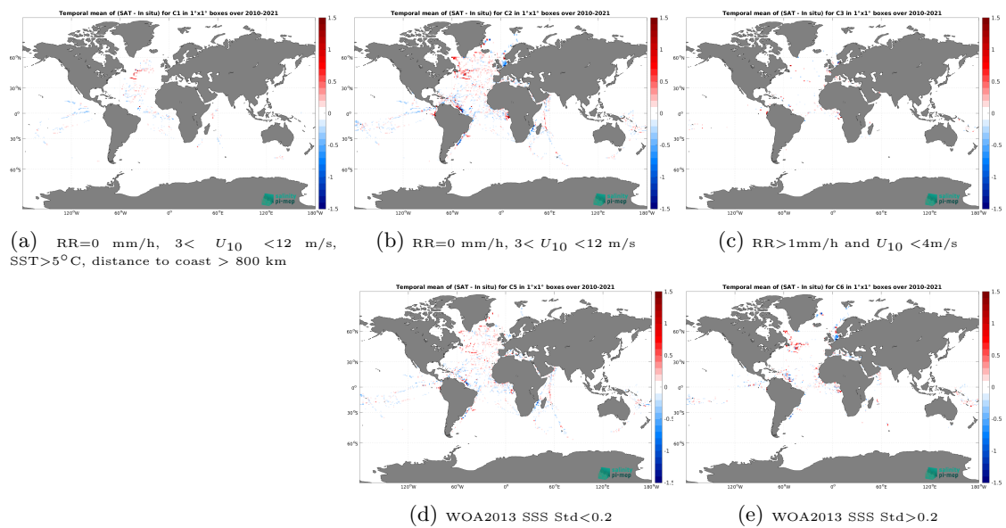
Figure 14: Temporal mean gridded over spatial boxes of size 1^\circ \times 1^\circ of \Delta\text{SSS} (CCI SSS L4 Merged-OI v4.41 - 7-day running (ESA) - TSG (GOSUD-Research-vessel)) for 5 different subdatasets corresponding to:RR=0 mm/h, 3 < U_{10} < 12 m/s, SST > 5^\circ\text{C} , distance to coast > 800 km (a), RR=0 mm/h, 3 < U_{10} < 12 m/s (b), RR > 1 mm/h and U_{10} < 4 m/s (c), WOA2013 SSS Std < 0.2 (d), WOA2013 SSS Std > 0.2 (e).
