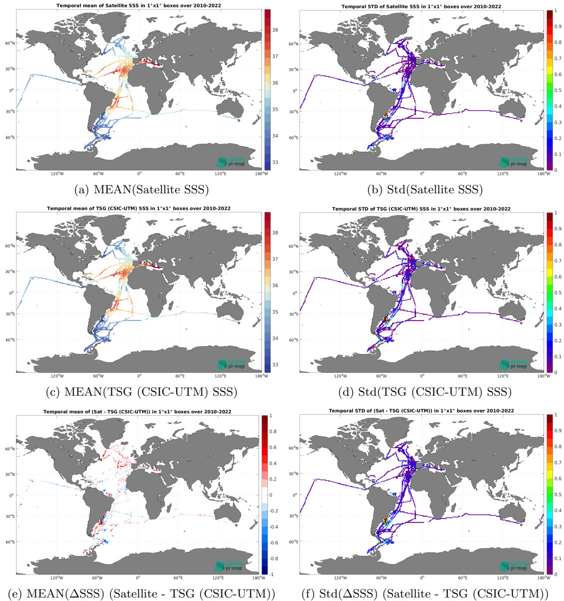
Figure 7: Temporal mean (left) and Std (right) of SSS from CCI SSS L4 Merged-OI v4.41 - 7-day running (ESA) (top), TSG (CSIC-UTM) (middle), and of \Delta SSS (Satellite - TSG (CSIC-UTM)). Only match-up pairs are used to generate these maps.
