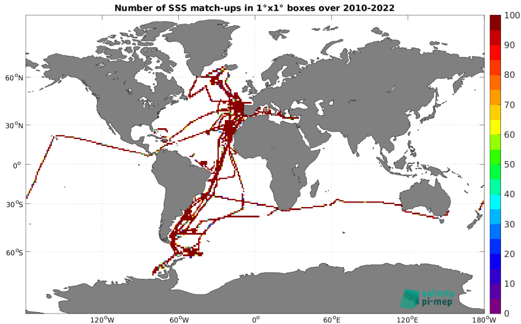
Figure 5: Number of SSS match-ups between TSG (CSIC-UTM) SSS and the CCI SSS L4 Merged-OI v4.41 - 7-day running (ESA) SSS product for the Global Ocean Pi-MEP region over 1^\circ \times 1^\circ boxes and for the full satellite product period.
