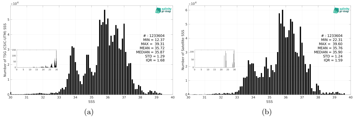
Figure 3: Histograms of SSS from TSG (CSIC-UTM) (a) and CCI SSS L4 Merged-OI v4.41 - 7-day running (ESA) (b) considering all match-up pairs per bins of 0.1 over the Global Ocean Pi-MEP region and for the full satellite product period.
