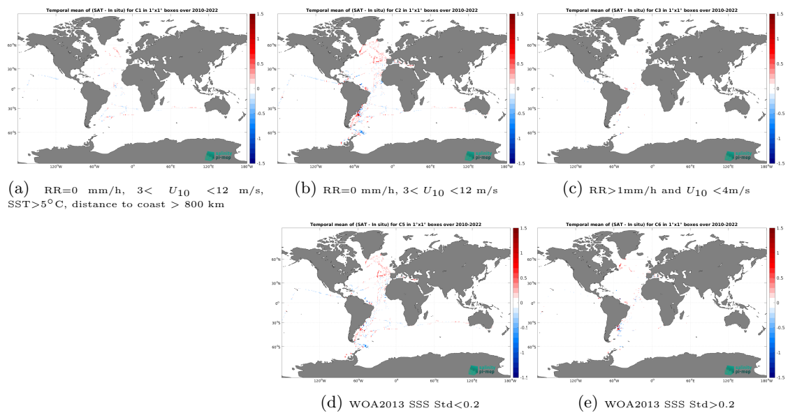
Figure 14: Temporal mean gridded over spatial boxes of size 1^\circ \times 1^\circ of \Delta SSS (CCI SSS L4 Merged-OI v4.41 - 7-day running (ESA) - TSG (CSIC-UTM)) for 5 different subdatasets corresponding to:RR=0 mm/h, 3 < U_{10} < 12 m/s, SST > 5^\circ\text{C} , distance to coast > 800 km (a), RR=0 mm/h, 3 < U_{10} < 12 m/s (b), RR > 1 mm/h and U_{10} < 4 m/s (c), WOA2013 SSS Std < 0.2 (d), WOA2013 SSS Std > 0.2 (e).
