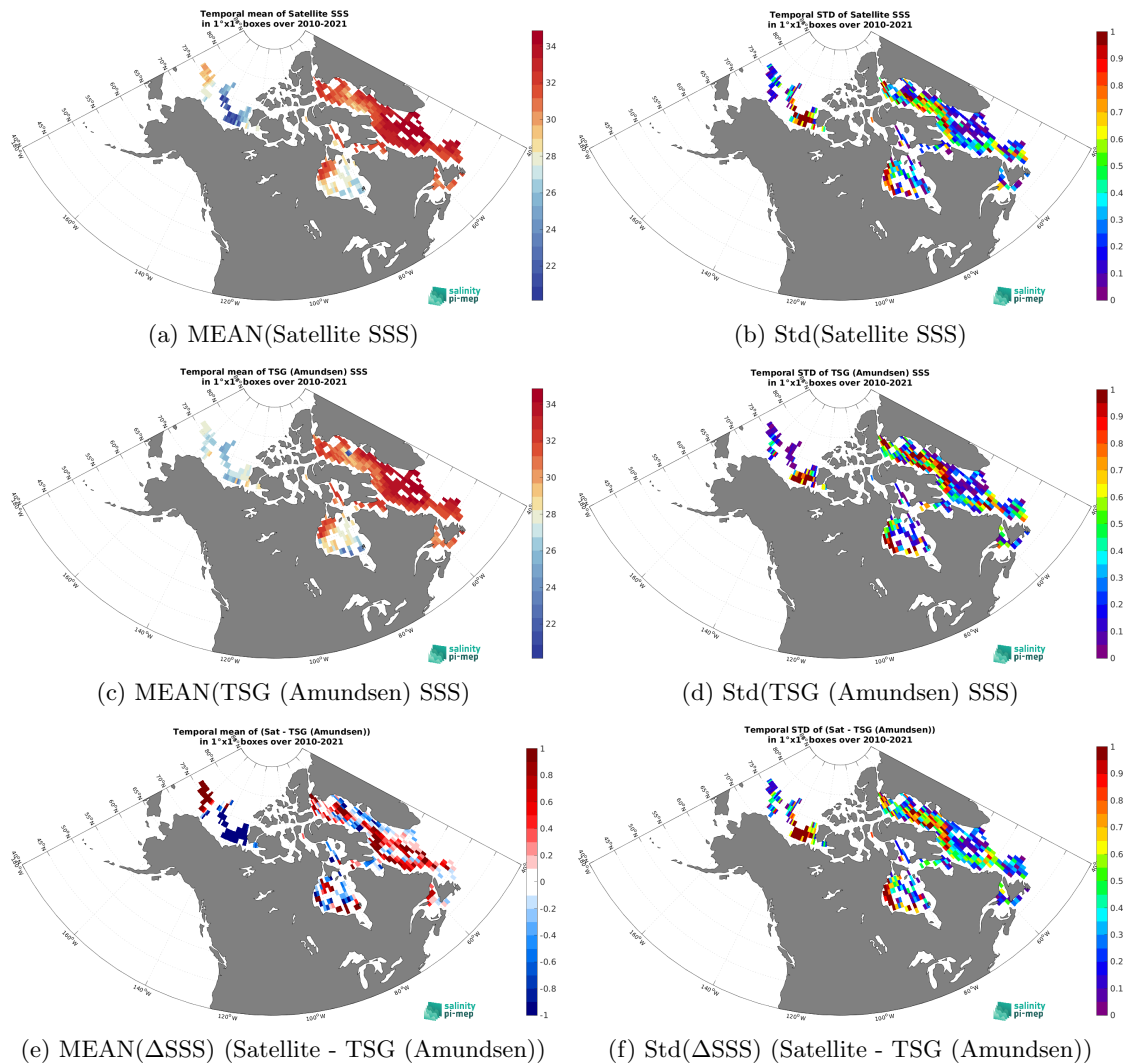
Figure 7: Temporal mean (left) and Std (right) of SSS from CCI SSS L4 Merged-OI v4.41 - 7-day running (ESA) (top), TSG (Amundsen) (middle), and of \Delta SSS (Satellite - TSG (Amundsen)). Only match-up pairs are used to generate these maps.
