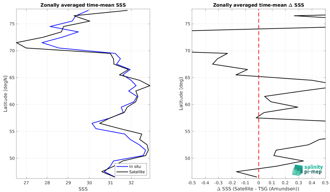
Figure 9: Left panel: Zonal mean SSS from CCI SSS L4 Merged-OI v4.41 - 7-day running (ESA) satellite product (black) and from TSG (Amundsen) (blue). Right panel: Zonal mean of \Delta SSS (Satellite - TSG (Amundsen)) for all the collected Pi-MEP match-up pairs estimated over the full satellite product period.
