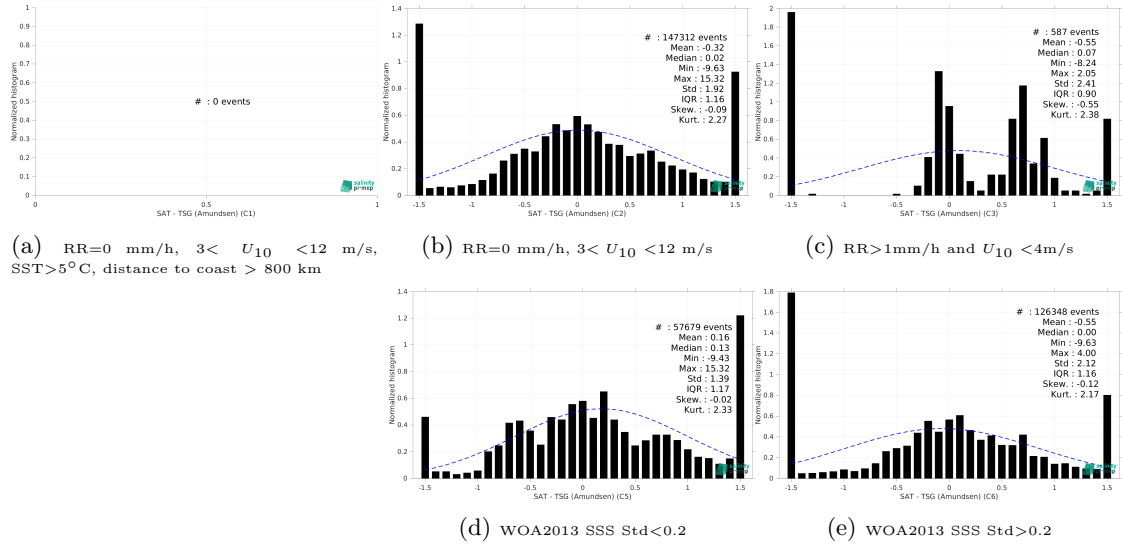
Figure 15: Normalized histogram of \Delta SSS (CCI SSS L4 Merged-OI v4.41 - 7-day running (ESA) - TSG (Amundsen)) for 5 different subdatasets corresponding to: RR=0 mm/h, 3 < U_{10} < 12 m/s, SST > 5°C, distance to coast > 800 km (a), RR=0 mm/h, 3 < U_{10} < 12 m/s (b), RR > 1mm/h and U_{10} < 4 m/s (c), WOA2013 SSS Std < 0.2 (d), WOA2013 SSS Std > 0.2 (e).
