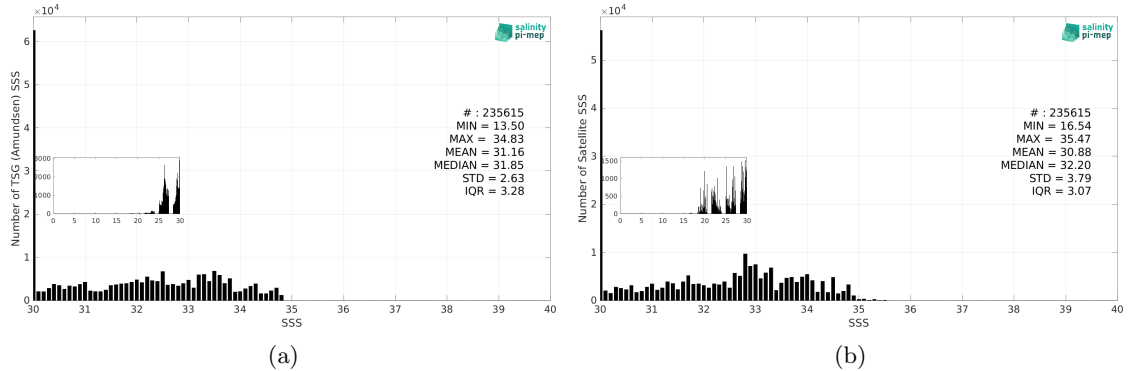
Figure 3: Histograms of SSS from TSG (Amundsen) (a) and CCI SSS L4 Merged-OI v4.41 - 7-day running (ESA) (b) considering all match-up pairs per bins of 0.1 over the Global Ocean Pi-MEP region and for the full satellite product period.
