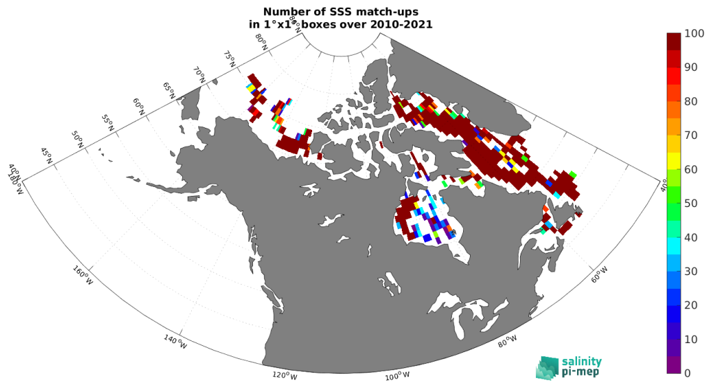
Figure 5: Number of SSS match-ups between TSG (Amundsen) SSS and the CCI SSS L4 Merged-OI v4.41 - 7-day running (ESA) SSS product for the Global Ocean Pi-MEP region over 1^\circ \times 1^\circ boxes and for the full satellite product period.
