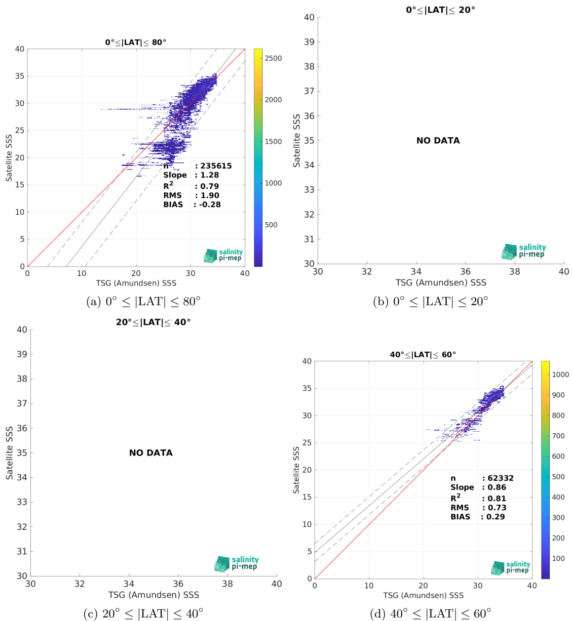
Figure 10: Contour maps of the concentration of CCI SSS L4 Merged-OI v4.41 - 7-day running (ESA) SSS (y-axis) versus TSG (Amundsen) SSS (x-axis) at match-up pairs for different latitude bands. For each plot, the red line shows x=y . The black thin and dashed lines indicate a linear fit through the data cloud and the \pm 95\% confidence levels, respectively. The number match-up pairs n , the slope and R^2 coefficient of the linear fit, the root mean square (RMS) and the mean bias between satellite and in situ data are indicated for each latitude band in each plots.
