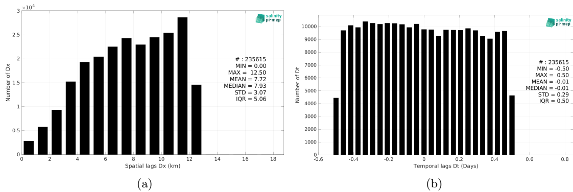
Figure 6: Histograms of the spatial (a) and temporal (b) lags between the location/time of the TSG (Amundsen) measurement and the date of the corresponding CCI SSS L4 Merged-OI v4.41 - 7-day running (ESA) SSS pixel.
