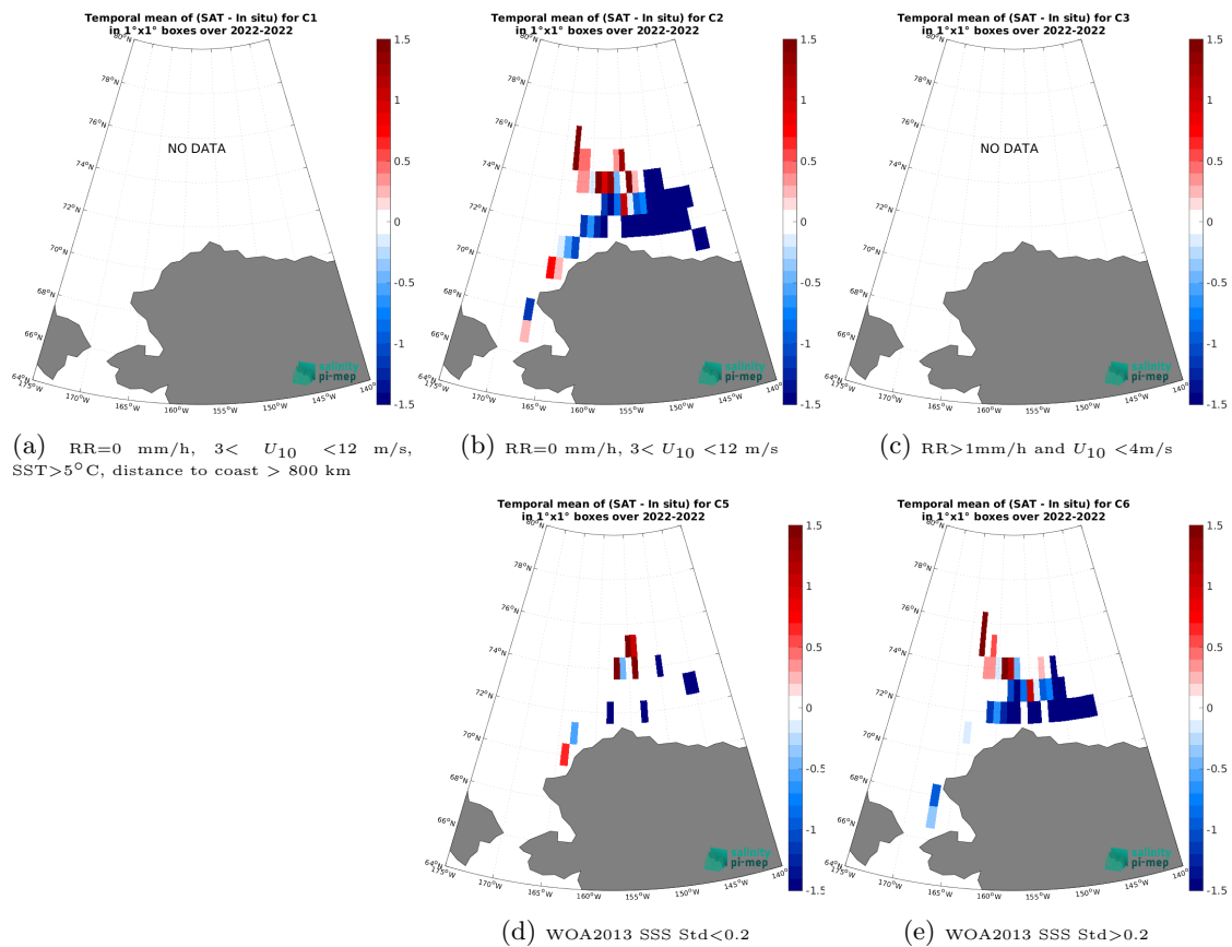
Figure 14: Temporal mean gridded over spatial boxes of size 1^\circ \times 1^\circ of \Delta SSS (CCI SSS L4 Merged-OI v4.41 - 7-day running (ESA) - SASSIE) for 5 different subdatasets corresponding to:RR=0 mm/h, 3 < U_{10} < 12 m/s, SST >5^\circ\text{C} , distance to coast > 800 km (a), RR=0 mm/h, 3 < U_{10} < 12 m/s (b), RR >1 mm/h and U_{10} < 4 m/s (c), WOA2013 SSS Std <0.2 (d), WOA2013 SSS Std >0.2 (e).
