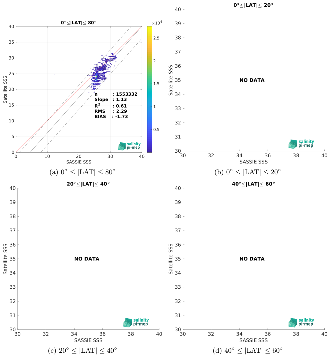
Figure 10: Contour maps of the concentration of CCI SSS L4 Merged-OI v4.41 - 7-day running (ESA) SSS (y-axis) versus SASSIE SSS (x-axis) at match-up pairs for different latitude bands. For each plot, the red line shows x=y . The black thin and dashed lines indicate a linear fit through the data cloud and the \pm 95\% confidence levels, respectively. The number match-up pairs n , the slope and R^2 coefficient of the linear fit, the root mean square (RMS) and the mean bias between satellite and in situ data are indicated for each latitude band in each plots.
