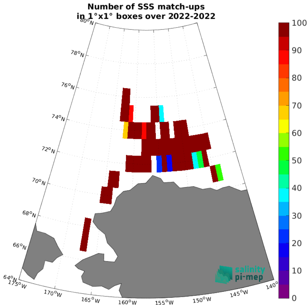
Figure 5: Number of SSS match-ups between SASSIE SSS and the CCI SSS L4 Merged-OI v4.41 - 7-day running (ESA) SSS product for the Global Ocean Pi-MEP region over 1^\circ \times 1^\circ boxes and for the full satellite product period.
