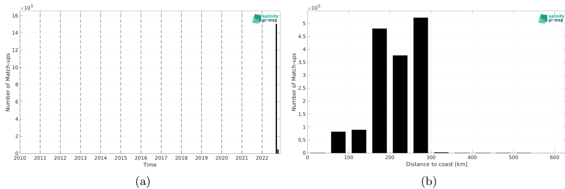
Figure 2: Number of match-ups between SASSIE and CCI SSS L4 Merged-OI v4.41 - 7-day running (ESA) SSS as a function of time (a) and as function of the distance to coast (b) over the Global Ocean Pi-MEP region and for the full satellite product period.
