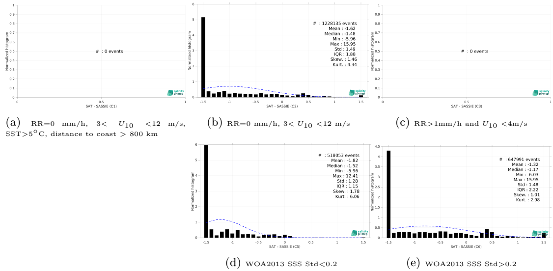
Figure 15: Normalized histogram of \Delta SSS (CCI SSS L4 Merged-OI v4.41 - 7-day running (ESA) - SASSIE) for 5 different subdatasets corresponding to: RR=0 mm/h, 3 < U_{10} < 12 m/s, SST > 5°C, distance to coast > 800 km (a), RR=0 mm/h, 3 < U_{10} < 12 m/s (b), RR > 1mm/h and U_{10} < 4 m/s (c), WOA2013 SSS Std < 0.2 (d), WOA2013 SSS Std > 0.2 (e).
