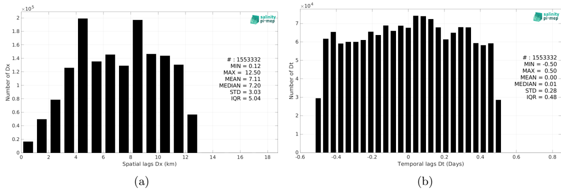
Figure 6: Histograms of the spatial (a) and temporal (b) lags between the location/time of the SASSIE measurement and the date of the corresponding CCI SSS L4 Merged-OI v4.41 - 7-day running (ESA) SSS pixel.
