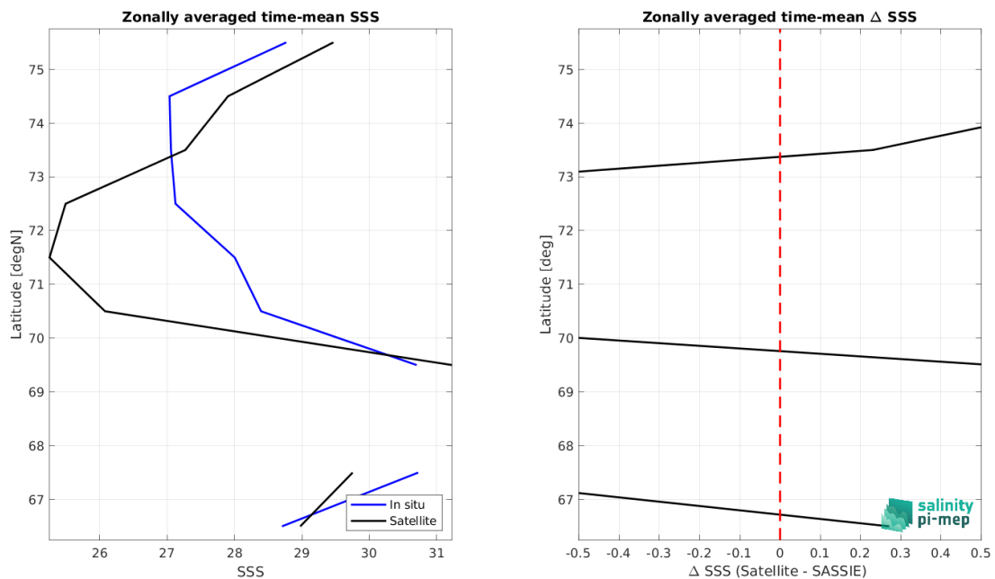
Figure 9: Left panel: Zonal mean SSS from CCI SSS L4 Merged-OI v4.41 - 7-day running (ESA) satellite product (black) and from SASSIE (blue). Right panel: Zonal mean of \Delta SSS (Satellite - SASSIE) for all the collected Pi-MEP match-up pairs estimated over the full satellite product period.
