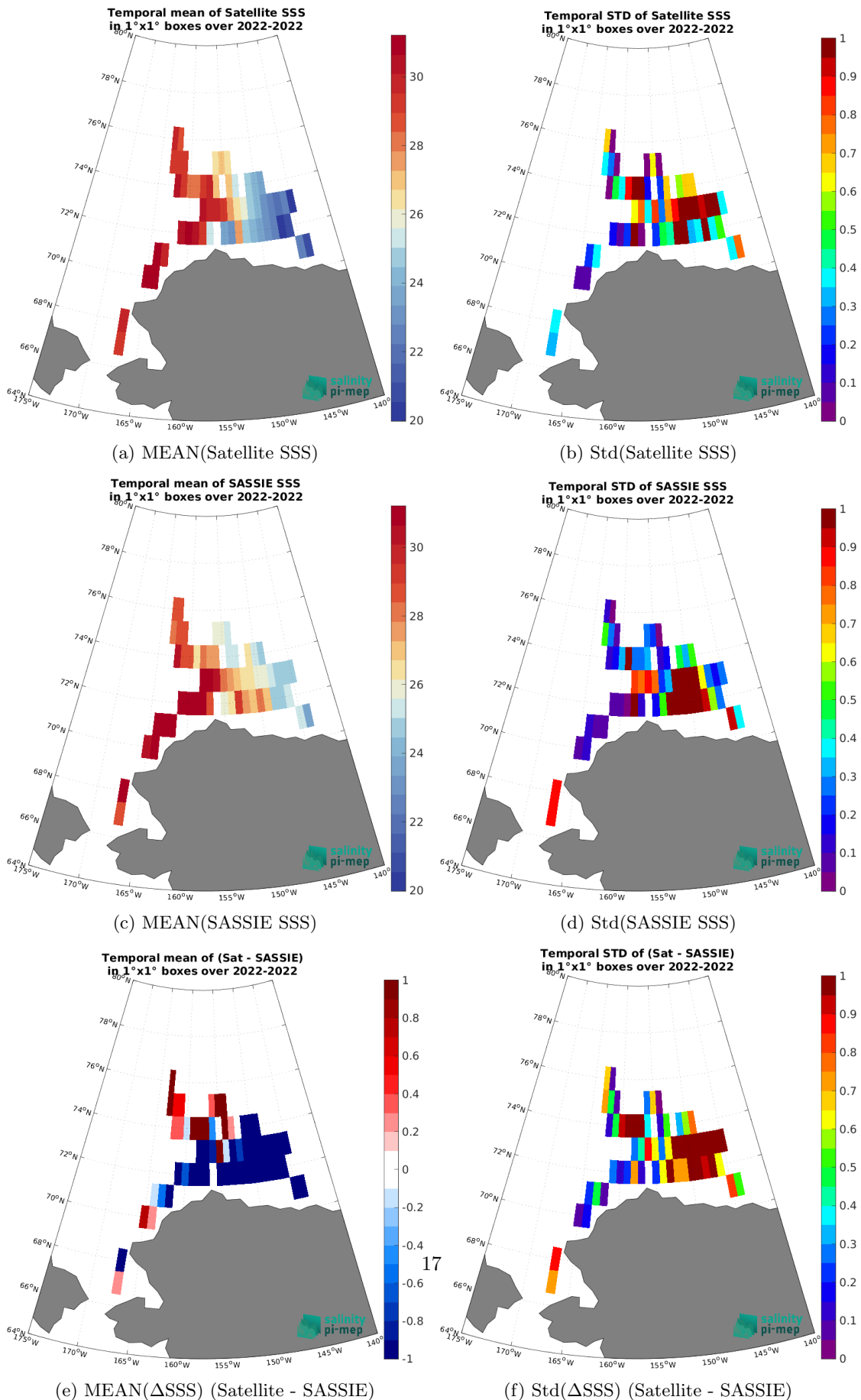
Figure 7: Temporal mean (left) and Std (right) of SSS from CCI SSS L4 Merged-OI v4.41 - 7-day running (ESA) (top), SASSIE (middle), and of \Delta SSS (Satellite - SASSIE). Only match-up pairs are used to generate these maps.
