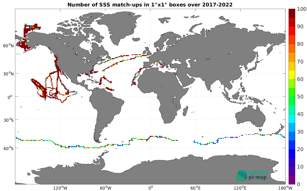
Figure 5: Number of SSS match-ups between Saildrone SSS and the CCI SSS L4 Merged-OI v4.41 - 7-day running (ESA) SSS product for the Global Ocean Pi-MEP region over 1^\circ \times 1^\circ boxes and for the full satellite product period.
