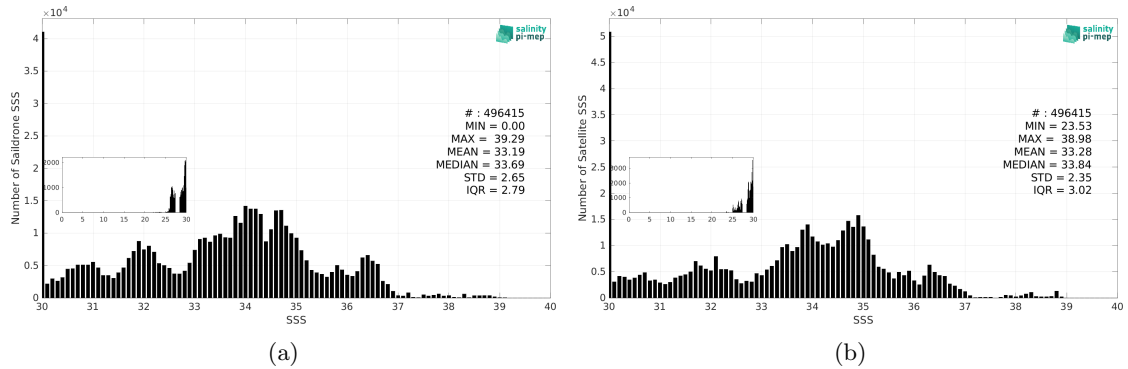
Figure 3: Histograms of SSS from Sairdrone (a) and CCI SSS L4 Merged-OI v4.41 - 7-day running (ESA) (b) considering all match-up pairs per bins of 0.1 over the Global Ocean Pi-MEP region and for the full satellite product period.
