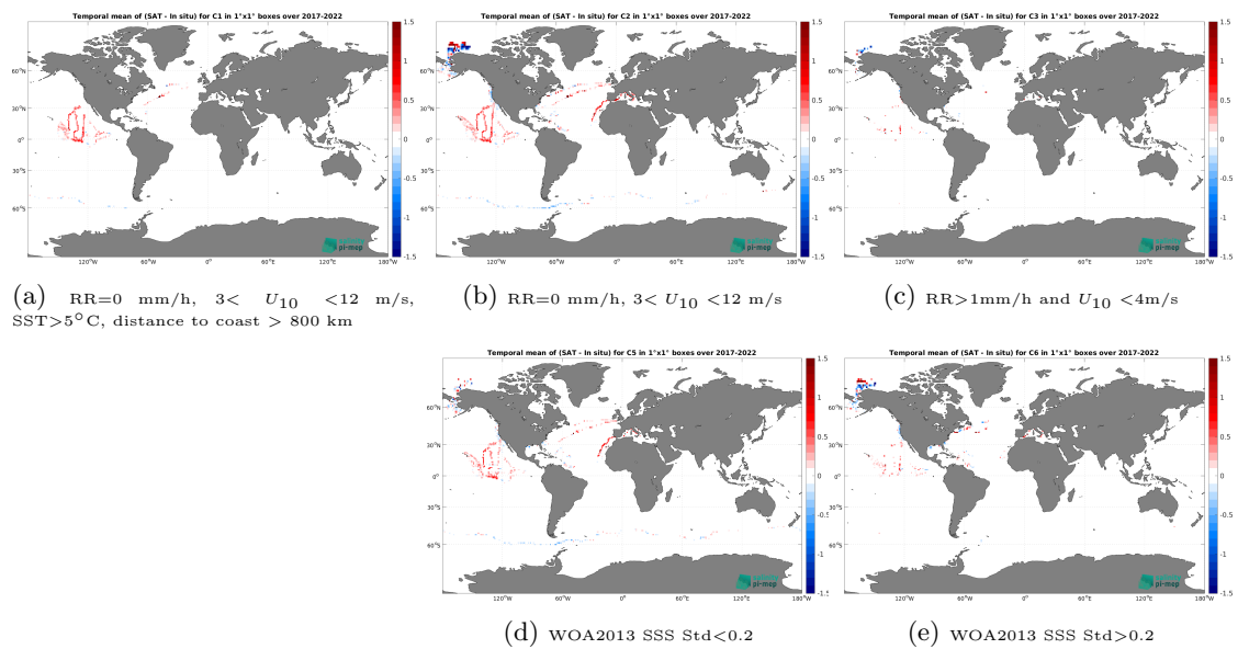
Figure 14: Temporal mean gridded over spatial boxes of size 1^\circ \times 1^\circ of \Delta\text{SSS} (CCI SSS L4 Merged-OI v4.41 - 7-day running (ESA) - Saildrone) for 5 different subdatasets corresponding to:RR=0 mm/h, 3 < U_{10} < 12 m/s, SST > 5^\circ\text{C} , distance to coast > 800 km (a), RR=0 mm/h, 3 < U_{10} < 12 m/s (b), RR > 1 mm/h and U_{10} < 4 m/s (c), WOA2013 SSS Std < 0.2 (d), WOA2013 SSS Std > 0.2 (e).
