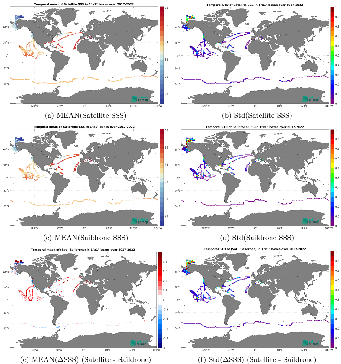
Figure 7: Temporal mean (left) and Std (right) of SSS from CCI SSS L4 Merged-OI v4.41 - 7-day running (ESA) (top), Saildrone (middle), and of \Delta SSS (Satellite - Saildrone). Only match-up pairs are used to generate these maps.
