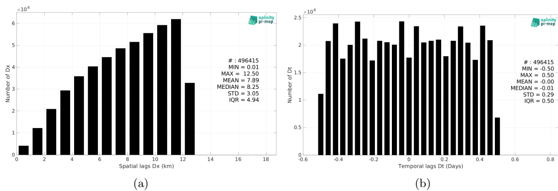
Figure 6: Histograms of the spatial (a) and temporal (b) lags between the location/time of the Saildrone measurement and the date of the corresponding CCI SSS L4 Merged-OI v4.41 - 7-day running (ESA) SSS pixel.
