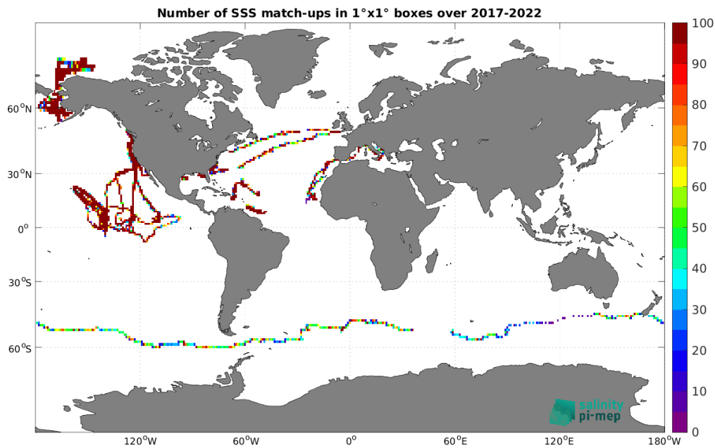
Figure 5: Number of SSS match-ups between Saildrone SSS and the CCI SSS L4 Merged-OI v4.41 - 7-day running (ESA) SSS product for the Global Ocean Pi-MEP region over 1°x1° boxes and for the full satellite product period.
