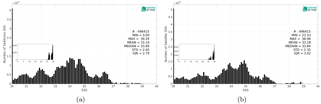
Figure 3: Histograms of SSS from Saildrone (a) and CCI SSS L4 Merged-OI v4.41 - 7-day running (ESA) (b) considering all match-up pairs per bins of 0.1 over the Global Ocean Pi-MEP region and for the full satellite product period.
