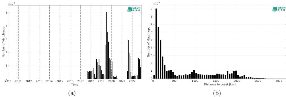
Figure 2: Number of match-ups between Saildrone and CCI SSS L4 Merged-OI v4.41 - 7-day running (ESA) SSS as a function of time (a) and as function of the distance to coast (b) over the Global Ocean Pi-MEP region and for the full satellite product period.
