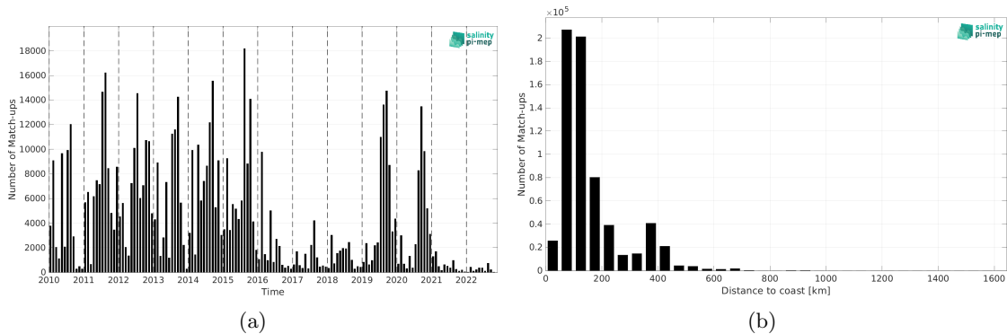
Figure 2: Number of match-ups between ICES and CCI SSS L4 Merged-OI v4.41 - 7-day running (ESA) SSS as a function of time (a) and as function of the distance to coast (b) over the Global Ocean Pi-MEP region and for the full satellite product period.
