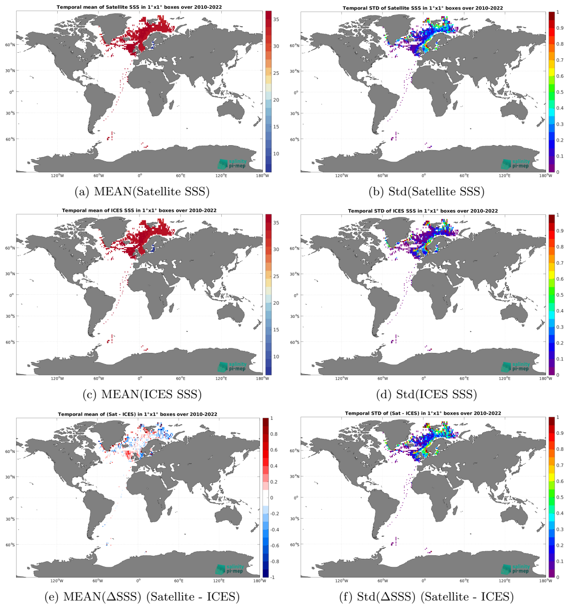
Figure 7: Temporal mean (left) and Std (right) of SSS from CCI SSS L4 Merged-OI v4.41 - 7-day running (ESA) (top), ICES (middle), and of \Delta SSS (Satellite - ICES). Only match-up pairs are used to generate these maps.
