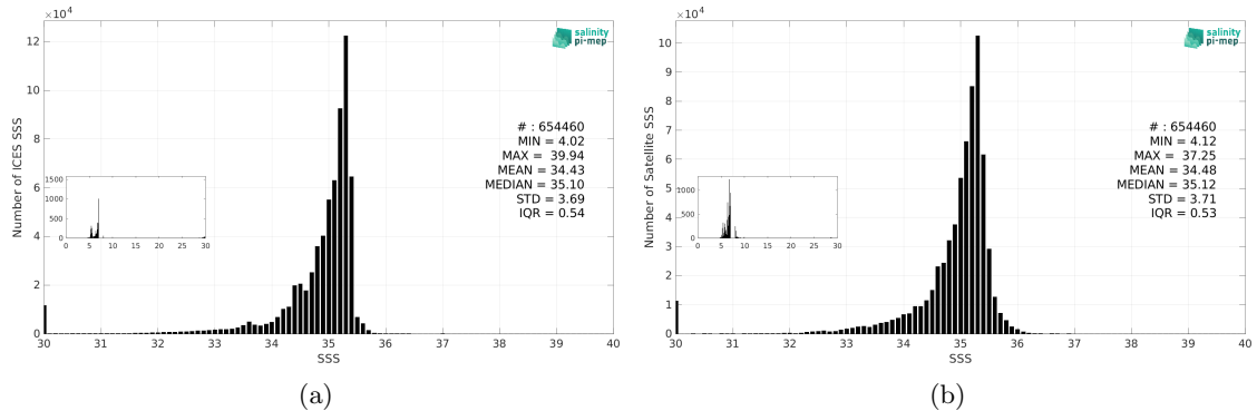
Figure 3: Histograms of SSS from ICES (a) and CCI SSS L4 Merged-OI v4.41 - 7-day running (ESA) (b) considering all match-up pairs per bins of 0.1 over the Global Ocean Pi-MEP region and for the full satellite product period.
