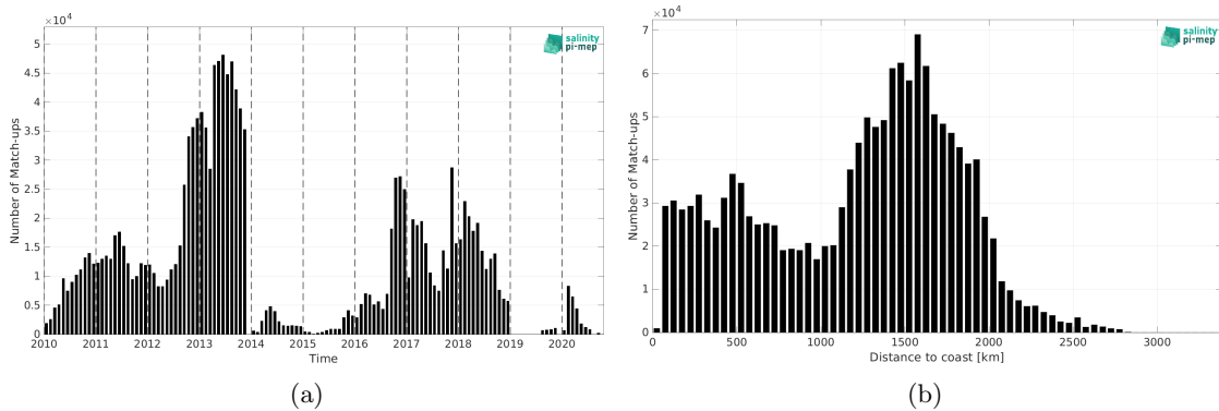
Figure 2: Number of match-ups between Surface drifters and CCI SSS L4 Merged-OI v4.41 - 7-day running (ESA) SSS as a function of time (a) and as function of the distance to coast (b) over the Global Ocean Pi-MEP region and for the full satellite product period.
