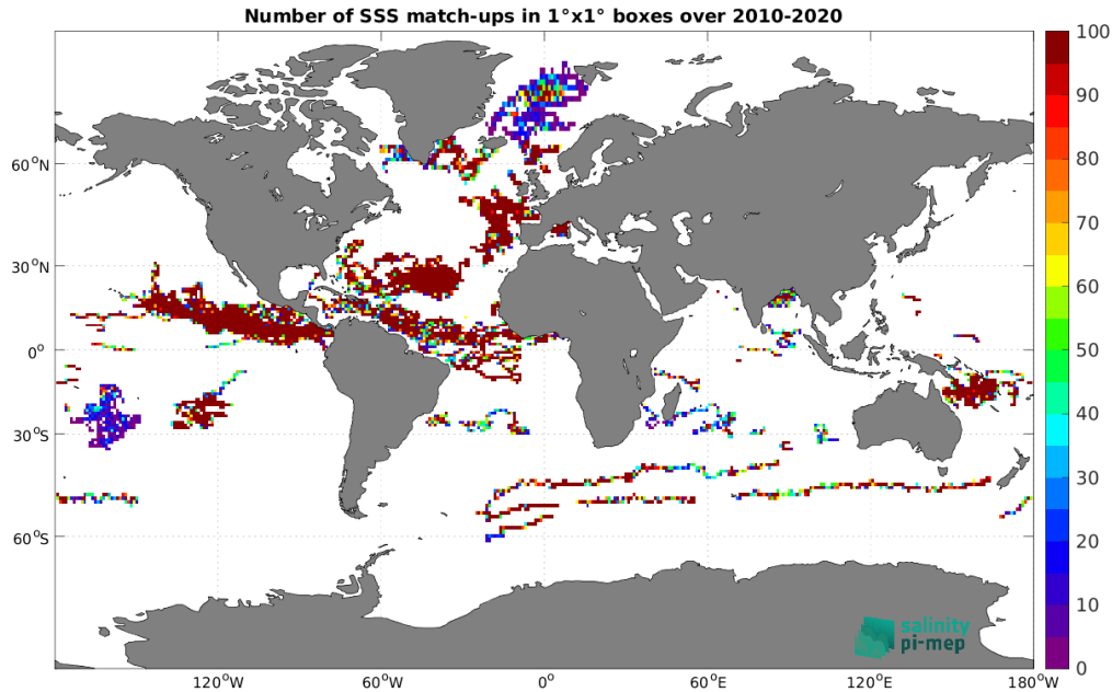
Figure 4: Number of SSS match-ups between Surface drifters SSS and the CCI SSS L4 Merged-OI v4.41 - 7-day running (ESA) SSS product for the Global Ocean Pi-MEP region over 1^\circ \times 1^\circ boxes and for the full satellite product period.
