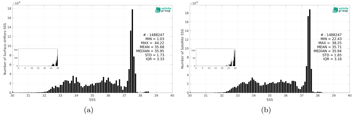
Figure 3: Histograms of SSS from Surface drifters (a) and CCI SSS L4 Merged-OI v4.41 - 7-day running (ESA) (b) considering all match-up pairs per bins of 0.1 over the Global Ocean Pi-MEP region and for the full satellite product period.
