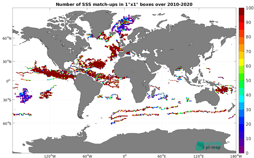
Figure 4: Number of SSS match-ups between Surface drifters SSS and the CCI SSS L4 Merged-OI v4.41 - 7-day running (ESA) SSS product for the Global Ocean Pi-MEP region over 1°×1° boxes and for the full satellite product period.
