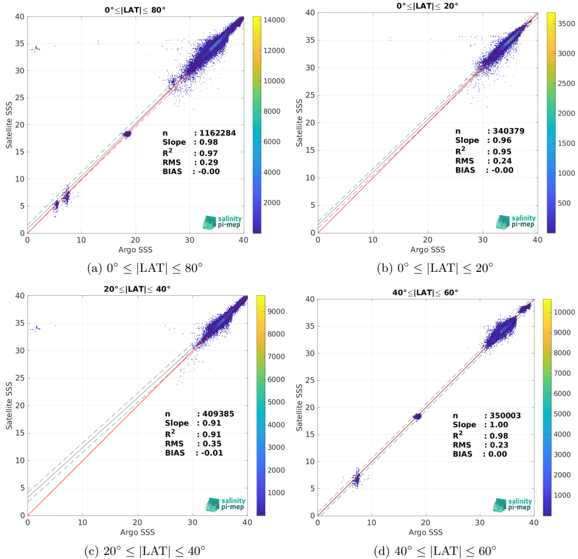
Figure 10: Contour maps of the concentration of CCI SSS L4 Merged-OI v4.41 - 7-day running (ESA) SSS (y-axis) versus Argo SSS (x-axis) at match-up pairs for different latitude bands. For each plot, the red line shows x=y . The black thin and dashed lines indicate a linear fit through the data cloud and the \pm 95\% confidence levels, respectively. The number match-up pairs n , the slope and R^2 coefficient of the linear fit, the root mean square (RMS) and the mean bias between satellite and in situ data are indicated for each latitude band in each plots.
