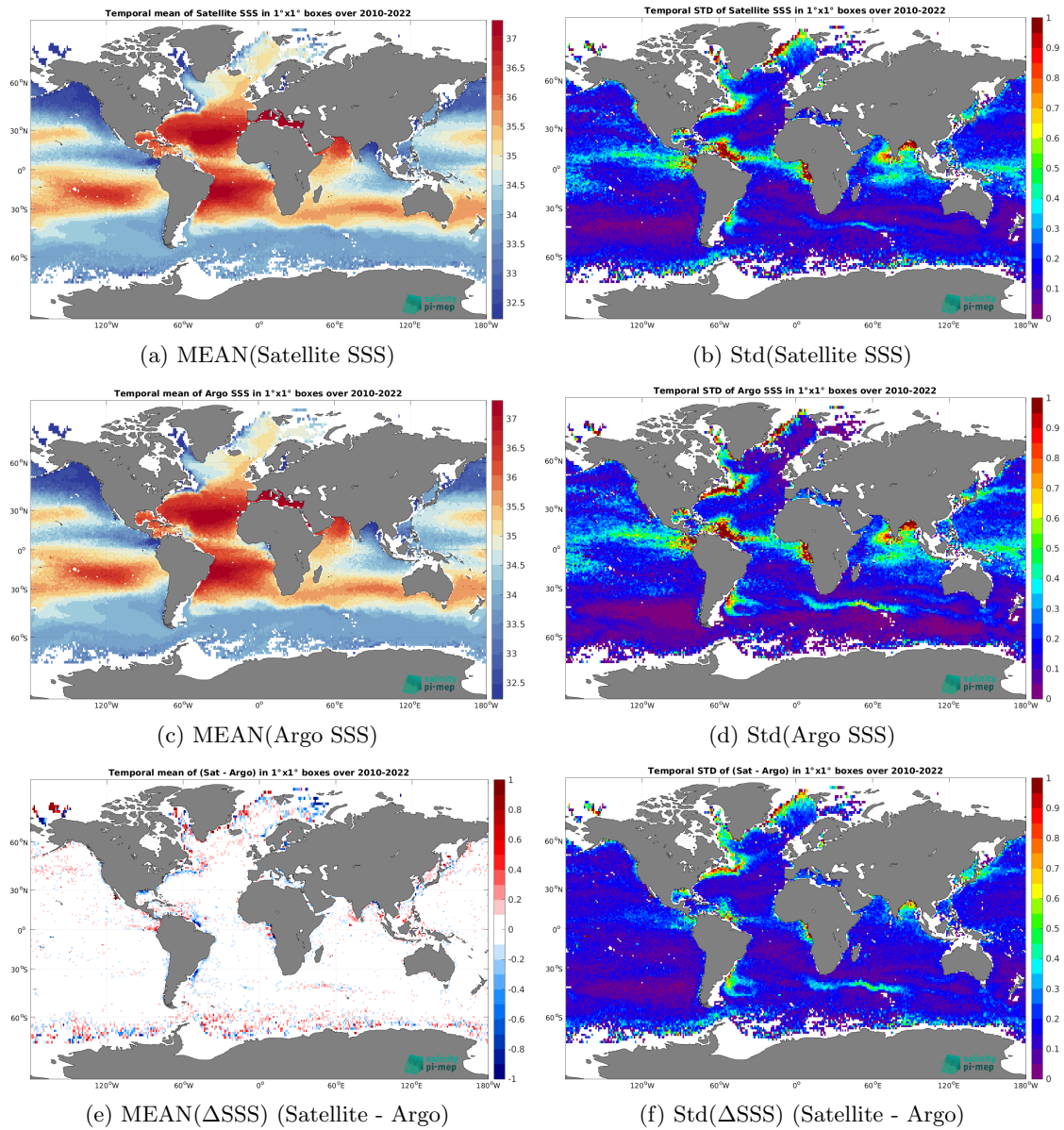
Figure 7: Temporal mean (left) and Std (right) of SSS from CCI SSS L4 Merged-OI v4.41 - 7-day running (ESA) (top), Argo (middle), and of \Delta SSS (Satellite - Argo). Only match-up pairs are used to generate these maps.
