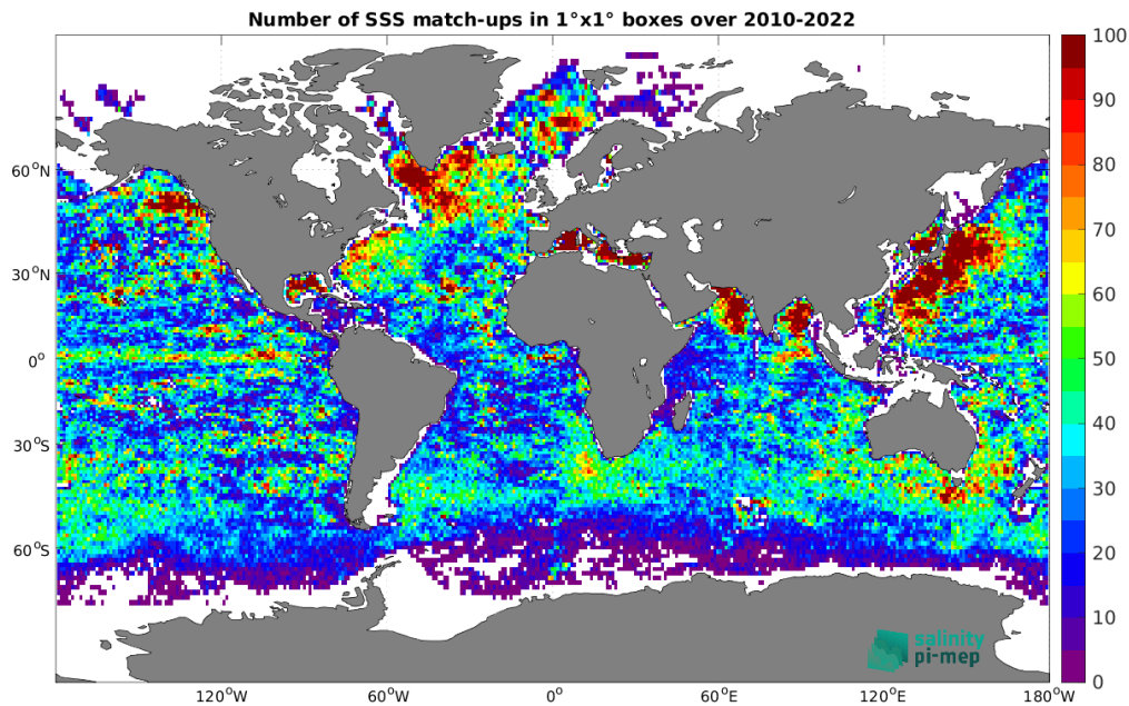
Figure 5: Number of SSS match-ups between Argo SSS and the CCI SSS L4 Merged-OI v4.41 - 7-day running (ESA) SSS product for the Global Ocean Pi-MEP region over 1^\circ \times 1^\circ boxes and for the full satellite product period.
