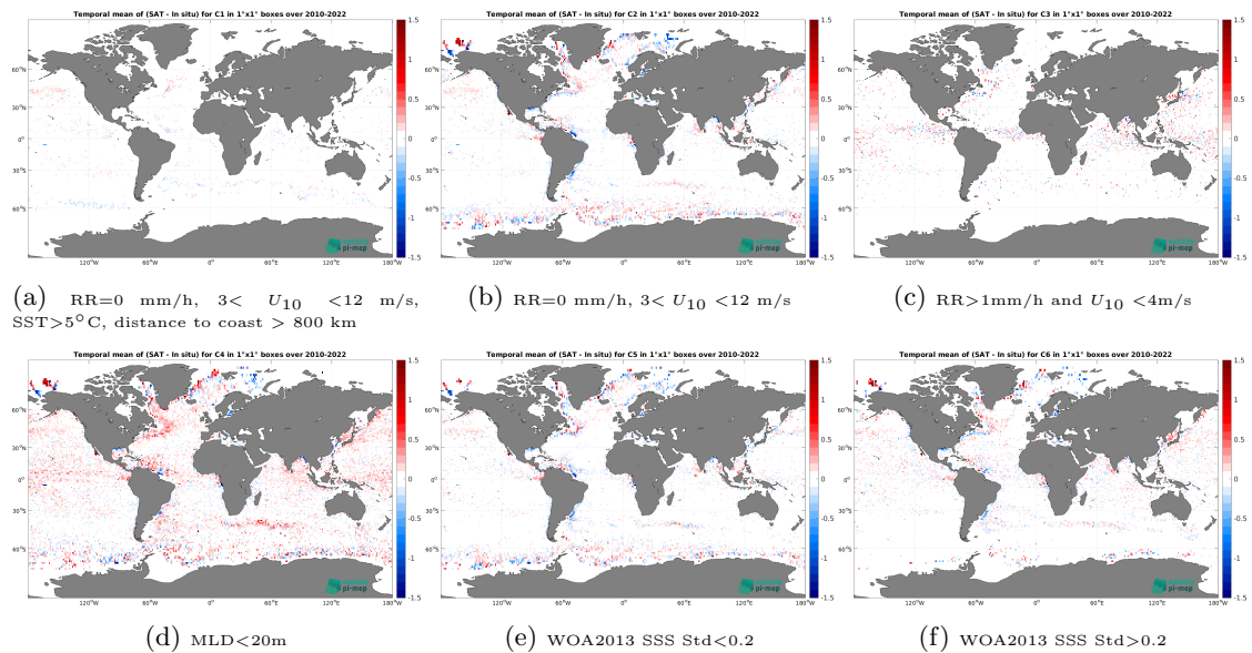
Figure 14: Temporal mean gridded over spatial boxes of size 1^\circ \times 1^\circ of \Delta\text{SSS} (CCI SSS L4 Merged-OI v4.41 - 7-day running (ESA) - Argo) for 6 different subdatasets corresponding to:RR=0 mm/h, 3 < U_{10} < 12 m/s, SST>5°C, distance to coast > 800 km (a), RR=0 mm/h, 3 < U_{10} < 12 m/s (b), RR>1mm/h and U_{10} < 4 m/s (c),MLD<20m (d),WOA2013 SSS Std<0.2 (e),WOA2013 SSS Std>0.2 (f).
