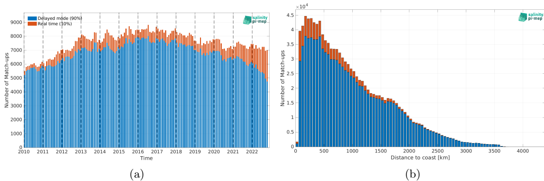
Figure 2: Number of match-ups between Argo and CCI SSS L4 Merged-OI v4.41 - 7-day running (ESA) SSS as a function of time (a) and as function of the distance to coast (b) over the Global Ocean Pi-MEP region and for the full satellite product period.
