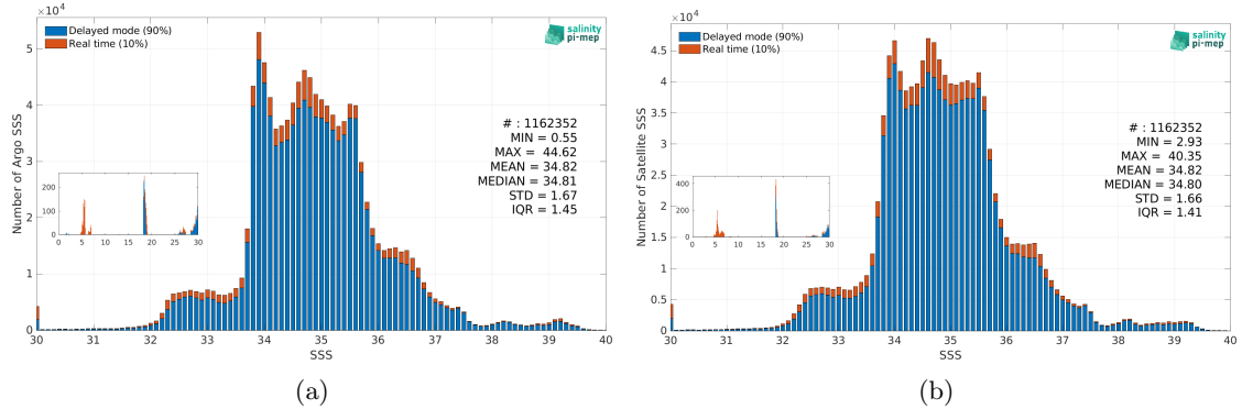
Figure 3: Histograms of SSS from Argo (a) and CCI SSS L4 Merged-OI v4.41 - 7-day running (ESA) (b) considering all match-up pairs per bins of 0.1 over the Global Ocean Pi-MEP region and for the full satellite product period.
