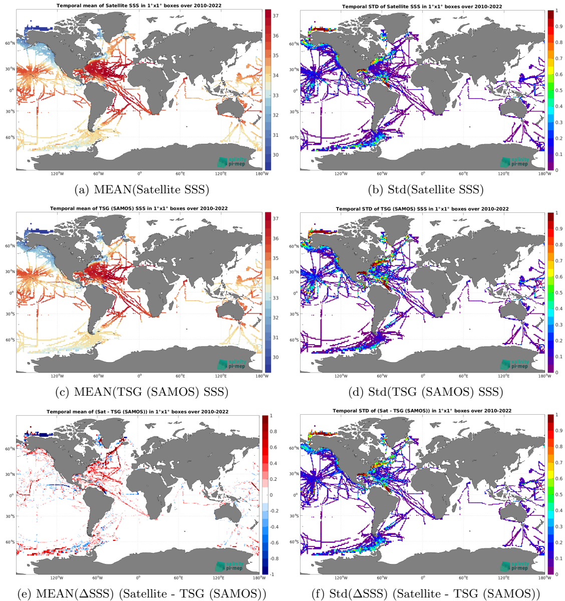
Figure 7: Temporal mean (left) and Std (right) of SSS from CCI SSS L4 Merged-OI v4.41 - 30-day running (ESA) (top), TSG (SAMOS) (middle), and of \Delta SSS (Satellite - TSG (SAMOS)). Only match-up pairs are used to generate these maps.
