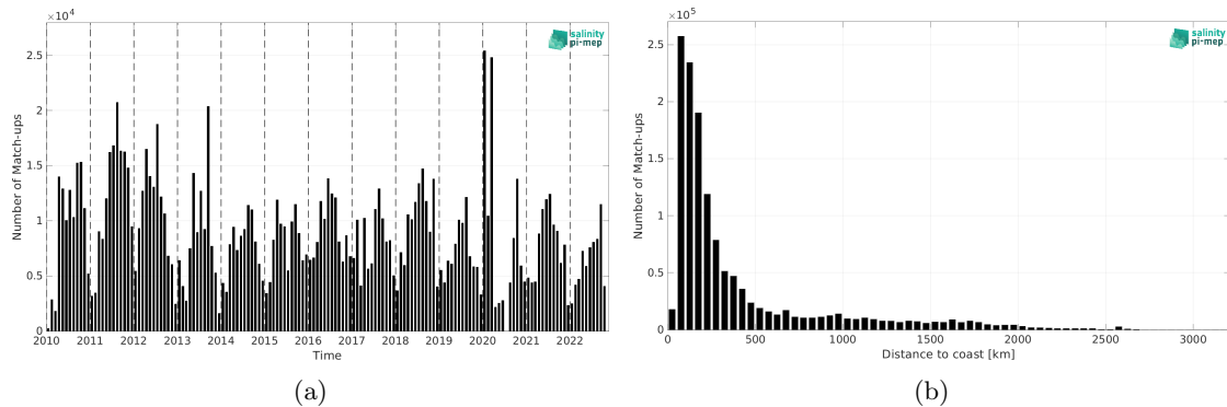
Figure 2: Number of match-ups between TSG (SAMOS) and CCI SSS L4 Merged-OI v4.41 - 30-day running (ESA) SSS as a function of time (a) and as function of the distance to coast (b) over the Global Ocean Pi-MEP region and for the full satellite product period.
