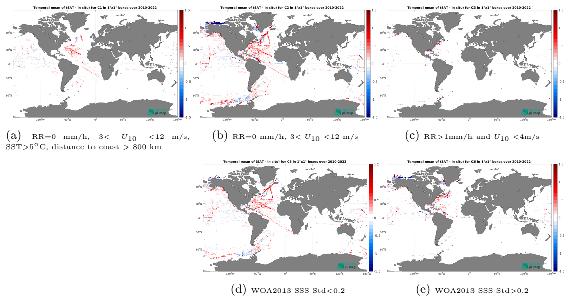
Figure 14: Temporal mean gridded over spatial boxes of size 1^\circ \times 1^\circ of \Delta SSS (CCI SSS L4 Merged-OI v4.41 - 30-day running (ESA) - TSG (SAMOS)) for 5 different subdatasets corresponding to:RR=0 mm/h, 3 < U_{10} < 12 m/s, SST > 5^\circ C, distance to coast > 800 km (a), RR=0 mm/h, 3 < U_{10} < 12 m/s (b), RR > 1 mm/h and U_{10} < 4 m/s (c), WOA2013 SSS Std < 0.2 (d), WOA2013 SSS Std > 0.2 (e).
