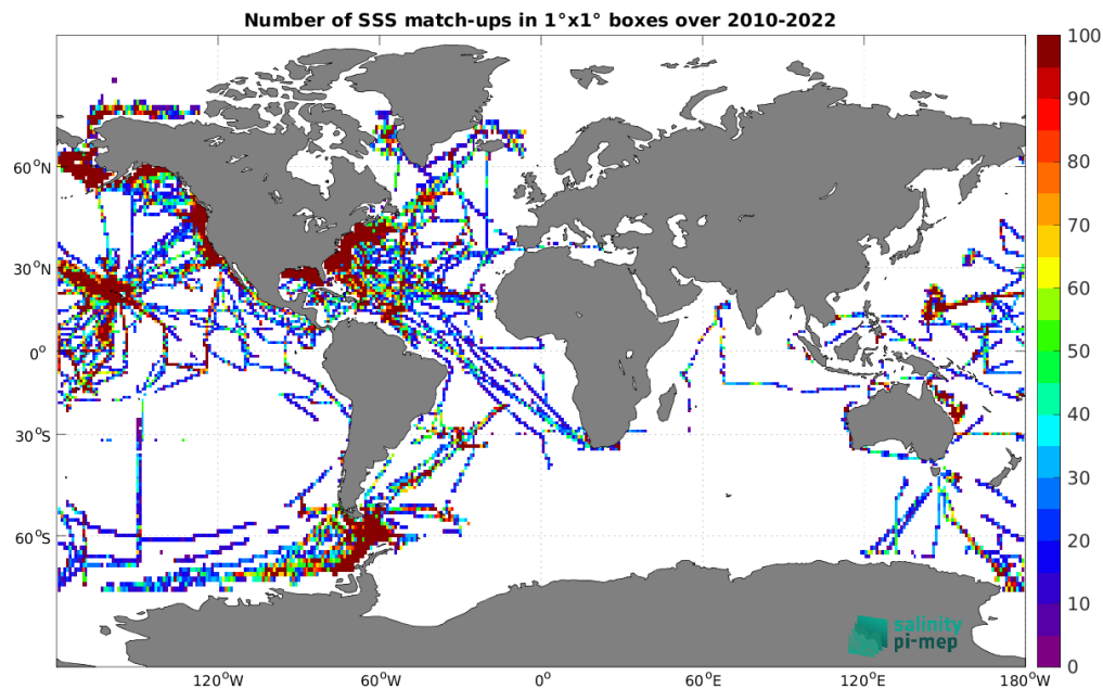
Figure 5: Number of SSS match-ups between TSG (SAMOS) SSS and the CCI SSS L4 Merged-OI v4.41 - 30-day running (ESA) SSS product for the Global Ocean Pi-MEP region over 1^\circ \times 1^\circ boxes and for the full satellite product period.
