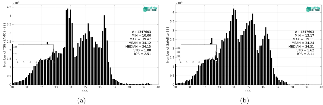
Figure 3: Histograms of SSS from TSG (SAMOS) (a) and CCI SSS L4 Merged-OI v4.41 - 30-day running (ESA) (b) considering all match-up pairs per bins of 0.1 over the Global Ocean Pi-MEP region and for the full satellite product period.
