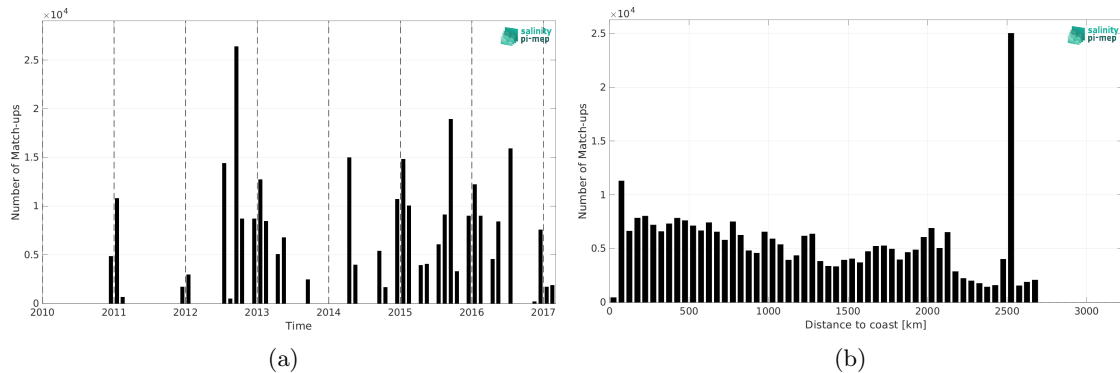
Figure 2: Number of match-ups between TSG (NCEI-0170743) and CCI SSS L4 Merged-OI v4.41 - 30-day running (ESA) SSS as a function of time (a) and as function of the distance to coast (b) over the Global Ocean Pi-MEP region and for the full satellite product period.
