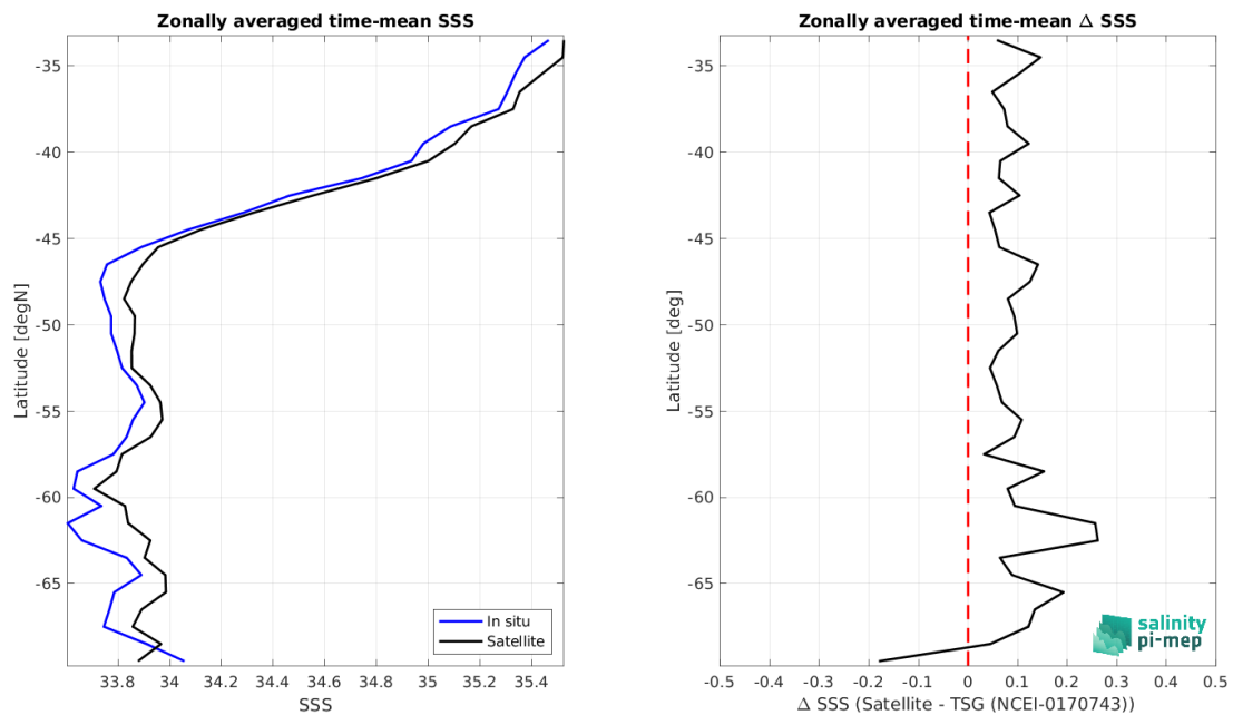
Figure 9: Left panel: Zonal mean SSS from CCI SSS L4 Merged-OI v4.41 - 30-day running (ESA) satellite product (black) and from TSG (NCEI-0170743) (blue). Right panel: Zonal mean of \Delta SSS (Satellite - TSG (NCEI-0170743)) for all the collected Pi-MEP match-up pairs estimated over the full satellite product period.
