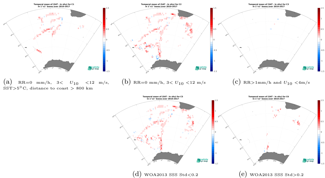
Figure 14: Temporal mean gridded over spatial boxes of size 1^\circ \times 1^\circ of \Delta\text{SSS} (CCI SSS L4 Merged-OI v4.41 - 30-day running (ESA) - TSG (NCEI-0170743)) for 5 different subdatasets corresponding to:RR=0 mm/h, 3 < U_{10} < 12 m/s, SST >5^\circ\text{C} , distance to coast > 800 km (a), RR=0 mm/h, 3 < U_{10} < 12 m/s (b), RR >1 mm/h and U_{10} < 4 m/s (c), WOA2013 SSS Std <0.2 (d), WOA2013 SSS Std >0.2 (e).
