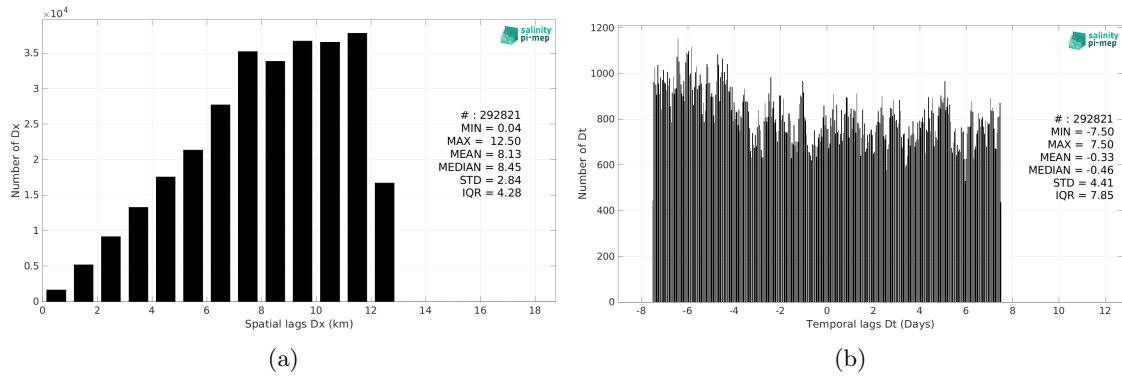
Figure 6: Histograms of the spatial (a) and temporal (b) lags between the location/time of the TSG (NCEI-0170743) measurement and the date of the corresponding CCI SSS L4 Merged-OI v4.41 - 30-day running (ESA) SSS pixel.
