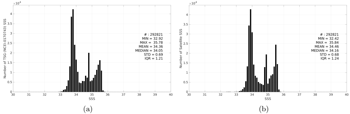
Figure 3: Histograms of SSS from TSG (NCEI-0170743) (a) and CCI SSS L4 Merged-OI v4.41 - 30-day running (ESA) (b) considering all match-up pairs per bins of 0.1 over the Global Ocean Pi-MEP region and for the full satellite product period.
