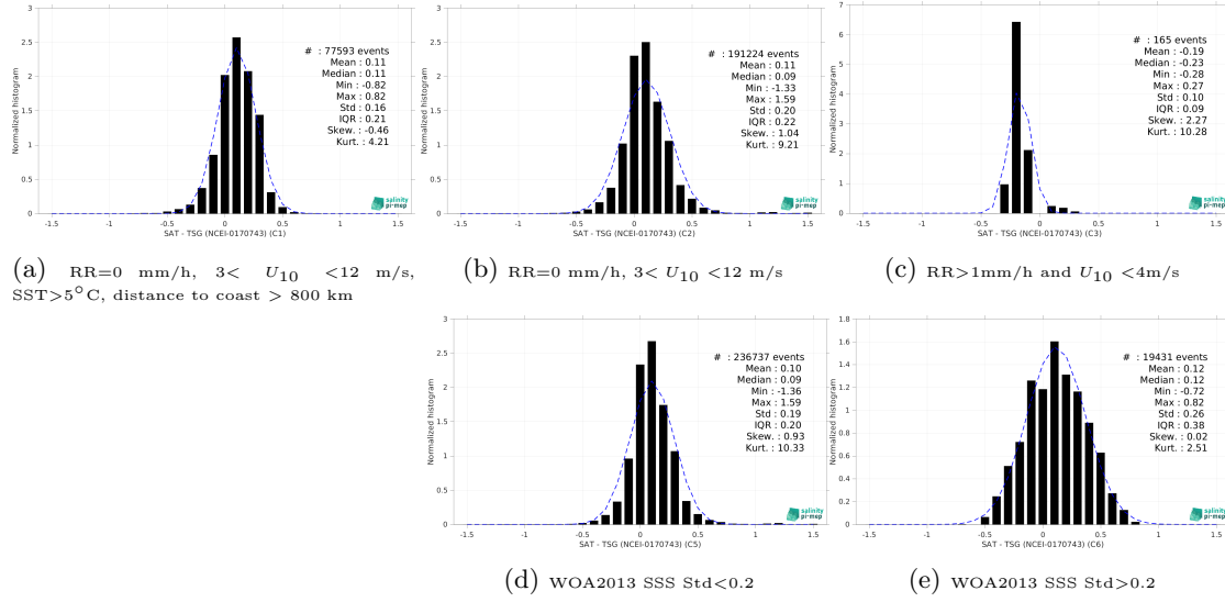
Figure 15: Normalized histogram of \Delta SSS (CCI SSS L4 Merged-OI v4.41 - 30-day running (ESA) - TSG (NCEI-0170743)) for 5 different subdatasets corresponding to: RR=0 mm/h, 3 < U_{10} < 12 m/s, SST>5°C, distance to coast > 800 km (a), RR=0 mm/h, 3 < U_{10} < 12 m/s (b), RR>1mm/h and U_{10} < 4 m/s (c), WOA2013 SSS Std<0.2 (d), WOA2013 SSS Std>0.2 (e).
