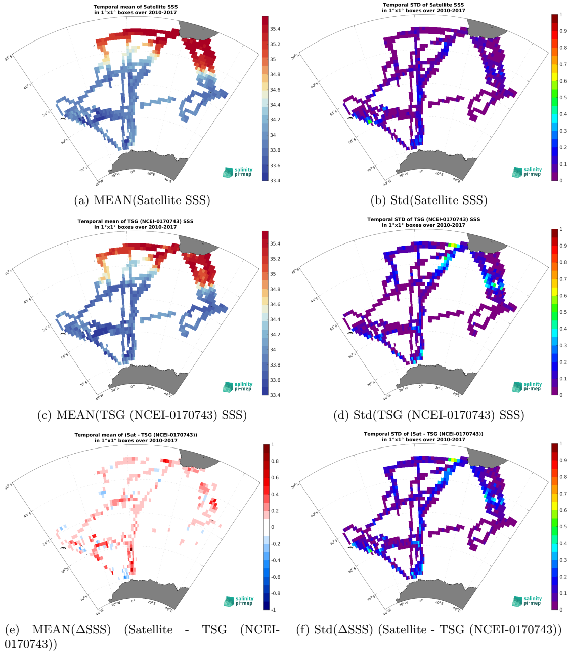
Figure 7: Temporal mean (left) and Std (right) of SSS from CCI SSS L4 Merged-OI v4.41 - 30-day running (ESA) (top), TSG (NCEI-0170743) (middle), and of \Delta SSS (Satellite - TSG (NCEI-0170743)). Only match-up pairs are used to generate these maps.
