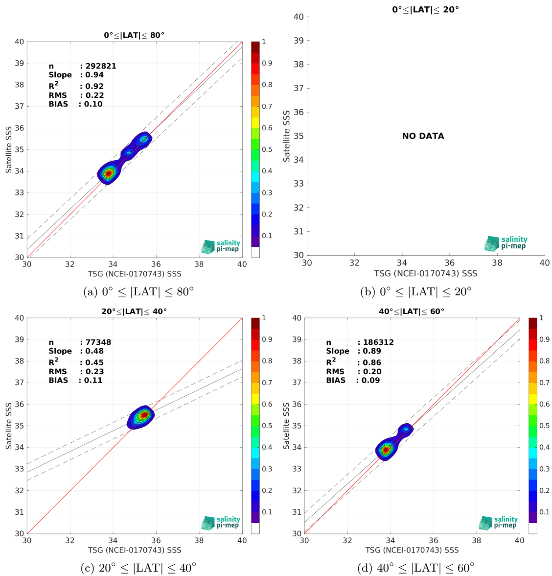
Figure 10: Contour maps of the concentration of CCI SSS L4 Merged-OI v4.41 - 30-day running (ESA) SSS (y-axis) versus TSG (NCEI-0170743) SSS (x-axis) at match-up pairs for different latitude bands. For each plot, the red line shows x=y . The black thin and dashed lines indicate a linear fit through the data cloud and the \pm 95\% confidence levels, respectively. The number match-up pairs n , the slope and R^2 coefficient of the linear fit, the root mean square (RMS) and the mean bias between satellite and in situ data are indicated for each latitude band in each plots.
