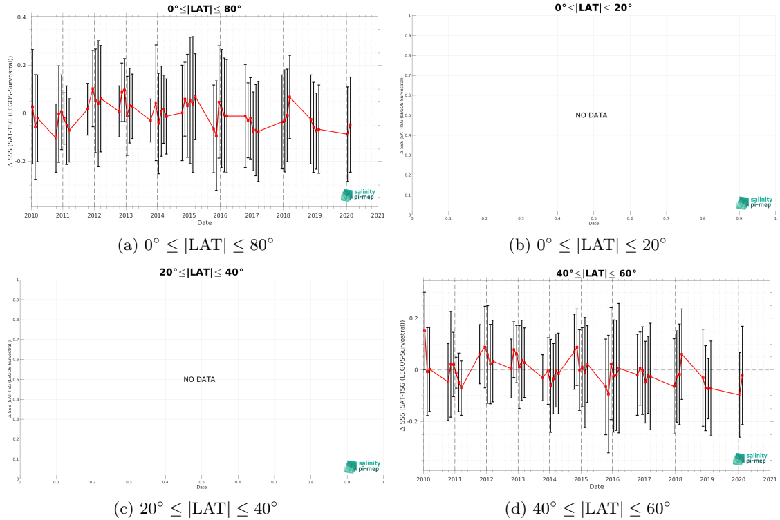
Figure 11: Monthly median (red curves) of \Delta SSS (Satellite - in situ (LEGOS-Survostral)) and \pm 1 Std (black vertical thick bars) as function of time for all the collected Pi-MEP match-up pairs estimated over the Global Ocean Pi-MEP region and for the full satellite product period are shown for different latitude bands: (a) 80^\circ\text{S}-80^\circ\text{N} , (b) 20^\circ\text{S}-20^\circ\text{N} , (c) 40^\circ\text{S}-20^\circ\text{S} and 20^\circ\text{N}-40^\circ\text{N} and (d) 60^\circ\text{S}-40^\circ\text{S} and 40^\circ\text{N}-60^\circ\text{N} .
