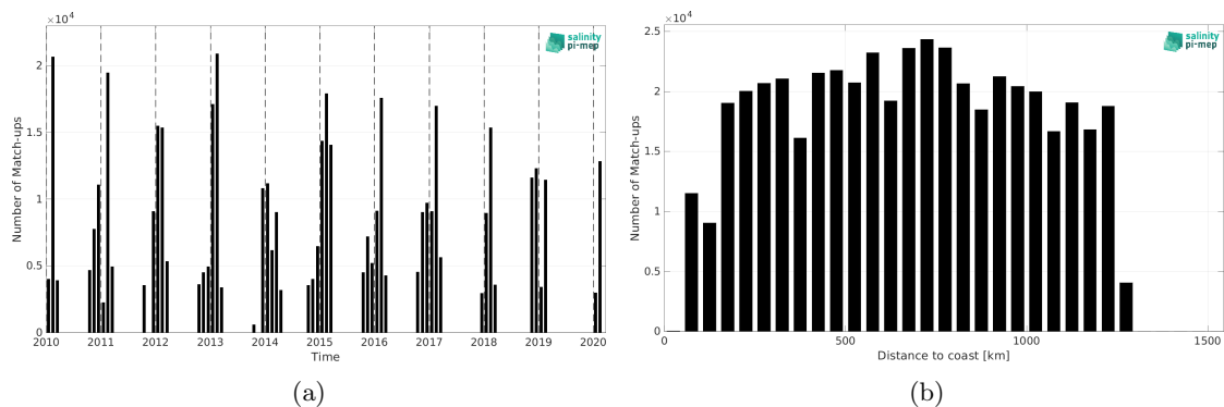
Figure 2: Number of match-ups between TSG (LEGOS-Survostral) and CCI SSS L4 Merged-OI v4.41 - 30-day running (ESA) SSS as a function of time (a) and as function of the distance to coast (b) over the Global Ocean Pi-MEP region and for the full satellite product period.
