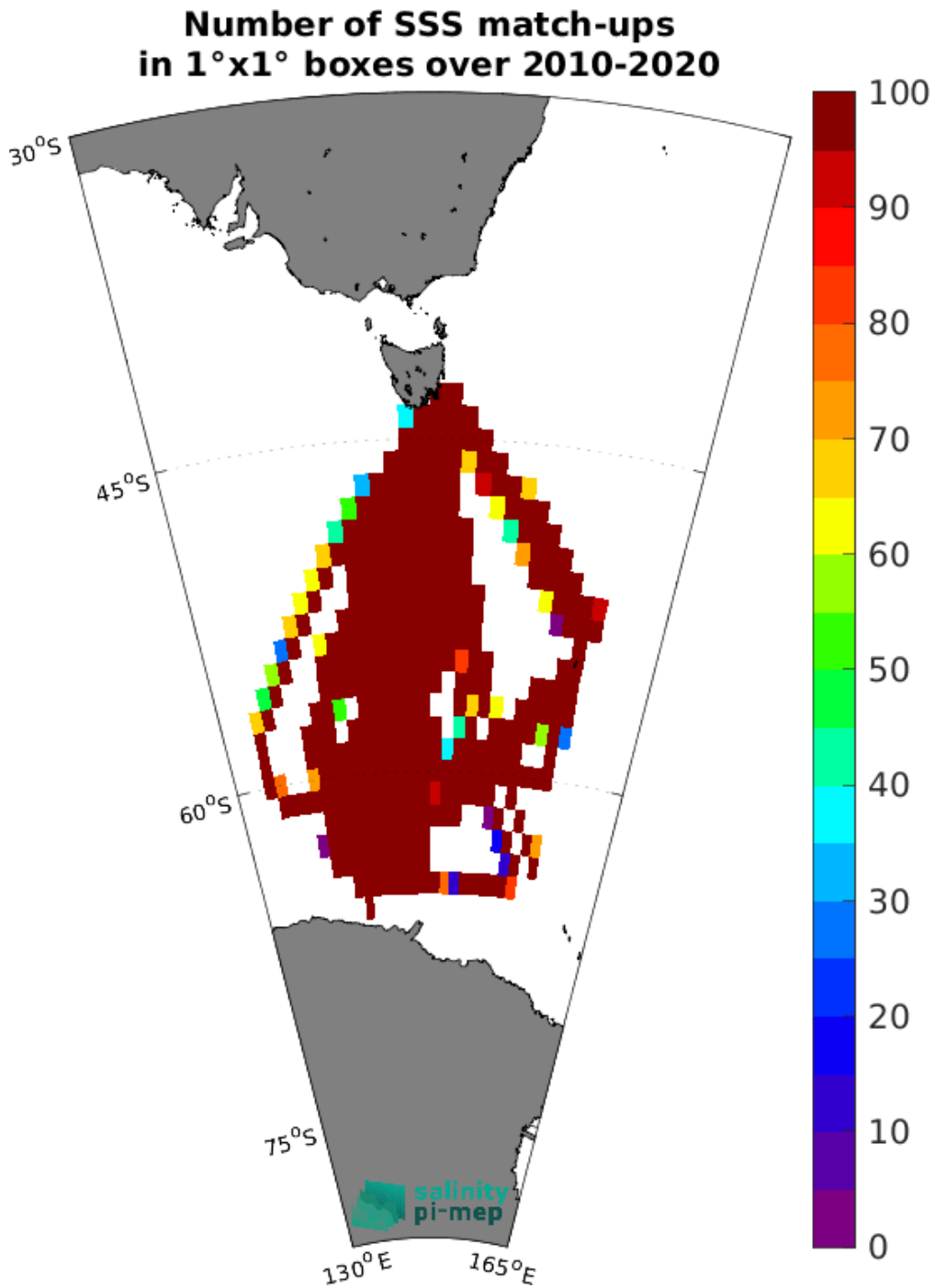
Figure 5: Number of SSS match-ups between TSG (LEGOS-Survostral) SSS and the CCI SSS L4 Merged-OI v4.41 - 30-day running (ESA) SSS product for the Global Ocean Pi-MEP region over 1°x1° boxes and for the full satellite product period.
