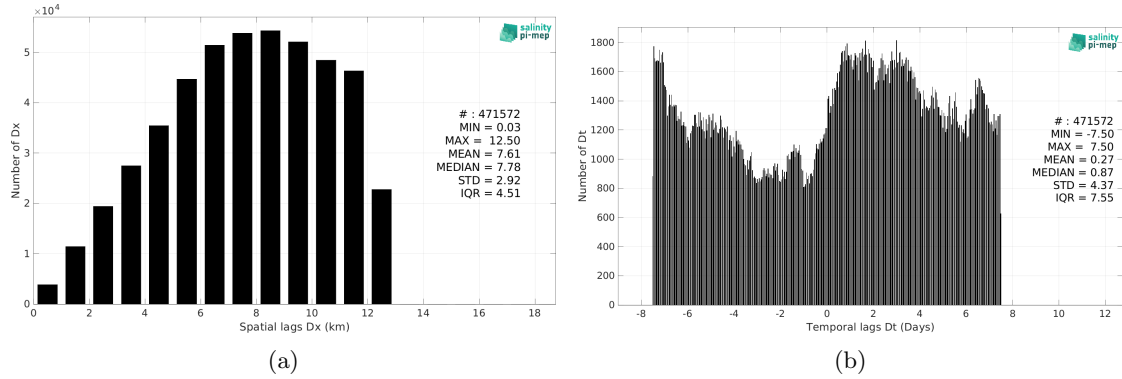
Figure 6: Histograms of the spatial (a) and temporal (b) lags between the location/time of the TSG (LEGOS-Survostral) measurement and the date of the corresponding CCI SSS L4 Merged-OI v4.41 - 30-day running (ESA) SSS pixel.
