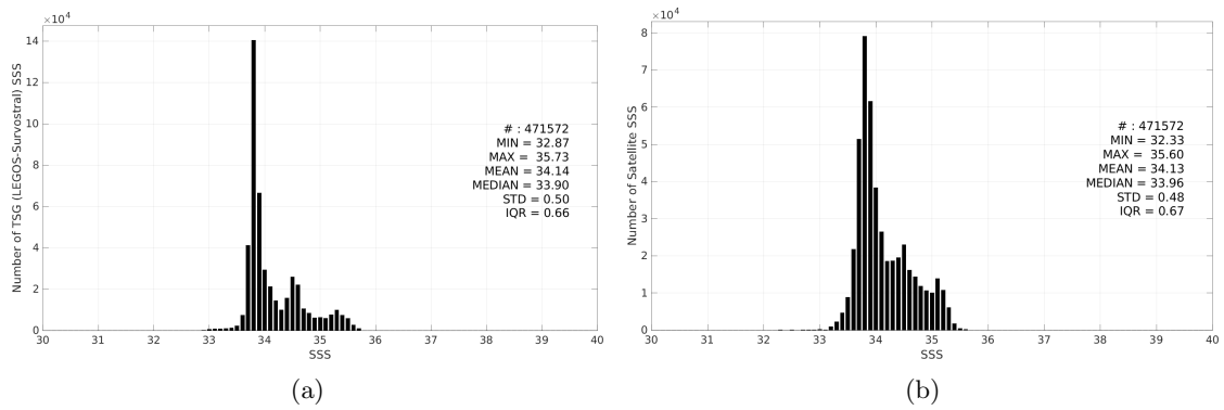
Figure 3: Histograms of SSS from TSG (LEGOS-Survostral) (a) and CCI SSS L4 Merged-OI v4.41 - 30-day running (ESA) (b) considering all match-up pairs per bins of 0.1 over the Global Ocean Pi-MEP region and for the full satellite product period.
