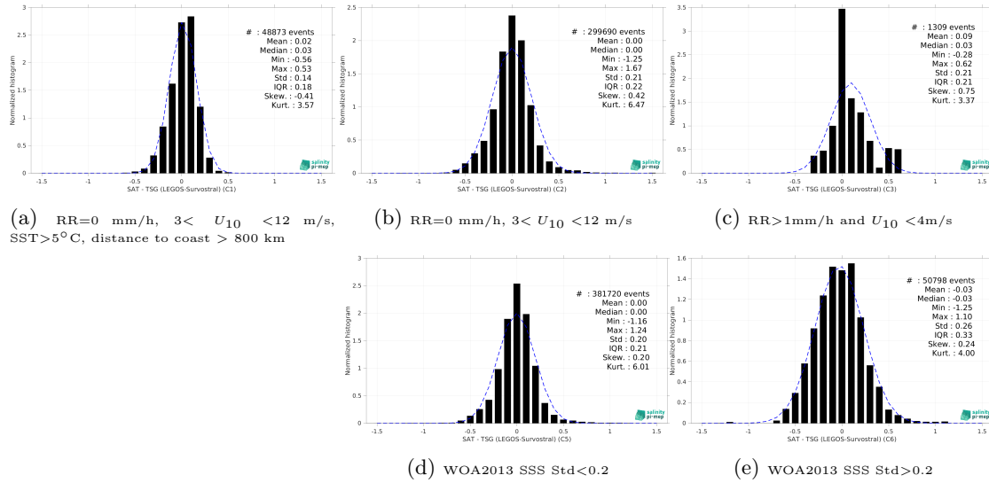
Figure 15: Normalized histogram of \Delta SSS (CCI SSS L4 Merged-OI v4.41 - 30-day running (ESA) - TSG (LEGOS-Survostral)) for 5 different subdatasets corresponding to: RR=0 mm/h, 3 < U_{10} < 12 m/s, SST>5°C, distance to coast > 800 km (a), RR=0 mm/h, 3 < U_{10} < 12 m/s (b), RR>1mm/h and U_{10} < 4 m/s (c), WOA2013 SSS Std<0.2 (d), WOA2013 SSS Std>0.2 (e).
