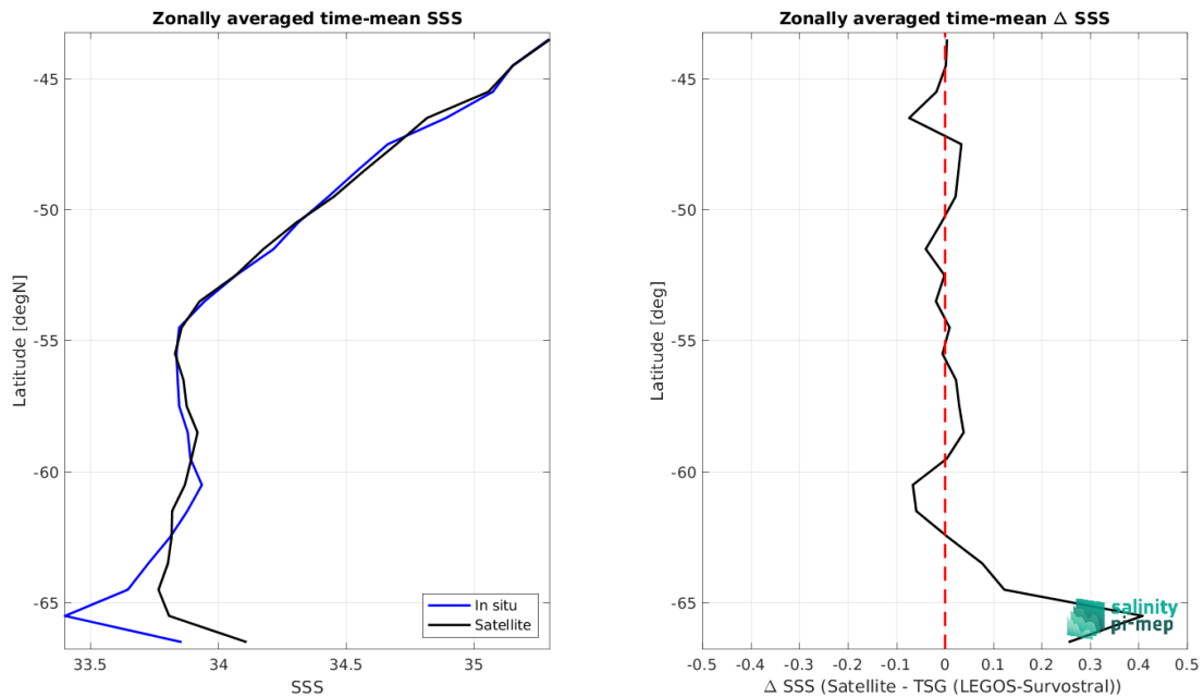
Figure 9: Left panel: Zonal mean SSS from CCI SSS L4 Merged-OI v4.41 - 30-day running (ESA) satellite product (black) and from TSG (LEGOS-Survostral) (blue). Right panel: Zonal mean of \Delta SSS (Satellite - TSG (LEGOS-Survostral)) for all the collected Pi-MEP match-up pairs estimated over the full satellite product period.
