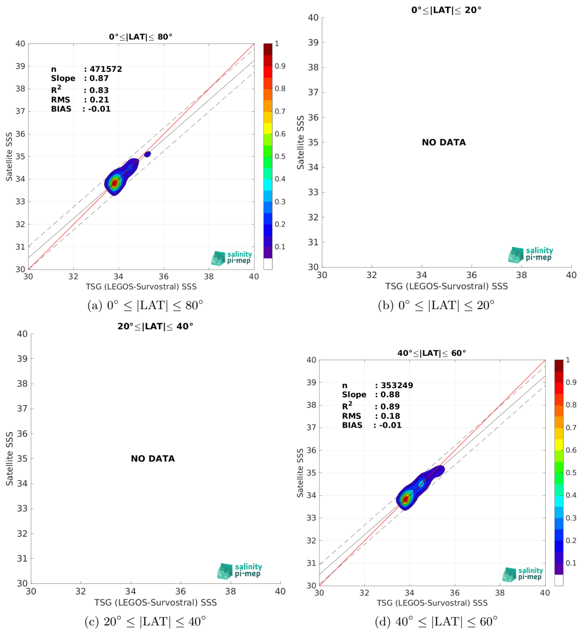
Figure 10: Contour maps of the concentration of CCI SSS L4 Merged-OI v4.41 - 30-day running (ESA) SSS (y-axis) versus TSG (LEGOS-Survostral) SSS (x-axis) at match-up pairs for different latitude bands. For each plot, the red line shows x=y . The black thin and dashed lines indicate a linear fit through the data cloud and the \pm 95\% confidence levels, respectively. The number match-up pairs n , the slope and R^2 coefficient of the linear fit, the root mean square (RMS) and the mean bias between satellite and in situ data are indicated for each latitude band in each plots.
