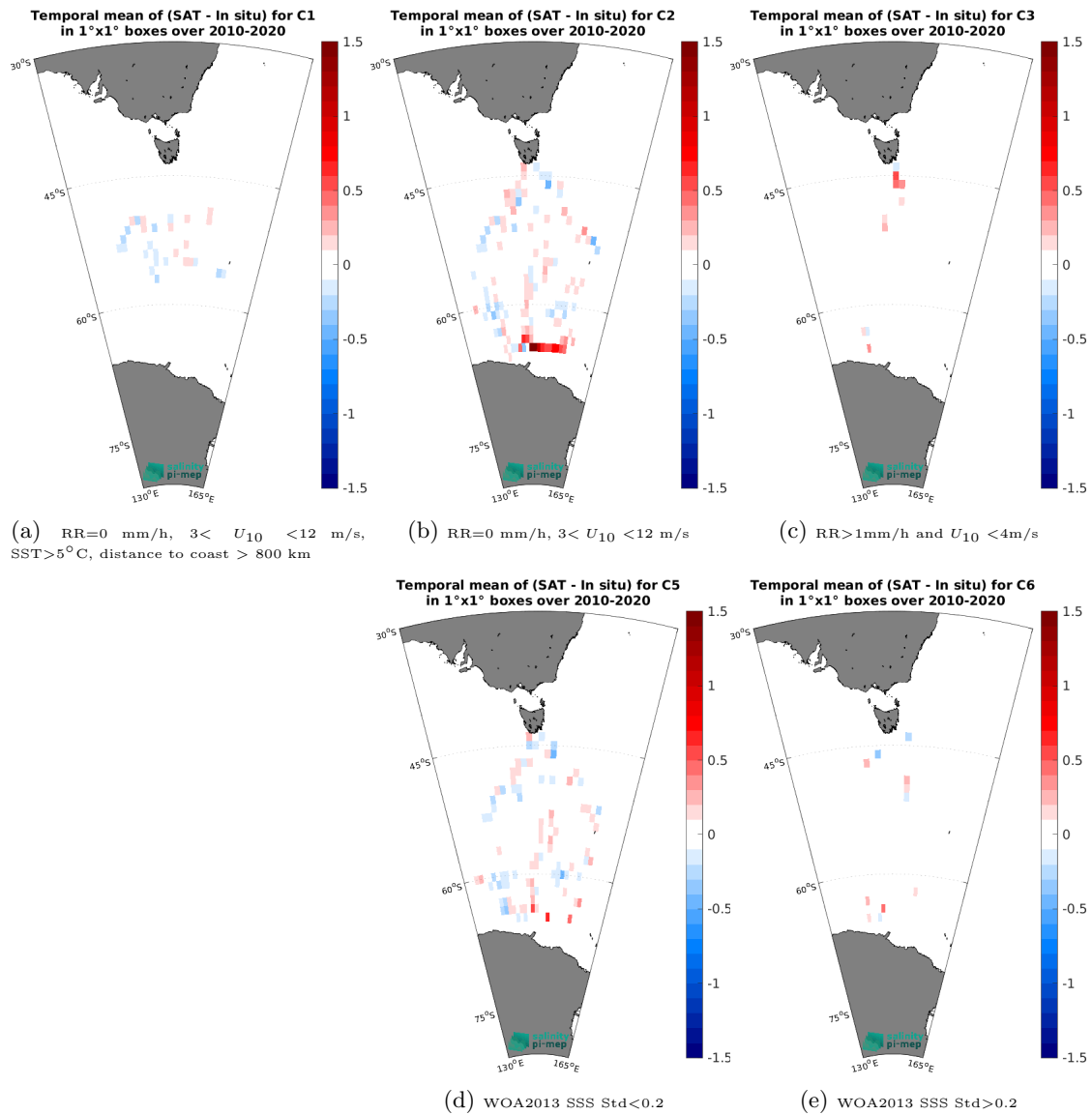
Figure 14: Temporal mean gridded over spatial boxes of size 1^\circ \times 1^\circ of \Delta\text{SSS} (CCI SSS L4 Merged-OI v4.41 - 30-day running (ESA) - TSG (LEGOS-Survostral)) for 5 different subdatasets corresponding to: RR=0 mm/h, 3 < U_{10} < 12 m/s, SST > 5^\circ\text{C} , distance to coast > 800 km (a), RR=0 mm/h, 3 < U_{10} < 12 m/s (b), RR > 1 mm/h and U_{10} < 4 m/s (c), WOA2013 SSS Std < 0.2 (d), WOA2013 SSS Std > 0.2 (e).
