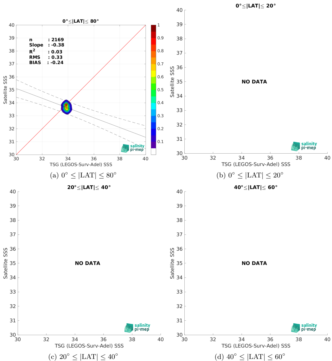
Figure 10: Contour maps of the concentration of CCI SSS L4 Merged-OI v4.41 - 30-day running (ESA) SSS (y-axis) versus TSG (LEGOS-Surv-Adel) SSS (x-axis) at match-up pairs for different latitude bands. For each plot, the red line shows x=y . The black thin and dashed lines indicate a linear fit through the data cloud and the \pm 95\% confidence levels, respectively. The number match-up pairs n , the slope and R^2 coefficient of the linear fit, the root mean square (RMS) and the mean bias between satellite and in situ data are indicated for each latitude band in each plots.
