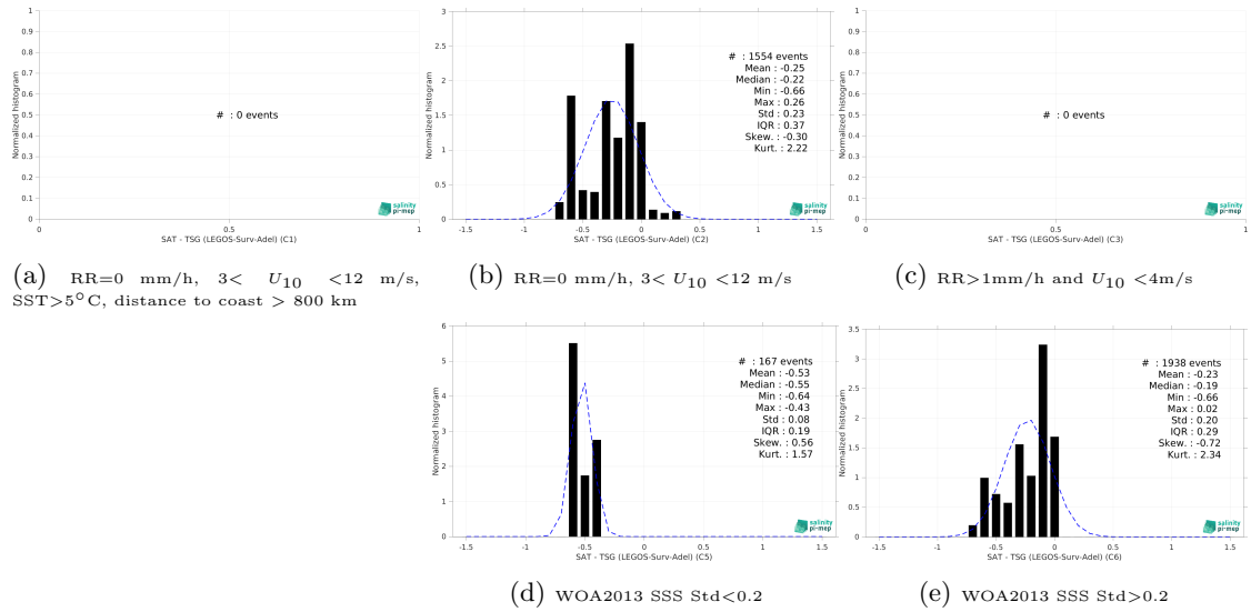
Figure 15: Normalized histogram of \Delta SSS (CCI SSS L4 Merged-OI v4.41 - 30-day running (ESA) - TSG (LEGOS-Surv-Adel)) for 5 different subdatasets corresponding to: RR=0 mm/h, 3 < U_{10} < 12 m/s, SST>5°C, distance to coast > 800 km (a), RR=0 mm/h, 3 < U_{10} < 12 m/s (b), RR>1mm/h and U_{10} < 4 m/s (c), WOA2013 SSS Std<0.2 (d), WOA2013 SSS Std>0.2 (e).
