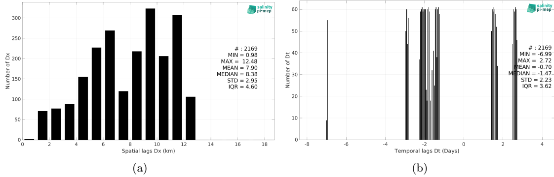
Figure 6: Histograms of the spatial (a) and temporal (b) lags between the location/time of the TSG (LEGOS-Surv-Adel) measurement and the date of the corresponding CCI SSS L4 Merged-OI v4.41 - 30-day running (ESA) SSS pixel.
