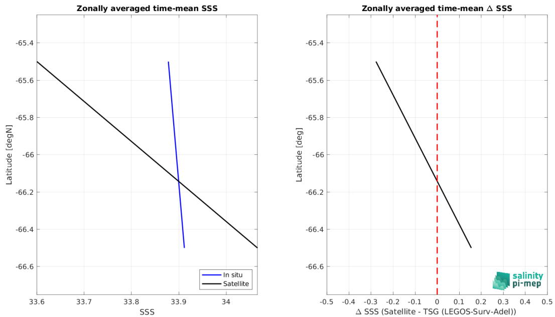
Figure 9: Left panel: Zonal mean SSS from CCI SSS L4 Merged-OI v4.41 - 30-day running (ESA) satellite product (black) and from TSG (LEGOS-Surv-Adel) (blue). Right panel: Zonal mean of \Delta SSS (Satellite - TSG (LEGOS-Surv-Adel)) for all the collected Pi-MEP match-up pairs estimated over the full satellite product period.
