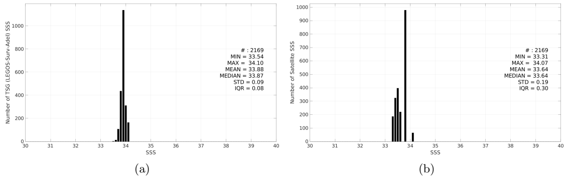
Figure 3: Histograms of SSS from TSG (LEGOS-Surv-Adel) (a) and CCI SSS L4 Merged-OI v4.41 - 30-day running (ESA) (b) considering all match-up pairs per bins of 0.1 over the Global Ocean Pi-MEP region and for the full satellite product period.
