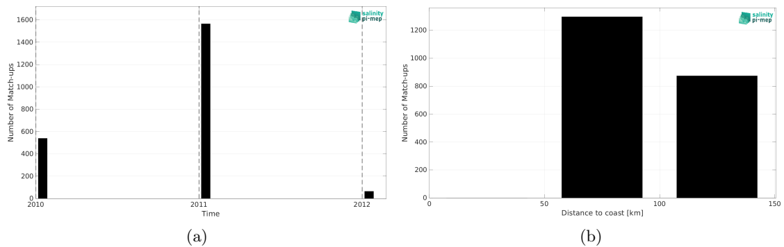
Figure 2: Number of match-ups between TSG (LEGOS-Surv-Adel) and CCI SSS L4 Merged-OI v4.41 - 30-day running (ESA) SSS as a function of time (a) and as function of the distance to coast (b) over the Global Ocean Pi-MEP region and for the full satellite product period.
