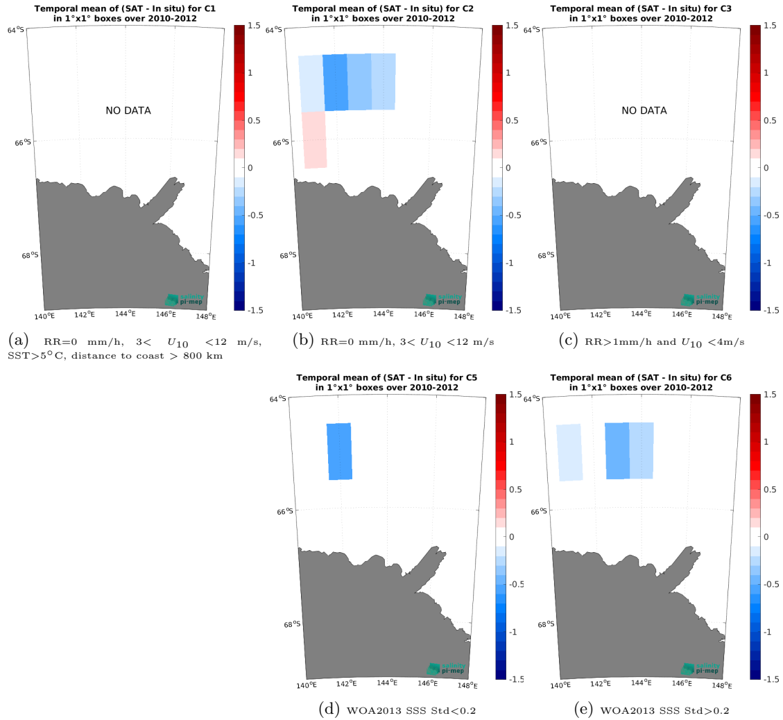
Figure 14: Temporal mean gridded over spatial boxes of size 1^\circ \times 1^\circ of \Delta SSS (CCI SSS L4 Merged-OI v4.41 - 30-day running (ESA) - TSG (LEGOS-Surv-Adel)) for 5 different subdatasets corresponding to: RR=0 mm/h, 3 < U_{10} < 12 m/s, SST>5°C, distance to coast > 800 km (a), RR=0 mm/h, 3 < U_{10} < 12 m/s (b), RR>1mm/h and U_{10} < 4 m/s (c), WOA2013 SSS Std<0.2 (d), WOA2013 SSS Std>0.2 (e).
