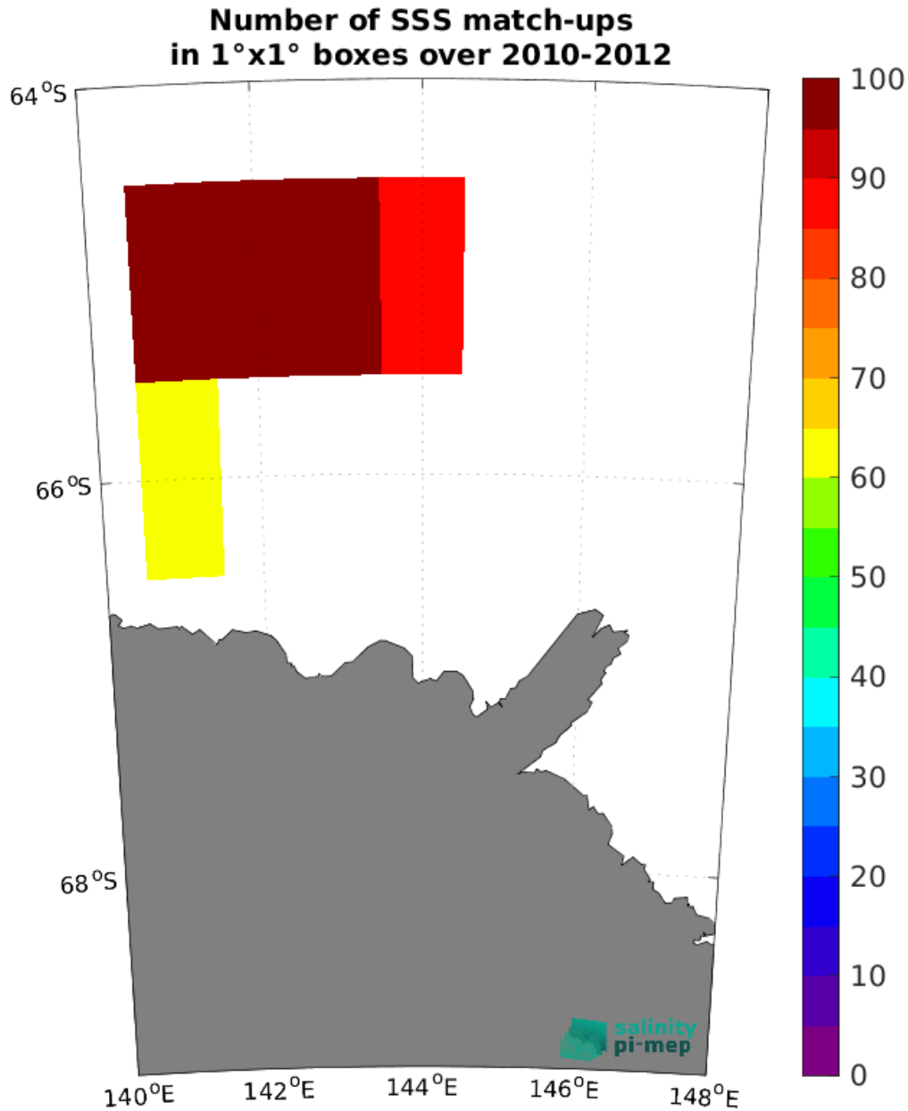
Figure 5: Number of SSS match-ups between TSG (LEGOS-Surv-Adel) SSS and the CCI SSS L4 Merged-OI v4.41 - 30-day running (ESA) SSS product for the Global Ocean Pi-MEP region over 1^\circ \times 1^\circ boxes and for the full satellite product period.
