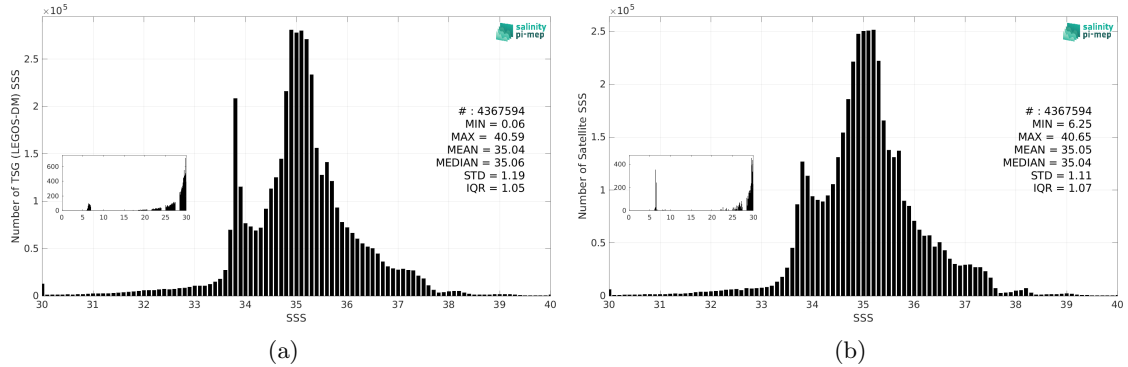
Figure 3: Histograms of SSS from TSG (LEGOS-DM) (a) and CCI SSS L4 Merged-OI v4.41 - 30-day running (ESA) (b) considering all match-up pairs per bins of 0.1 over the Global Ocean Pi-MEP region and for the full satellite product period.
