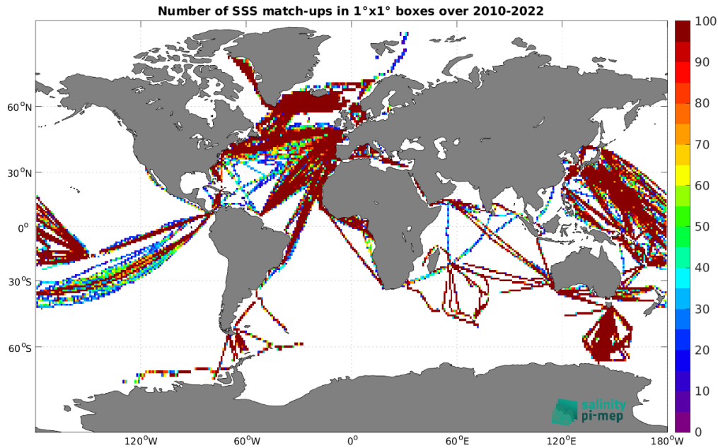
Figure 5: Number of SSS match-ups between TSG (LEGOS-DM) SSS and the CCI SSS L4 Merged-OI v4.41 - 30-day running (ESA) SSS product for the Global Ocean Pi-MEP region over 1^\circ \times 1^\circ boxes and for the full satellite product period.
