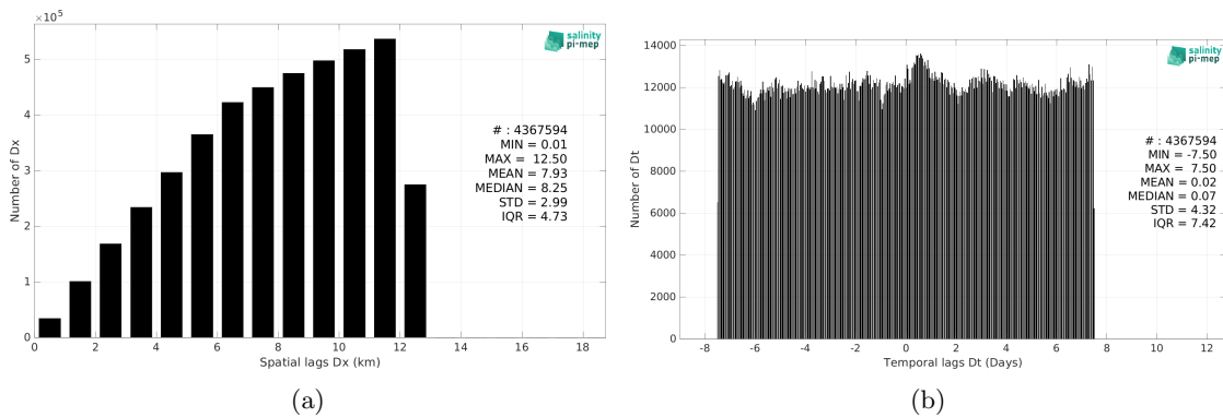
Figure 6: Histograms of the spatial (a) and temporal (b) lags between the location/time of the TSG (LEGOS-DM) measurement and the date of the corresponding CCI SSS L4 Merged-OI v4.41 - 30-day running (ESA) SSS pixel.
