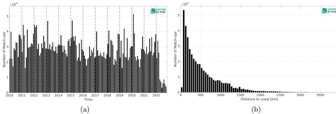
Figure 2: Number of match-ups between TSG (LEGOS-DM) and CCI SSS L4 Merged-OI v4.41 - 30-day running (ESA) SSS as a function of time (a) and as function of the distance to coast (b) over the Global Ocean Pi-MEP region and for the full satellite product period.
