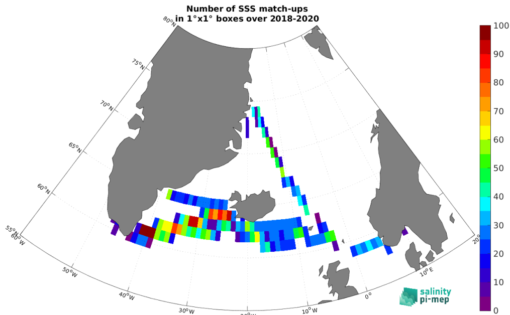
Figure 5: Number of SSS match-ups between TSG (Lauge-Koch) SSS and the CCI SSS L4 Merged-OI v4.41 - 30-day running (ESA) SSS product for the Global Ocean Pi-MEP region over 1^\circ \times 1^\circ boxes and for the full satellite product period.
