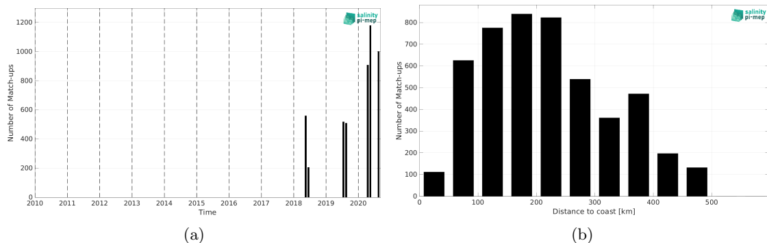
Figure 2: Number of match-ups between TSG (Lauge-Koch) and CCI SSS L4 Merged-OI v4.41 - 30-day running (ESA) SSS as a function of time (a) and as function of the distance to coast (b) over the Global Ocean Pi-MEP region and for the full satellite product period.
