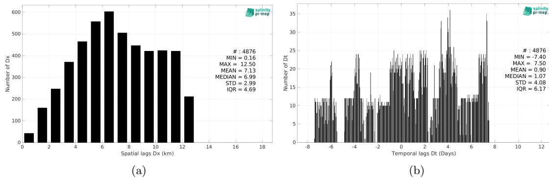
Figure 6: Histograms of the spatial (a) and temporal (b) lags between the location/time of the TSG (Lauge-Koch) measurement and the date of the corresponding CCI SSS L4 Merged-OI v4.41 - 30-day running (ESA) SSS pixel.
