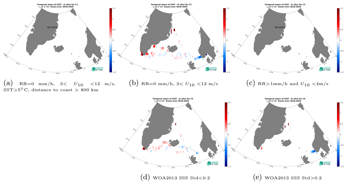
Figure 14: Temporal mean gridded over spatial boxes of size 1^\circ \times 1^\circ of \Delta\text{SSS} (CCI SSS L4 Merged-OI v4.41 - 30-day running (ESA) - TSG (Lauge-Koch)) for 5 different subdatasets corresponding to:RR=0 mm/h, 3 < U_{10} < 12 m/s, SST > 5^\circ\text{C} , distance to coast > 800 km (a), RR=0 mm/h, 3 < U_{10} < 12 m/s (b), RR > 1 mm/h and U_{10} < 4 m/s (c), WOA2013 SSS Std < 0.2 (d), WOA2013 SSS Std > 0.2 (e).
