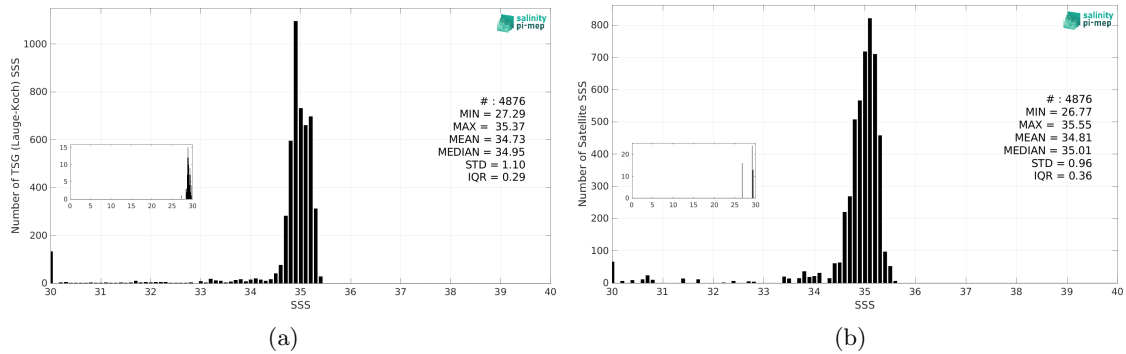
Figure 3: Histograms of SSS from TSG (Lauge-Koch) (a) and CCI SSS L4 Merged-OI v4.41 - 30-day running (ESA) (b) considering all match-up pairs per bins of 0.1 over the Global Ocean Pi-MEP region and for the full satellite product period.
