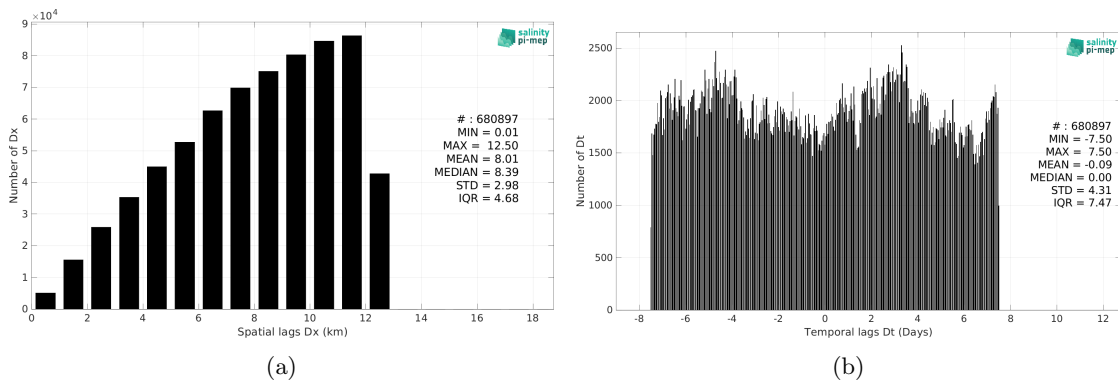
Figure 6: Histograms of the spatial (a) and temporal (b) lags between the location/time of the TSG (GOSUD-Sailing-ship) measurement and the date of the corresponding CCI SSS L4 Merged-OI v4.41 - 30-day running (ESA) SSS pixel.
