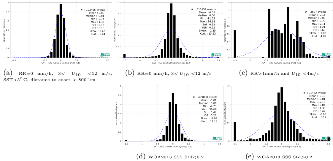
Figure 15: Normalized histogram of \Delta SSS (CCI SSS L4 Merged-OI v4.41 - 30-day running (ESA) - TSG (GOSUD-Sailing-ship)) for 5 different subdatasets corresponding to: RR=0 mm/h, 3 < U_{10} < 12 m/s, SST>5°C, distance to coast > 800 km (a), RR=0 mm/h, 3 < U_{10} < 12 m/s (b), RR>1mm/h and U_{10} < 4 m/s (c), WOA2013 SSS Std<0.2 (d), WOA2013 SSS Std>0.2 (e).
