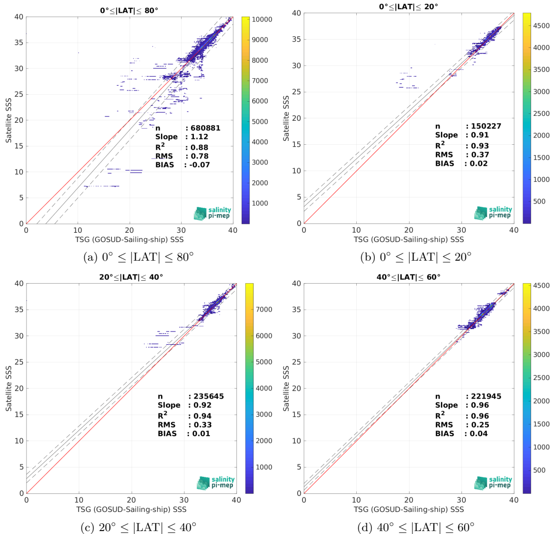
Figure 10: Contour maps of the concentration of CCI SSS L4 Merged-OI v4.41 - 30-day running (ESA) SSS (y-axis) versus TSG (GOSUD-Sailing-ship) SSS (x-axis) at match-up pairs for different latitude bands. For each plot, the red line shows x=y . The black thin and dashed lines indicate a linear fit through the data cloud and the \pm 95\% confidence levels, respectively. The number of match-up pairs n , the slope and R^2 coefficient of the linear fit, the root mean square (RMS) and the mean bias between satellite and in situ data are indicated for each latitude band in each plot.
