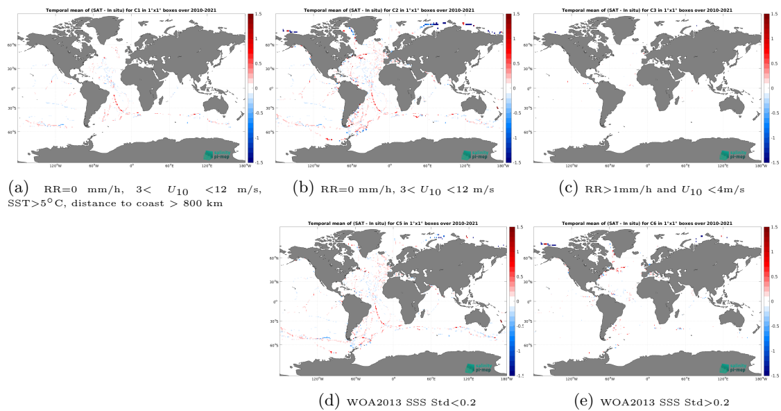
Figure 14: Temporal mean gridded over spatial boxes of size 1^\circ \times 1^\circ of \Delta SSS (CCI SSS L4 Merged-OI v4.41 - 30-day running (ESA) - TSG (GOSUD-Sailing-ship)) for 5 different subdatasets corresponding to: RR=0 mm/h, 3 < U_{10} < 12 m/s, SST > 5^\circ\text{C} , distance to coast > 800 km (a), RR=0 mm/h, 3 < U_{10} < 12 m/s (b), RR > 1 mm/h and U_{10} < 4 m/s (c), WOA2013 SSS Std < 0.2 (d), WOA2013 SSS Std > 0.2 (e).
