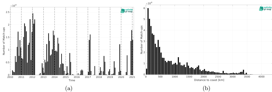
Figure 2: Number of match-ups between TSG (GOSUD-Sailing-ship) and CCI SSS L4 Merged-OI v4.41 - 30-day running (ESA) SSS as a function of time (a) and as function of the distance to coast (b) over the Global Ocean Pi-MEP region and for the full satellite product period.
