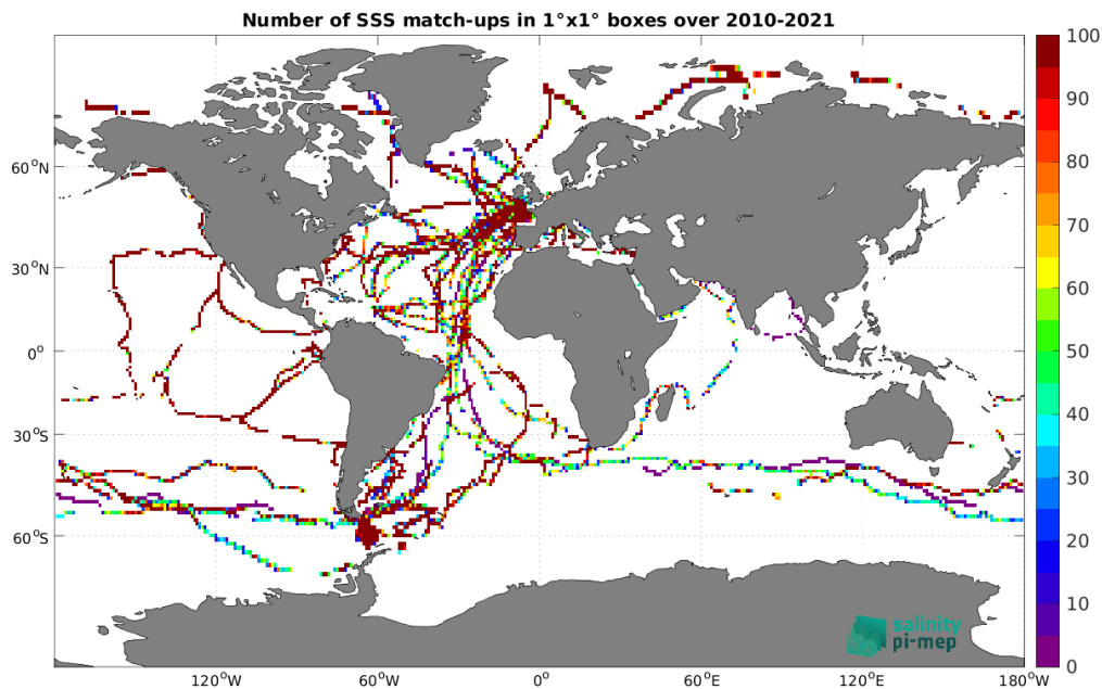
Figure 5: Number of SSS match-ups between TSG (GOSUD-Sailing-ship) SSS and the CCI SSS L4 Merged-OI v4.41 - 30-day running (ESA) SSS product for the Global Ocean Pi-MEP region over 1^\circ \times 1^\circ boxes and for the full satellite product period.
