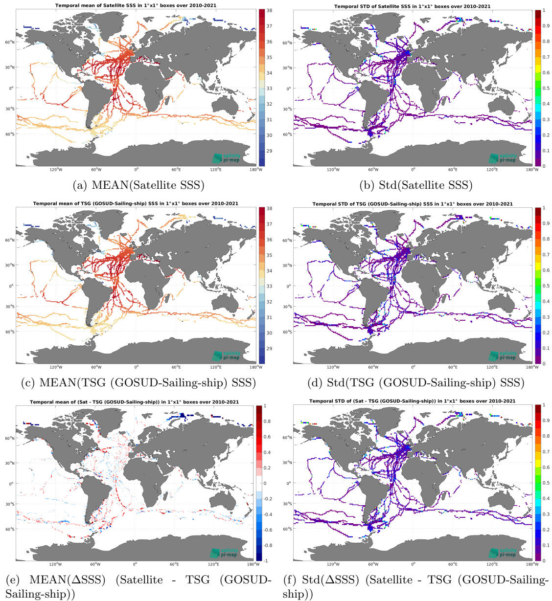
Figure 7: Temporal mean (left) and Std (right) of SSS from CCI SSS L4 Merged-OI v4.41 - 30-day running (ESA) (top), TSG (GOSUD-Sailing-ship) (middle), and of \Delta SSS (Satellite - TSG (GOSUD-Sailing-ship)). Only match-up pairs are used to generate these maps.
