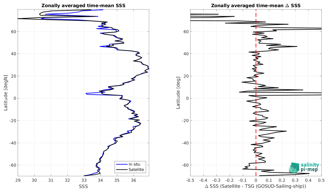
Figure 9: Left panel: Zonal mean SSS from CCI SSS L4 Merged-OI v4.41 - 30-day running (ESA) satellite product (black) and from TSG (GOSUD-Sailing-ship) (blue). Right panel: Zonal mean of \Delta SSS (Satellite - TSG (GOSUD-Sailing-ship)) for all the collected Pi-MEP match-up pairs estimated over the full satellite product period.
