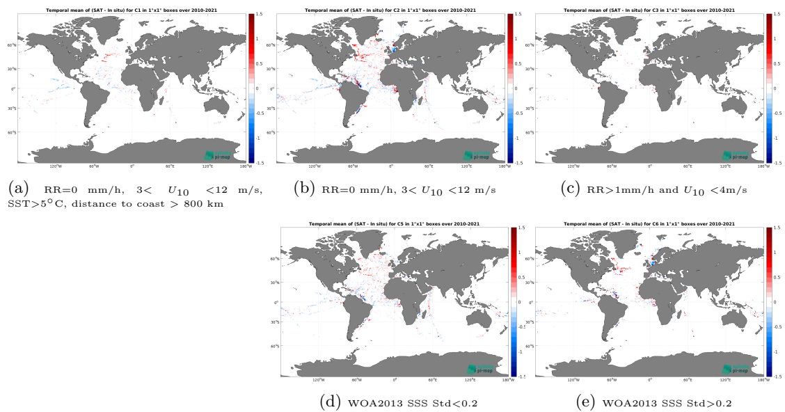
Figure 14: Temporal mean gridded over spatial boxes of size 1^\circ \times 1^\circ of \Delta\text{SSS} (CCI SSS L4 Merged-OI v4.41 - 30-day running (ESA) - TSG (GOSUD-Research-vessel)) for 5 different subdatasets corresponding to:RR=0 mm/h, 3 < U_{10} < 12 m/s, SST > 5^\circ\text{C} , distance to coast > 800 km (a), RR=0 mm/h, 3 < U_{10} < 12 m/s (b), RR > 1 mm/h and U_{10} < 4 m/s (c), WOA2013 SSS Std < 0.2 (d), WOA2013 SSS Std > 0.2 (e).
