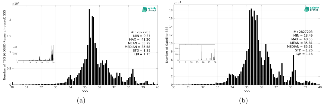
Figure 3: Histograms of SSS from TSG (GOSUD-Research-vessel) (a) and CCI SSS L4 Merged-OI v4.41 - 30-day running (ESA) (b) considering all match-up pairs per bins of 0.1 over the Global Ocean Pi-MEP region and for the full satellite product period.
