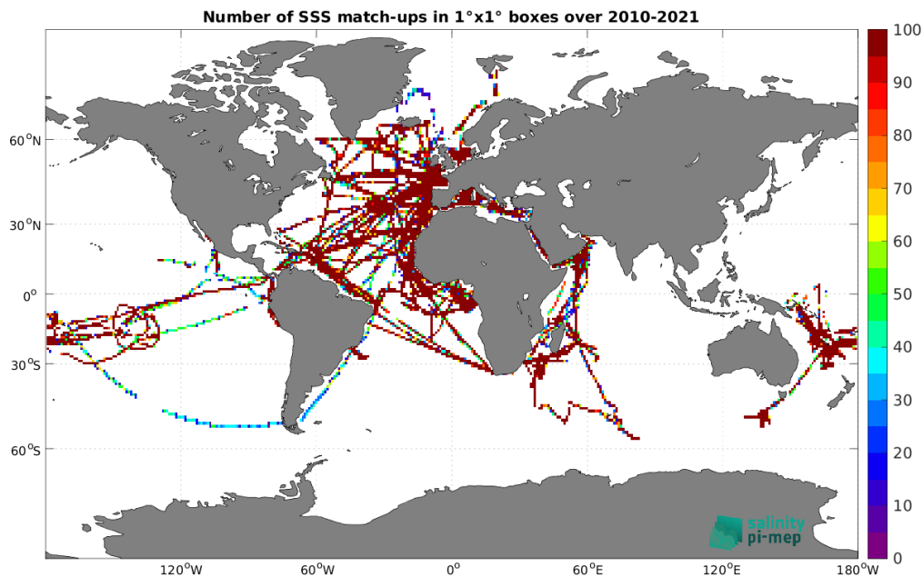
Figure 5: Number of SSS match-ups between TSG (GOSUD-Research-vessel) SSS and the CCI SSS L4 Merged-OI v4.41 - 30-day running (ESA) SSS product for the Global Ocean Pi-MEP region over 1^\circ \times 1^\circ boxes and for the full satellite product period.
