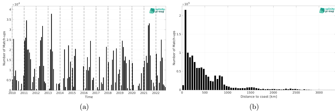
Figure 2: Number of match-ups between TSG (CSIC-UTM) and CCI SSS L4 Merged-OI v4.41 - 30-day running (ESA) SSS as a function of time (a) and as function of the distance to coast (b) over the Global Ocean Pi-MEP region and for the full satellite product period.
