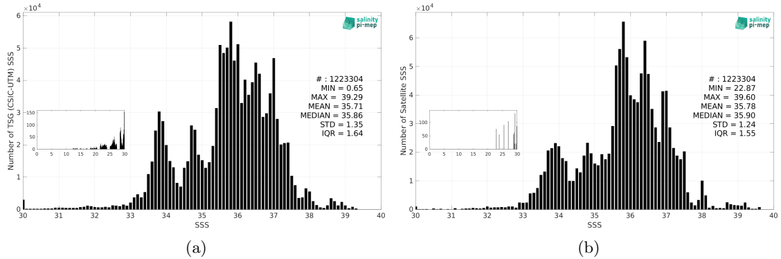
Figure 3: Histograms of SSS from TSG (CSIC-UTM) (a) and CCI SSS L4 Merged-OI v4.41 - 30-day running (ESA) (b) considering all match-up pairs per bins of 0.1 over the Global Ocean Pi-MEP region and for the full satellite product period.
