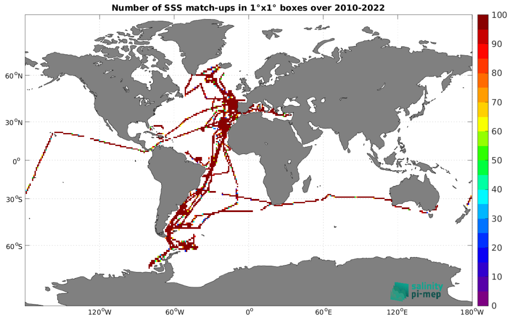
Figure 5: Number of SSS match-ups between TSG (CSIC-UTM) SSS and the CCI SSS L4 Merged-OI v4.41 - 30-day running (ESA) SSS product for the Global Ocean Pi-MEP region over 1^\circ \times 1^\circ boxes and for the full satellite product period.
