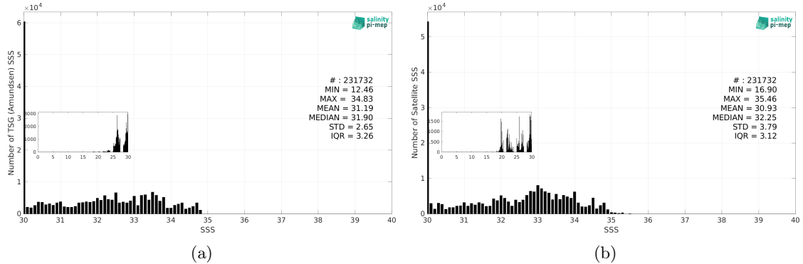
Figure 3: Histograms of SSS from TSG (Amundsen) (a) and CCI SSS L4 Merged-OI v4.41 - 30-day running (ESA) (b) considering all match-up pairs per bins of 0.1 over the Global Ocean Pi-MEP region and for the full satellite product period.
