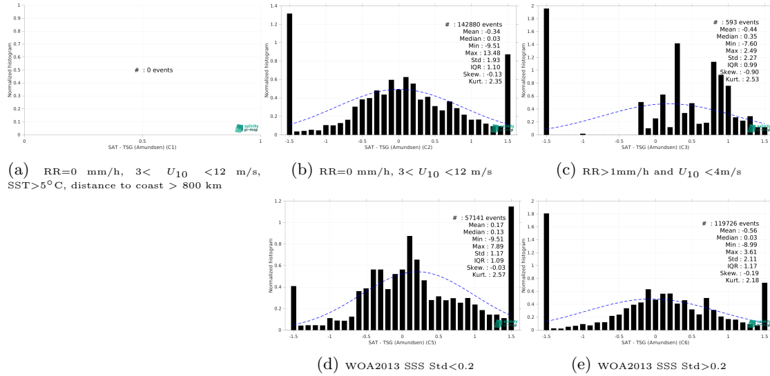
Figure 15: Normalized histogram of \Delta SSS (CCI SSS L4 Merged-OI v4.41 - 30-day running (ESA) - TSG (Amundsen)) for 5 different subdatasets corresponding to: RR=0 mm/h, 3 < U_{10} < 12 m/s, SST > 5°C, distance to coast > 800 km (a), RR=0 mm/h, 3 < U_{10} < 12 m/s (b), RR > 1mm/h and U_{10} < 4 m/s (c), WOA2013 SSS Std < 0.2 (d), WOA2013 SSS Std > 0.2 (e).
