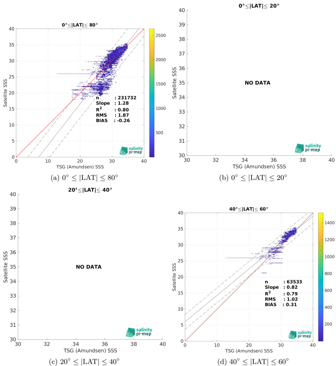
Figure 10: Contour maps of the concentration of CCI SSS L4 Merged-OI v4.41 - 30-day running (ESA) SSS (y-axis) versus TSG (Amundsen) SSS (x-axis) at match-up pairs for different latitude bands. For each plot, the red line shows x=y . The black thin and dashed lines indicate a linear fit through the data cloud and the \pm 95\% confidence levels, respectively. The number match-up pairs n , the slope and R^2 coefficient of the linear fit, the root mean square (RMS) and the mean bias between satellite and in situ data are indicated for each latitude band in each plots.
