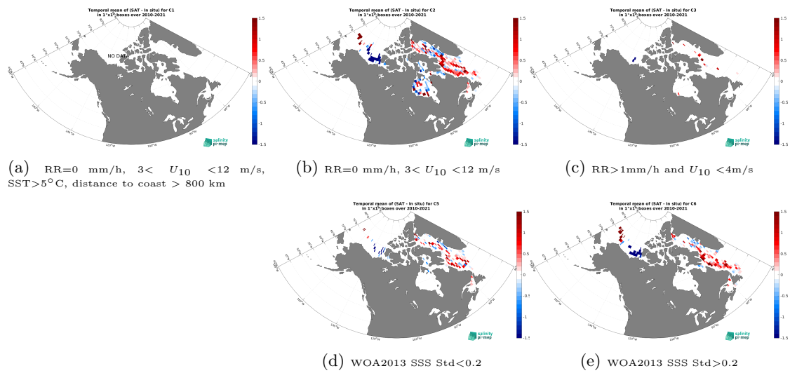
Figure 14: Temporal mean gridded over spatial boxes of size 1^\circ \times 1^\circ of \Delta SSS (CCI SSS L4 Merged-OI v4.41 - 30-day running (ESA) - TSG (Amundsen)) for 5 different subdatasets corresponding to:RR=0 mm/h, 3 < U_{10} < 12 m/s, SST > 5^\circ C, distance to coast > 800 km (a), RR=0 mm/h, 3 < U_{10} < 12 m/s (b), RR > 1 mm/h and U_{10} < 4 m/s (c), WOA2013 SSS Std < 0.2 (d), WOA2013 SSS Std > 0.2 (e).
