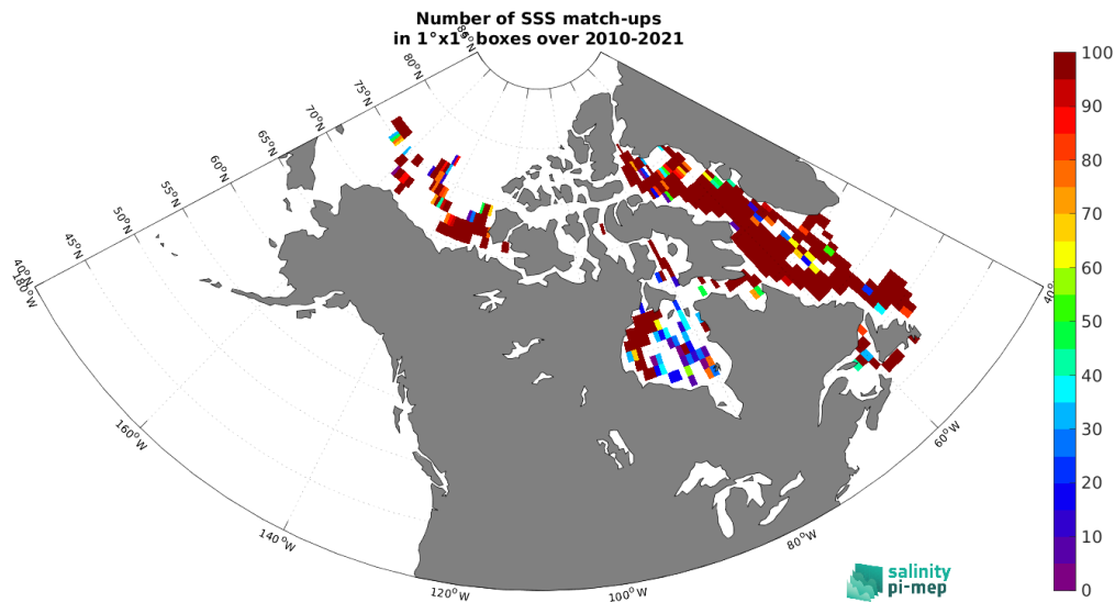
Figure 5: Number of SSS match-ups between TSG (Amundsen) SSS and the CCI SSS L4 Merged-OI v4.41 - 30-day running (ESA) SSS product for the Global Ocean Pi-MEP region over 1^\circ \times 1^\circ boxes and for the full satellite product period.
