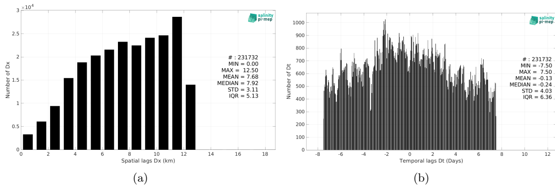
Figure 6: Histograms of the spatial (a) and temporal (b) lags between the location/time of the TSG (Amundsen) measurement and the date of the corresponding CCI SSS L4 Merged-OI v4.41 - 30-day running (ESA) SSS pixel.
