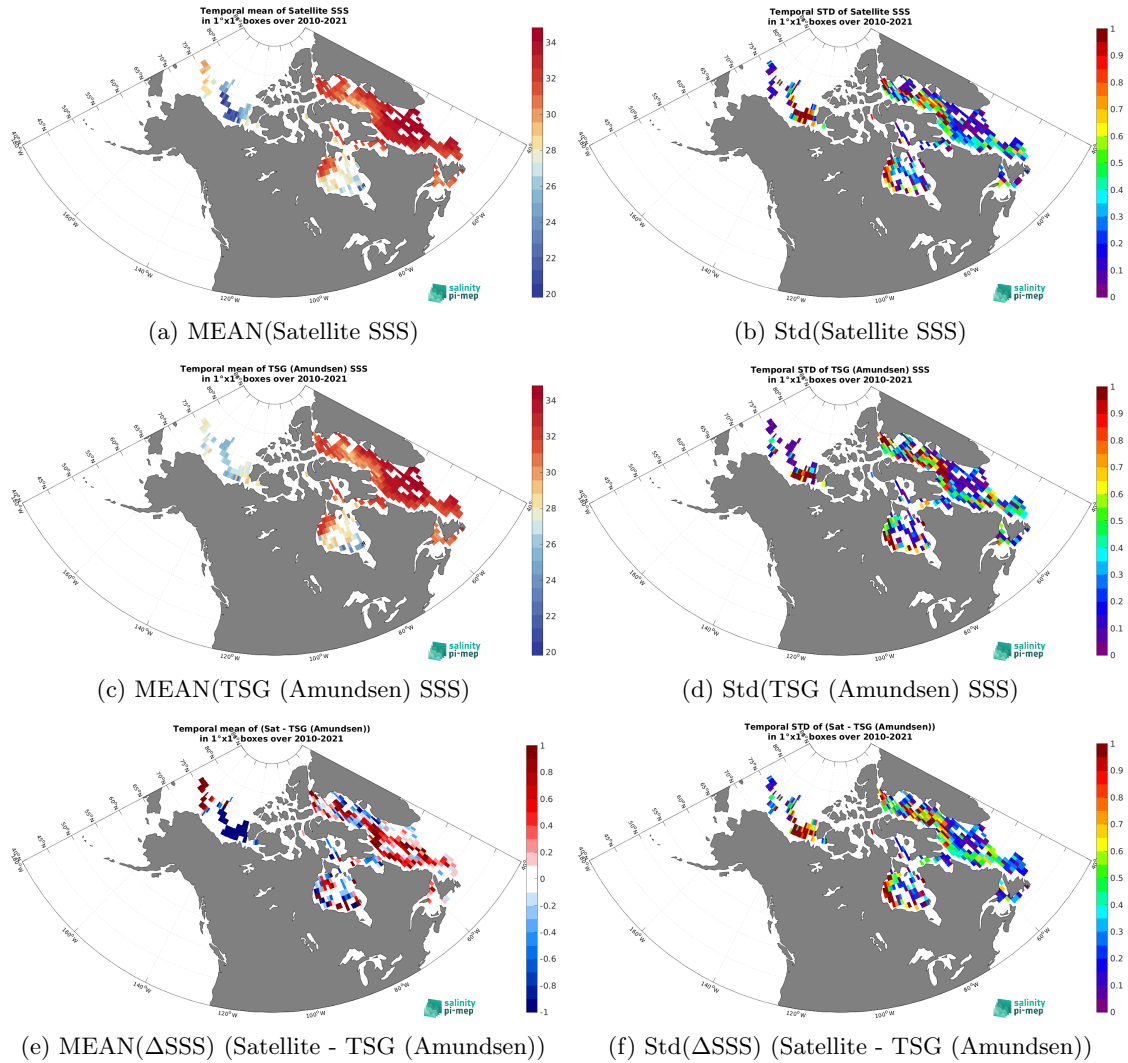
Figure 7: Temporal mean (left) and Std (right) of SSS from CCI SSS L4 Merged-OI v4.41 - 30-day running (ESA) (top), TSG (Amundsen) (middle), and of \Delta SSS (Satellite - TSG (Amundsen)). Only match-up pairs are used to generate these maps.
