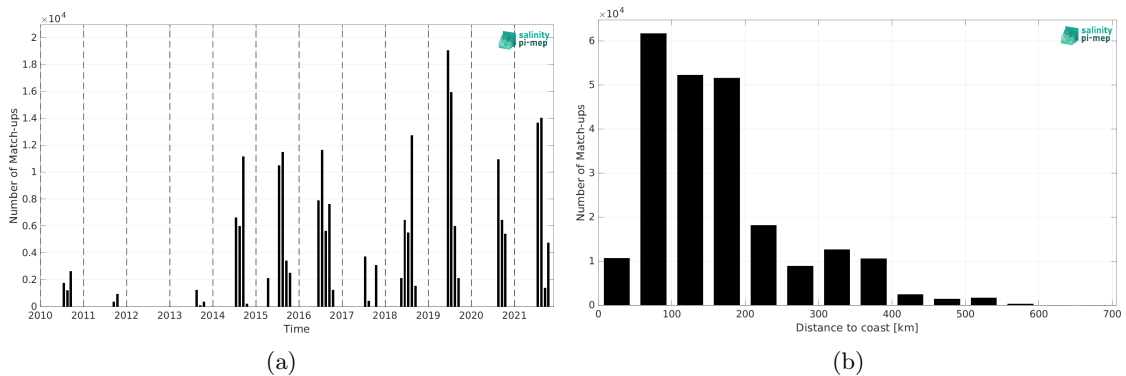
Figure 2: Number of match-ups between TSG (Amundsen) and CCI SSS L4 Merged-OI v4.41 - 30-day running (ESA) SSS as a function of time (a) and as function of the distance to coast (b) over the Global Ocean Pi-MEP region and for the full satellite product period.
