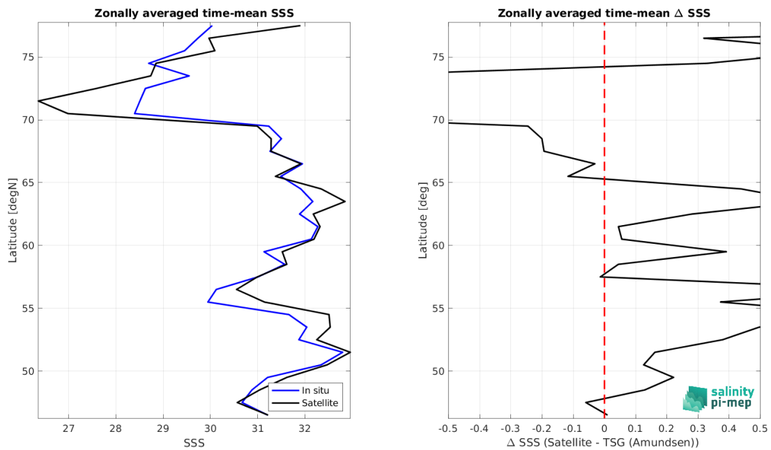
Figure 9: Left panel: Zonal mean SSS from CCI SSS L4 Merged-OI v4.41 - 30-day running (ESA) satellite product (black) and from TSG (Amundsen) (blue). Right panel: Zonal mean of \Delta SSS (Satellite - TSG (Amundsen)) for all the collected Pi-MEP match-up pairs estimated over the full satellite product period.
