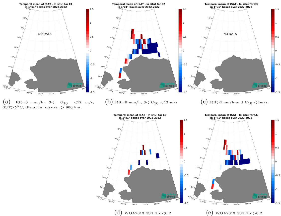
Figure 14: Temporal mean gridded over spatial boxes of size 1^\circ \times 1^\circ of \Delta\text{SSS} (CCI SSS L4 Merged-OI v4.41 - 30-day running (ESA) - SASSIE) for 5 different subdatasets corresponding to:RR=0 mm/h, 3 < U_{10} < 12 m/s, SST>5°C, distance to coast > 800 km (a), RR=0 mm/h, 3 < U_{10} < 12 m/s (b), RR>1mm/h and U_{10} < 4 m/s (c), WOA2013 SSS Std<0.2 (d), WOA2013 SSS Std>0.2 (e).
