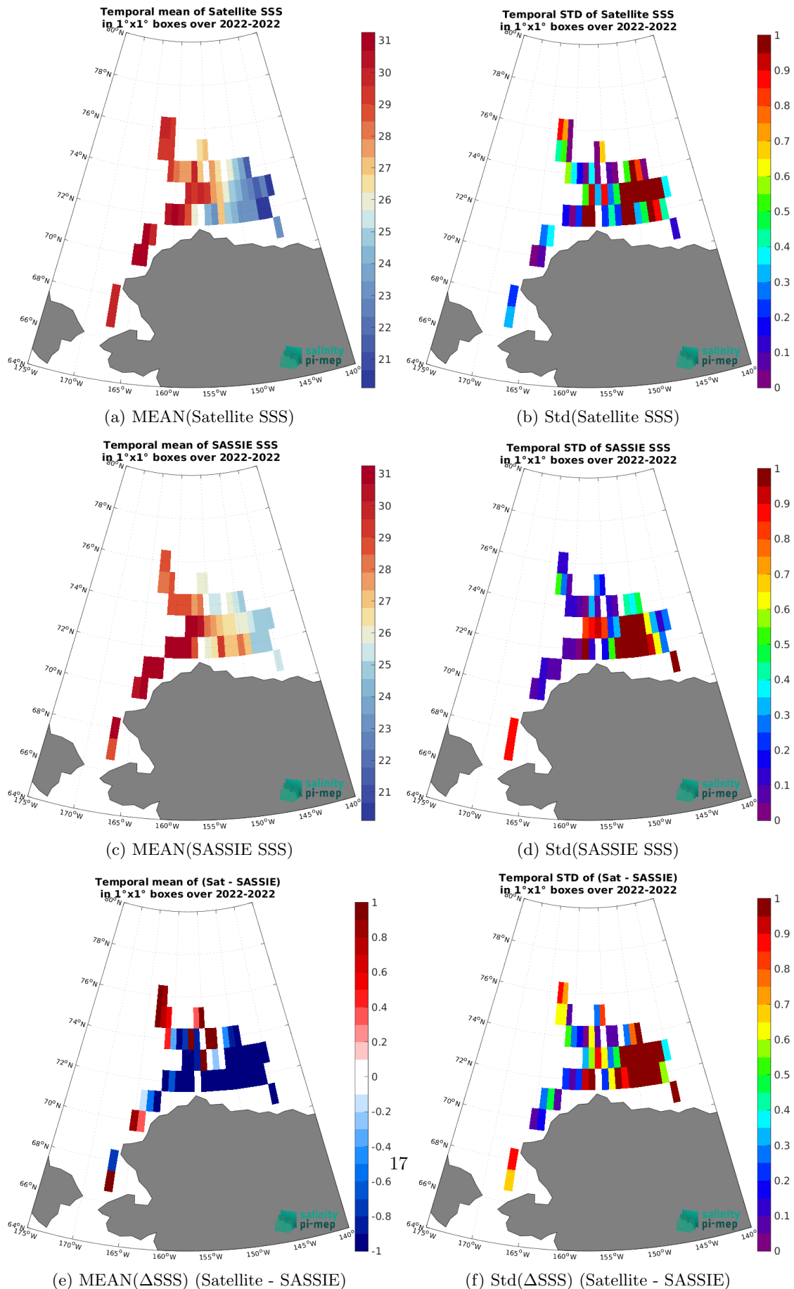
Figure 7: Temporal mean (left) and Std (right) of SSS from CCI SSS L4 Merged-OI v4.41 - 30-day running (ESA) (top), SASSIE (middle), and of \Delta SSS (Satellite - SASSIE). Only match-up pairs are used to generate these maps.
