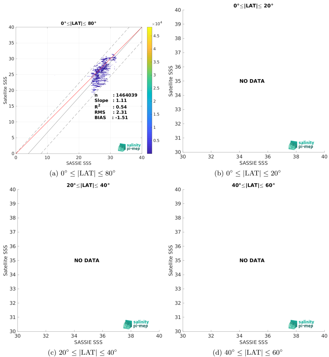
Figure 10: Contour maps of the concentration of CCI SSS L4 Merged-OI v4.41 - 30-day running (ESA) SSS (y-axis) versus SASSIE SSS (x-axis) at match-up pairs for different latitude bands. For each plot, the red line shows x=y . The black thin and dashed lines indicate a linear fit through the data cloud and the \pm 95\% confidence levels, respectively. The number match-up pairs n , the slope and R^2 coefficient of the linear fit, the root mean square (RMS) and the mean bias between satellite and in situ data are indicated for each latitude band in each plots.
