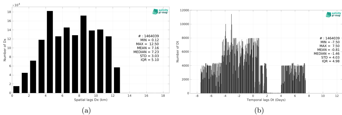
Figure 6: Histograms of the spatial (a) and temporal (b) lags between the location/time of the SASSIE measurement and the date of the corresponding CCI SSS L4 Merged-OI v4.41 - 30-day running (ESA) SSS pixel.
