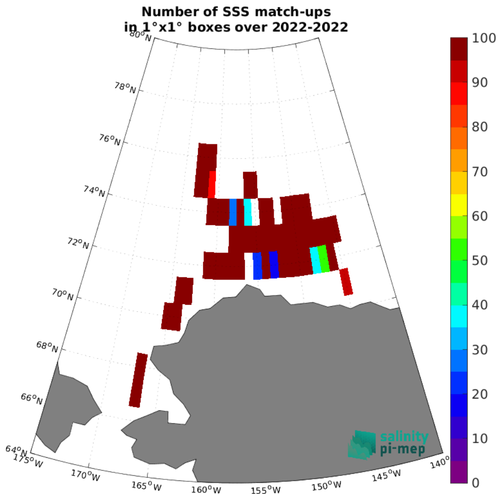
Figure 5: Number of SSS match-ups between SASSIE SSS and the CCI SSS L4 Merged-OI v4.41 - 30-day running (ESA) SSS product for the Global Ocean Pi-MEP region over 1^\circ \times 1^\circ boxes and for the full satellite product period.
