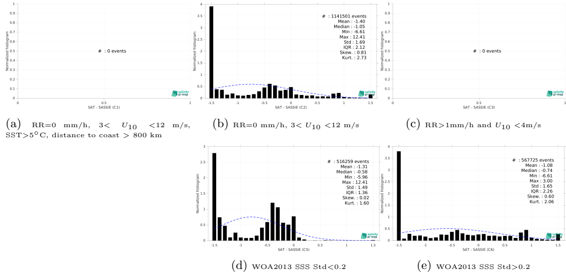
Figure 15: Normalized histogram of \Delta SSS (CCI SSS L4 Merged-OI v4.41 - 30-day running (ESA) - SASSIE) for 5 different subdatasets corresponding to: RR=0 mm/h, 3 < U_{10} < 12 m/s, SST > 5°C, distance to coast > 800 km (a), RR=0 mm/h, 3 < U_{10} < 12 m/s (b), RR > 1mm/h and U_{10} < 4 m/s (c), WOA2013 SSS Std < 0.2 (d), WOA2013 SSS Std > 0.2 (e).
