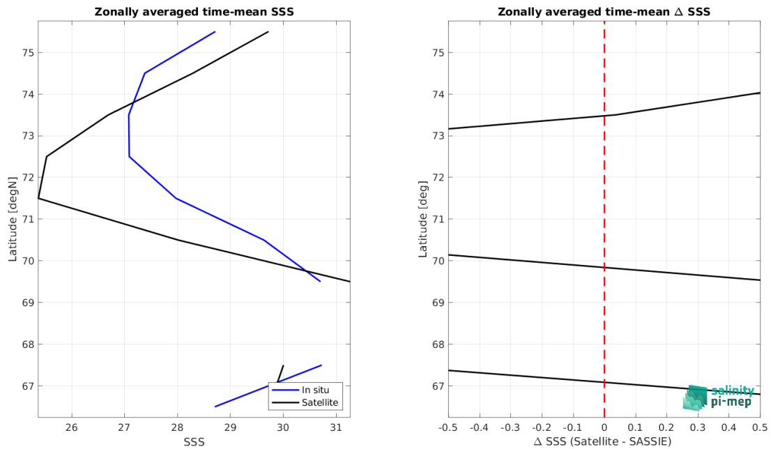
Figure 9: Left panel: Zonal mean SSS from CCI SSS L4 Merged-OI v4.41 - 30-day running (ESA) satellite product (black) and from SASSIE (blue). Right panel: Zonal mean of \Delta SSS (Satellite - SASSIE) for all the collected Pi-MEP match-up pairs estimated over the full satellite product period.
