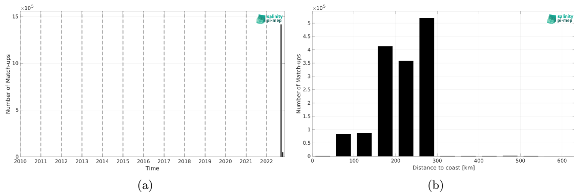
Figure 2: Number of match-ups between SASSIE and CCI SSS L4 Merged-OI v4.41 - 30-day running (ESA) SSS as a function of time (a) and as function of the distance to coast (b) over the Global Ocean Pi-MEP region and for the full satellite product period.
