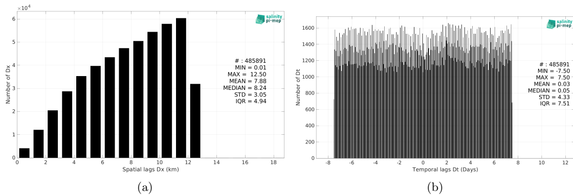
Figure 6: Histograms of the spatial (a) and temporal (b) lags between the location/time of the Saifdrone measurement and the date of the corresponding CCI SSS L4 Merged-OI v4.41 - 30-day running (ESA) SSS pixel.
