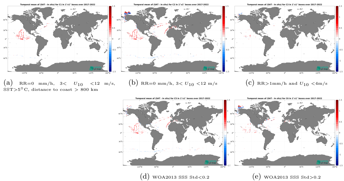
Figure 14: Temporal mean gridded over spatial boxes of size 1^\circ \times 1^\circ of \Delta SSS (CCI SSS L4 Merged-OI v4.41 - 30-day running (ESA) - Saildrone) for 5 different subdatasets corresponding to:RR=0 mm/h, 3 < U_{10} < 12 m/s, SST > 5^\circ\text{C} , distance to coast > 800 km (a), RR=0 mm/h, 3 < U_{10} < 12 m/s (b), RR > 1 mm/h and U_{10} < 4 m/s (c), WOA2013 SSS Std < 0.2 (d), WOA2013 SSS Std > 0.2 (e).
