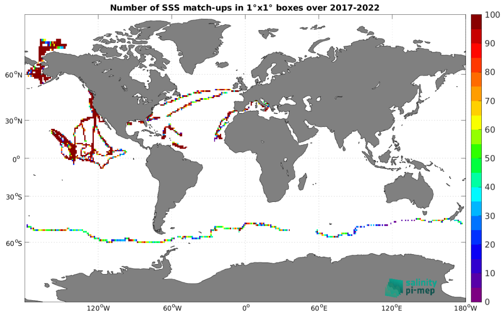
Figure 5: Number of SSS match-ups between Saifdrone SSS and the CCI SSS L4 Merged-OI v4.41 - 30-day running (ESA) SSS product for the Global Ocean Pi-MEP region over 1^\circ \times 1^\circ boxes and for the full satellite product period.
