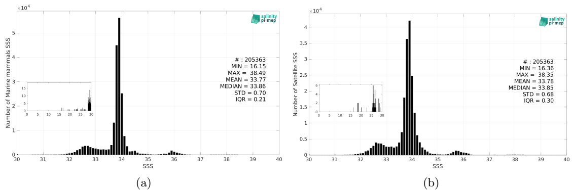
Figure 3: Histograms of SSS from Marine mammals (a) and CCI SSS L4 Merged-OI v4.41 - 30-day running (ESA) (b) considering all match-up pairs per bins of 0.1 over the Global Ocean Pi-MEP region and for the full satellite product period.
