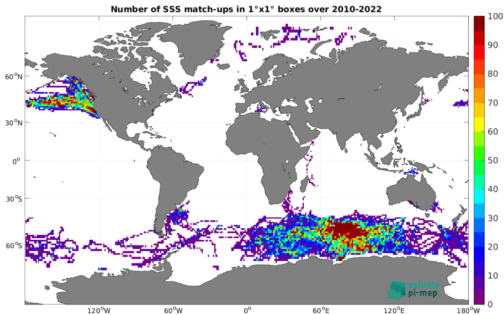
Figure 5: Number of SSS match-ups between Marine mammals SSS and the CCI SSS L4 Merged-OI v4.41 - 30-day running (ESA) SSS product for the Global Ocean Pi-MEP region over 1^\circ \times 1^\circ boxes and for the full satellite product period.
