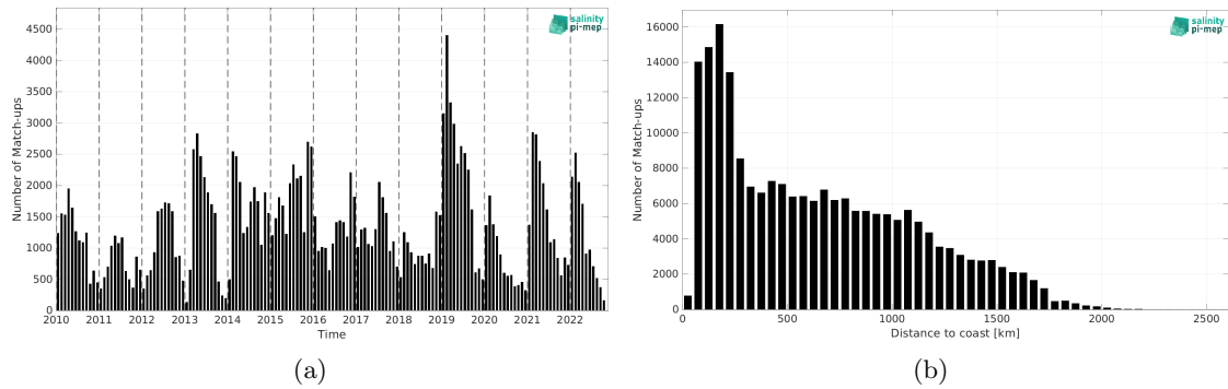
Figure 2: Number of match-ups between Marine mammals and CCI SSS L4 Merged-OI v4.41 - 30-day running (ESA) SSS as a function of time (a) and as function of the distance to coast (b) over the Global Ocean Pi-MEP region and for the full satellite product period.
