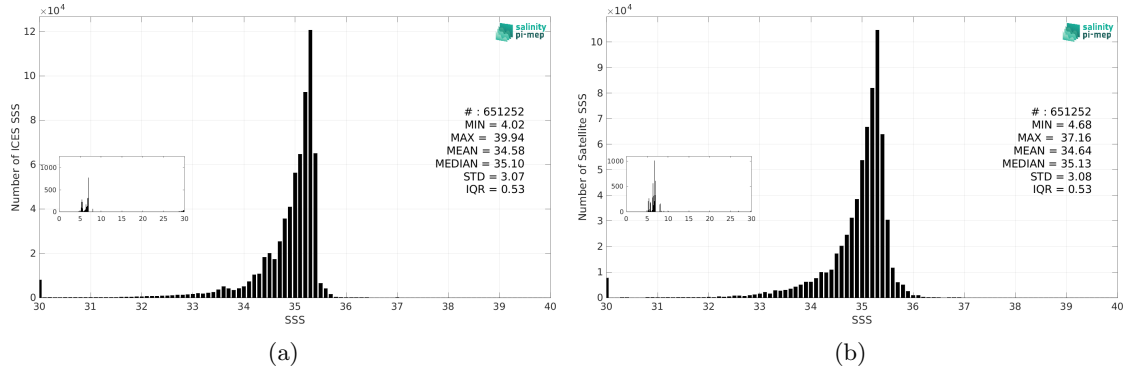
Figure 3: Histograms of SSS from ICES (a) and CCI SSS L4 Merged-OI v4.41 - 30-day running (ESA) (b) considering all match-up pairs per bins of 0.1 over the Global Ocean Pi-MEP region and for the full satellite product period.
