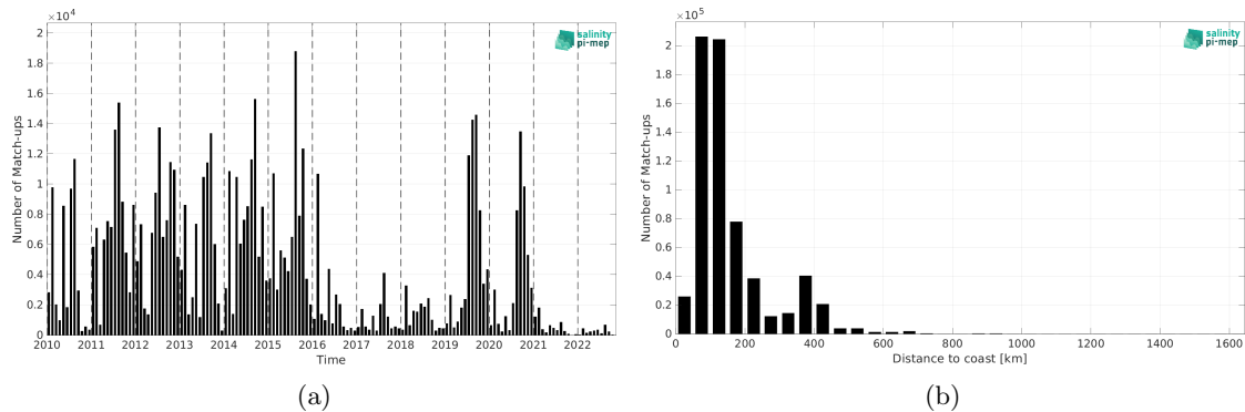
Figure 2: Number of match-ups between ICES and CCI SSS L4 Merged-OI v4.41 - 30-day running (ESA) SSS as a function of time (a) and as function of the distance to coast (b) over the Global Ocean Pi-MEP region and for the full satellite product period.
