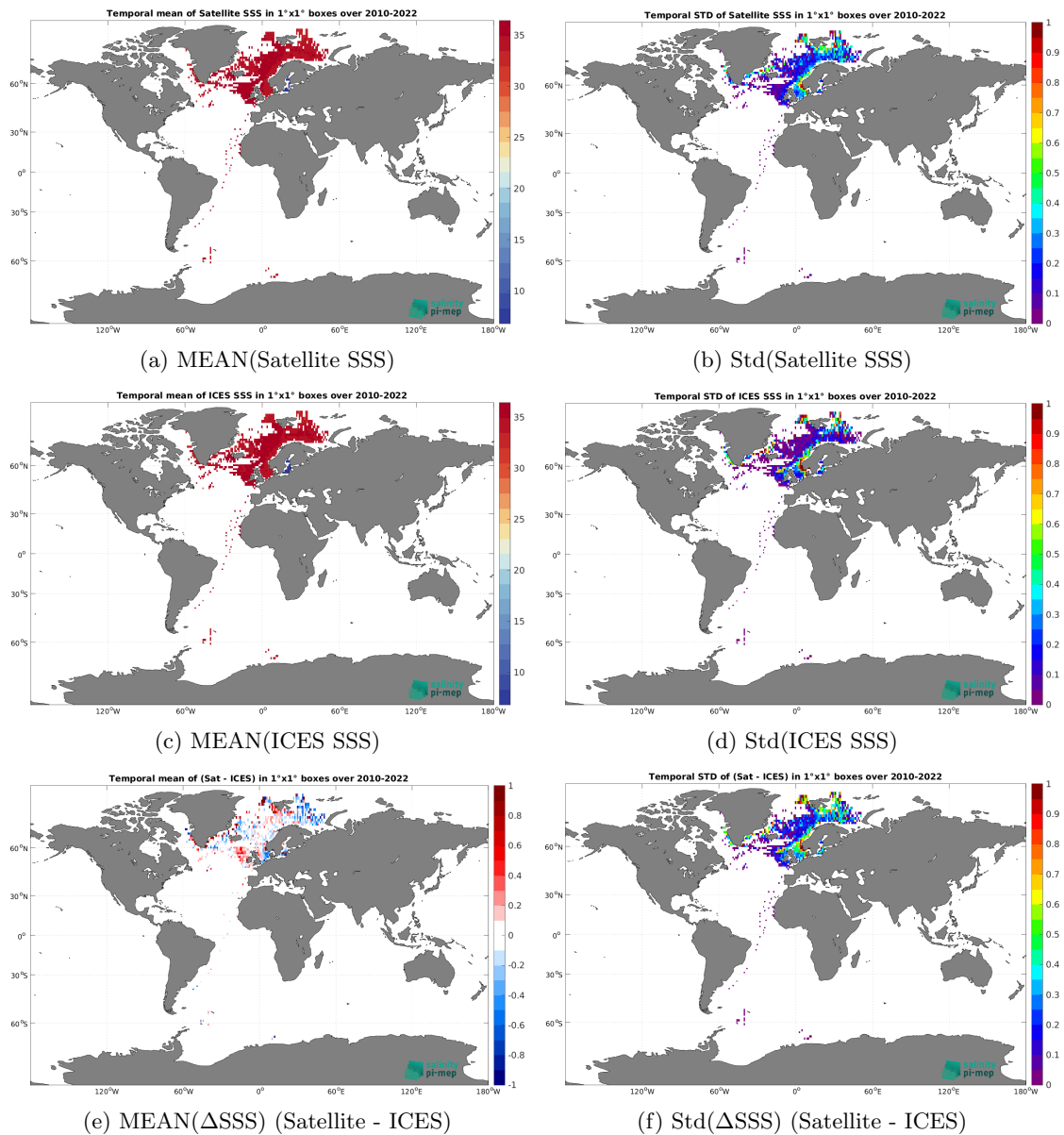
Figure 7: Temporal mean (left) and Std (right) of SSS from CCI SSS L4 Merged-OI v4.41 - 30-day running (ESA) (top), ICES (middle), and of \Delta SSS (Satellite - ICES). Only match-up pairs are used to generate these maps.
