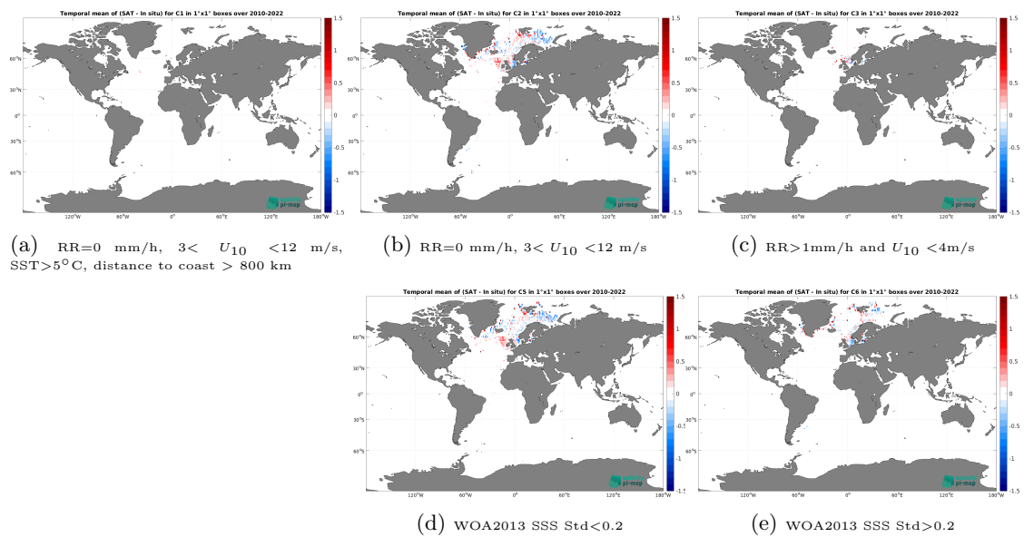
Figure 14: Temporal mean gridded over spatial boxes of size 1^\circ \times 1^\circ of \Delta SSS (CCI SSS L4 Merged-OI v4.41 - 30-day running (ESA) - ICES) for 5 different subdatasets corresponding to:RR=0 mm/h, 3 < U_{10} < 12 m/s, SST > 5^\circ\text{C} , distance to coast > 800 km (a), RR=0 mm/h, 3 < U_{10} < 12 m/s (b), RR > 1 mm/h and U_{10} < 4 m/s (c), WOA2013 SSS Std < 0.2 (d), WOA2013 SSS Std > 0.2 (e).
