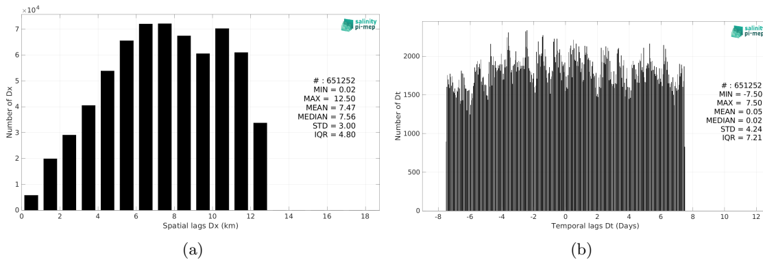
Figure 6: Histograms of the spatial (a) and temporal (b) lags between the location/time of the ICES measurement and the date of the corresponding CCI SSS L4 Merged-OI v4.41 - 30-day running (ESA) SSS pixel.
