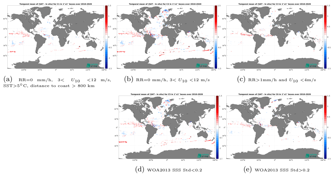
Figure 13: Temporal mean gridded over spatial boxes of size 1^\circ \times 1^\circ of \Delta\text{SSS} (CCI SSS L4 Merged-OI v4.41 - 30-day running (ESA) - Surface drifters) for 5 different subdatasets corresponding to:RR=0 mm/h, 3 < U_{10} < 12 m/s, SST > 5^\circ\text{C} , distance to coast > 800 km (a), RR=0 mm/h, 3 < U_{10} < 12 m/s (b), RR > 1 mm/h and U_{10} < 4 m/s (c), WOA2013 SSS Std < 0.2 (d), WOA2013 SSS Std > 0.2 (e).
