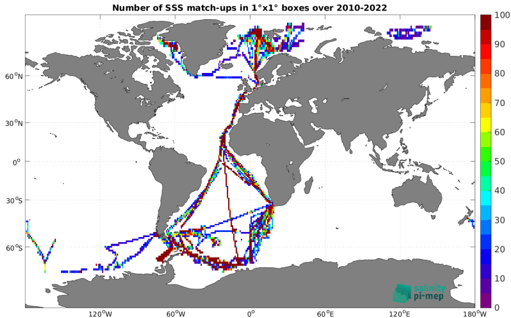
Figure 4: Number of SSS match-ups between TSG (Polarstern) SSS and the CCI SSS L4 Merged-OI v4.4 - 7-day running (ESA) SSS product for the Global Ocean Pi-MEP region over 1°x1° boxes and for the full satellite product period.
