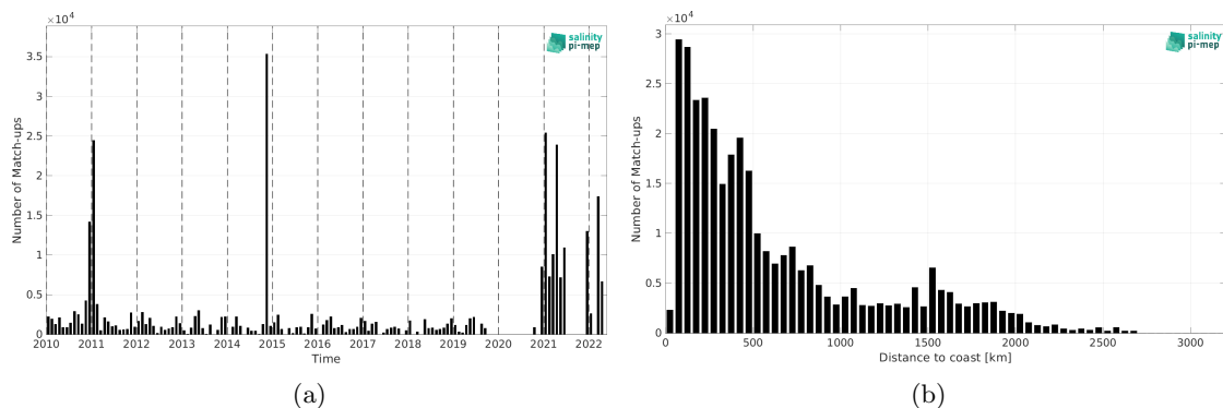
Figure 1: Number of match-ups between TSG (Polarstern) and CCI SSS L4 Merged-OI v4.4 - 7-day running (ESA) SSS as a function of time (a) and as function of the distance to coast (b) over the Global Ocean Pi-MEP region and for the full satellite product period.
