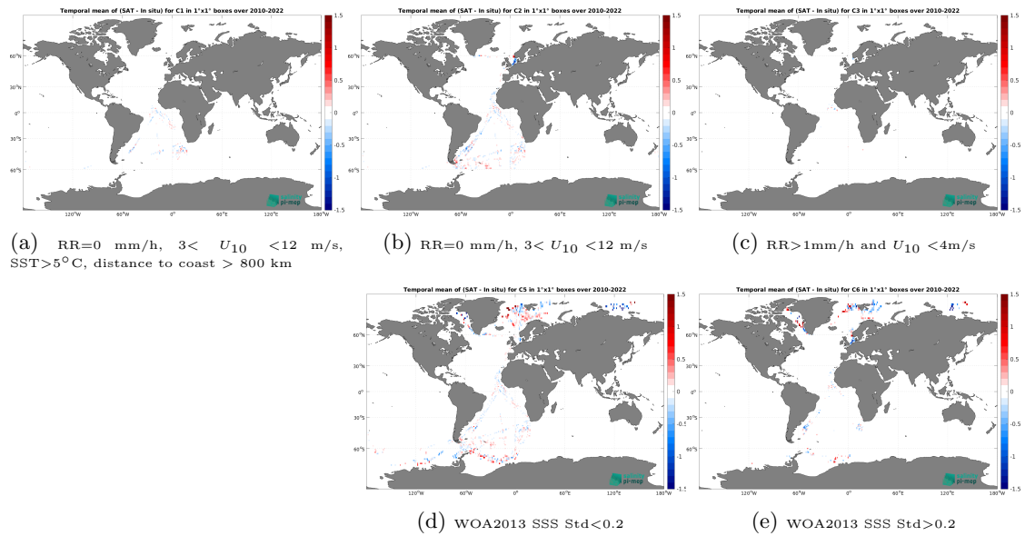
Figure 12: Temporal mean gridded over spatial boxes of size 1^\circ \times 1^\circ of \Delta SSS (CCI SSS L4 Merged-OI v4.4 - 7-day running (ESA) - TSG (Polarstern)) for 5 different subdatasets corresponding to: RR=0 mm/h, 3 < U_{10} < 12 m/s, SST > 5^\circ\text{C} , distance to coast > 800 km (a), RR=0 mm/h, 3 < U_{10} < 12 m/s (b), RR > 1\text{mm/h} and U_{10} < 4\text{m/s} (c), WOA2013 SSS Std < 0.2 (d), WOA2013 SSS Std > 0.2 (e).
