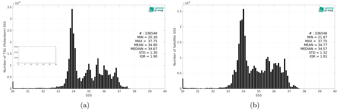
Figure 2: Histograms of SSS from TSG (Polarstern) (a) and CCI SSS L4 Merged-OI v4.4 - 7-day running (ESA) (b) considering all match-up pairs per bins of 0.1 over the Global Ocean Pi-MEP region and for the full satellite product period.
