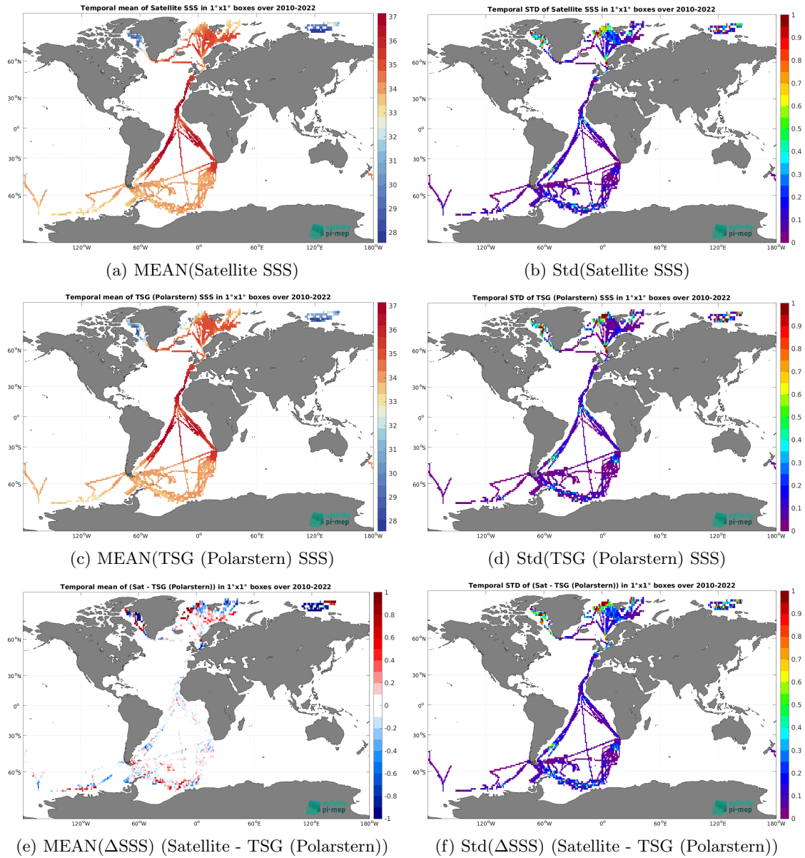
Figure 6: Temporal mean (left) and Std (right) of SSS from CCI SSS L4 Merged-OI v4.4 - 7-day running (ESA) (top), TSG (Polarstern) (middle), and of \Delta SSS (Satellite - TSG (Polarstern)). Only match-up pairs are used to generate these maps.
