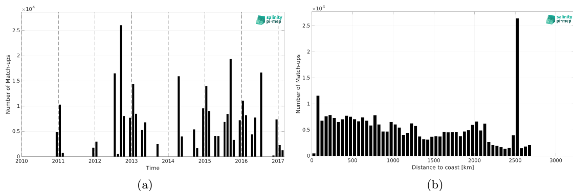
Figure 1: Number of match-ups between TSG (NCEI-0170743) and CCI SSS L4 Merged-OI v4.4 - 7-day running (ESA) SSS as a function of time (a) and as function of the distance to coast (b) over the Global Ocean Pi-MEP region and for the full satellite product period.
