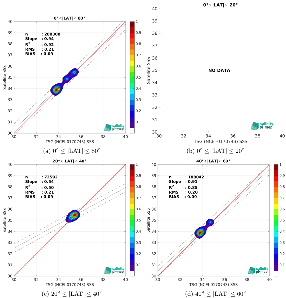
Figure 9: Contour maps of the concentration of CCI SSS L4 Merged-OI v4.4 - 7-day running (ESA) SSS (y-axis) versus TSG (NCEI-0170743) SSS (x-axis) at match-up pairs for different latitude bands. For each plot, the red line shows x=y . The black thin and dashed lines indicate a linear fit through the data cloud and the \pm 95\% confidence levels, respectively. The number match-up pairs n , the slope and R^2 coefficient of the linear fit, the root mean square (RMS) and the mean bias between satellite and in situ data are indicated for each latitude band in each plots.
