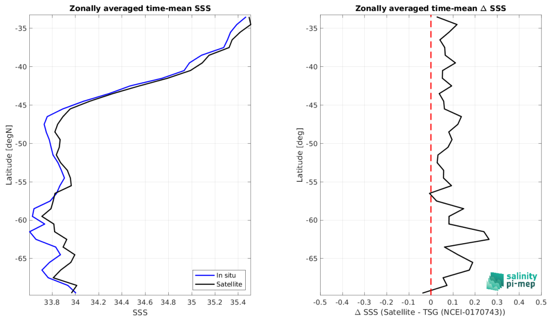
Figure 8: Left panel: Zonal mean SSS from CCI SSS L4 Merged-OI v4.4 - 7-day running (ESA) satellite product (black) and from TSG (NCEI-0170743) (blue). Right panel: Zonal mean of \Delta SSS (Satellite - TSG (NCEI-0170743)) for all the collected Pi-MEP match-up pairs estimated over the full satellite product period.
