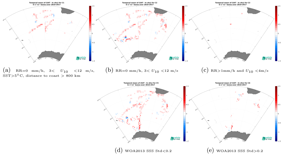
Figure 12: Temporal mean gridded over spatial boxes of size 1^{\circ}\times 1^{\circ} of \Delta\text{SSS} (CCI SSS L4 Merged-OI v4.4 - 7-day running (ESA) - TSG (NCEI-0170743)) for 5 different subdatasets corresponding to:RR=0 mm/h, 3 < U_{10} < 12 m/s, SST >5^{\circ}\text{C} , distance to coast > 800 km (a), RR=0 mm/h, 3 < U_{10} < 12 m/s (b), RR >1 mm/h and U_{10} < 4 m/s (c), WOA2013 SSS Std <0.2 (d), WOA2013 SSS Std >0.2 (e).
