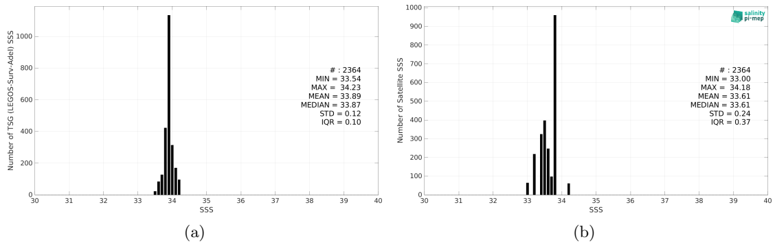
Figure 2: Histograms of SSS from TSG (LEGOS-Surv-Adel) (a) and CCI SSS L4 Merged-OI v4.4 - 7-day running (ESA) (b) considering all match-up pairs per bins of 0.1 over the Global Ocean Pi-MEP region and for the full satellite product period.
