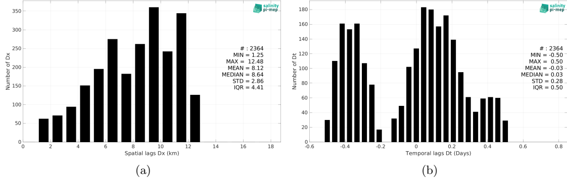
Figure 5: Histograms of the spatial (a) and temporal (b) lags between the location/time of the TSG (LEGOS-Surv-Adel) measurement and the date of the corresponding CCI SSS L4 Merged-OI v4.4 - 7-day running (ESA) SSS pixel.
