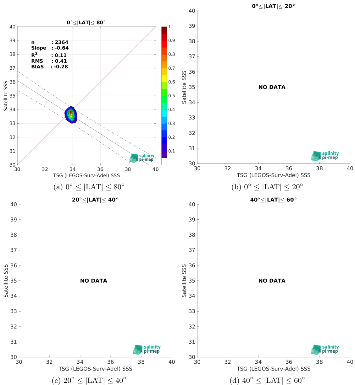
Figure 9: Contour maps of the concentration of CCI SSS L4 Merged-OI v4.4 - 7-day running (ESA) SSS (y-axis) versus TSG (LEGOS-Surv-Adel) SSS (x-axis) at match-up pairs for different latitude bands. For each plot, the red line shows x=y . The black thin and dashed lines indicate a linear fit through the data cloud and the \pm 95\% confidence levels, respectively. The number match-up pairs n , the slope and R^2 coefficient of the linear fit, the root mean square (RMS) and the mean bias between satellite and in situ data are indicated for each latitude band in each plots.
