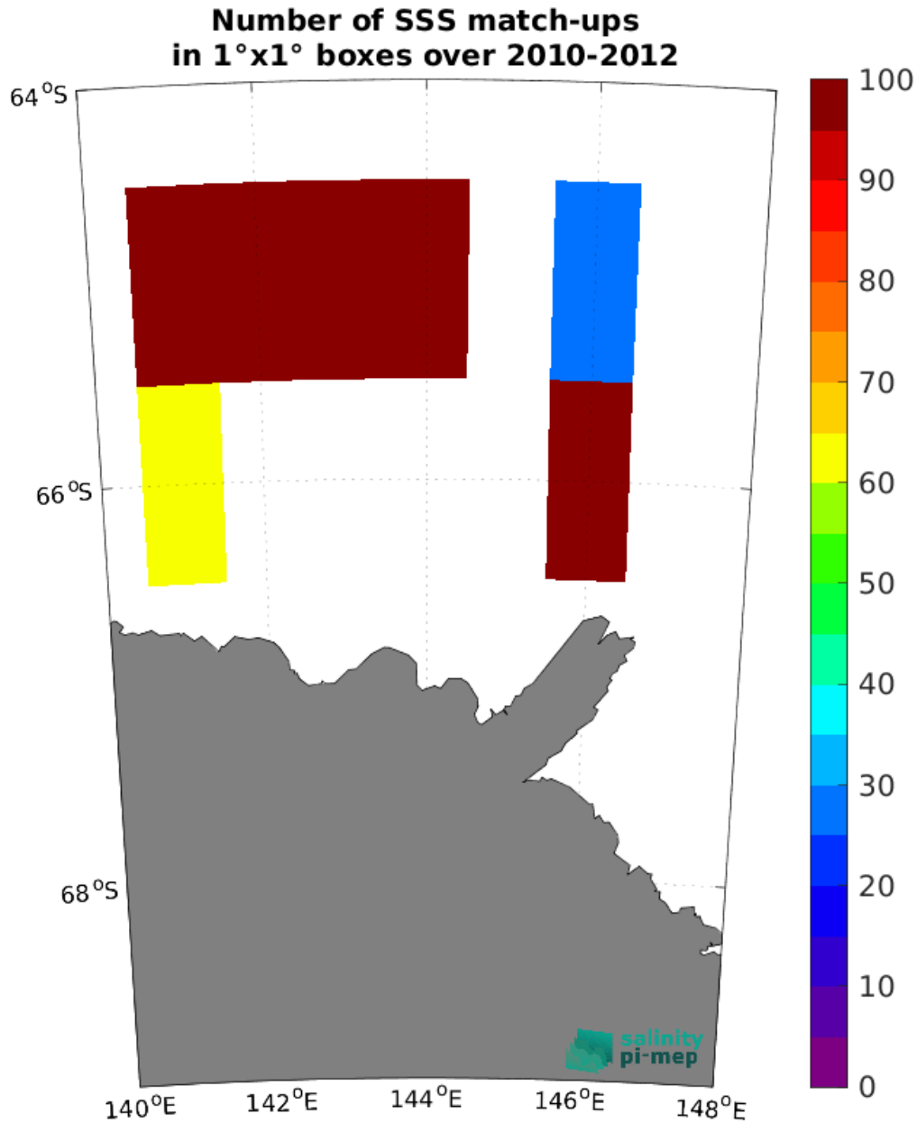
Figure 4: Number of SSS match-ups between TSG (LEGOS-Surv-Adel) SSS and the CCI SSS L4 Merged-OI v4.4 - 7-day running (ESA) SSS product for the Global Ocean Pi-MEP region over 1^\circ \times 1^\circ boxes and for the full satellite product period.
