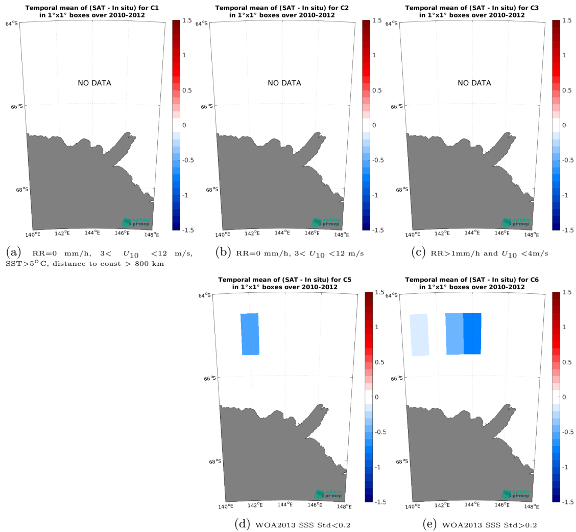
Figure 12: Temporal mean gridded over spatial boxes of size 1^\circ \times 1^\circ of \Delta\text{SSS} (CCI SSS L4 Merged-OI v4.4 - 7-day running (ESA) - TSG (LEGOS-Surv-Adel)) for 5 different subdatasets corresponding to: RR=0 mm/h, 3 < U_{10} < 12 m/s, SST > 5^\circ\text{C} , distance to coast > 800 km (a), RR=0 mm/h, 3 < U_{10} < 12 m/s (b), RR > 1\text{mm/h} and U_{10} < 4\text{m/s} (c), WOA2013 SSS Std < 0.2 (d), WOA2013 SSS Std > 0.2 (e).
