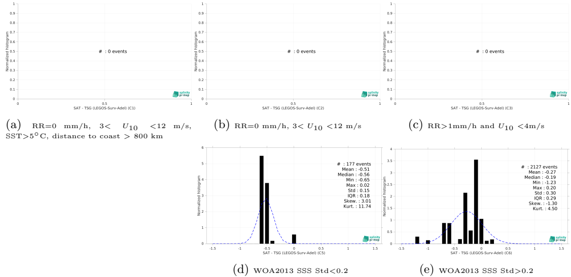
Figure 13: Normalized histogram of \Delta SSS (CCI SSS L4 Merged-OI v4.4 - 7-day running (ESA) - TSG (LEGOS-Surv-Adel)) for 5 different subdatasets corresponding to: RR=0 mm/h, 3 < U_{10} < 12 m/s, SST > 5°C, distance to coast > 800 km (a), RR=0 mm/h, 3 < U_{10} < 12 m/s (b), RR > 1mm/h and U_{10} < 4 m/s (c), WOA2013 SSS Std < 0.2 (d), WOA2013 SSS Std > 0.2 (e).
