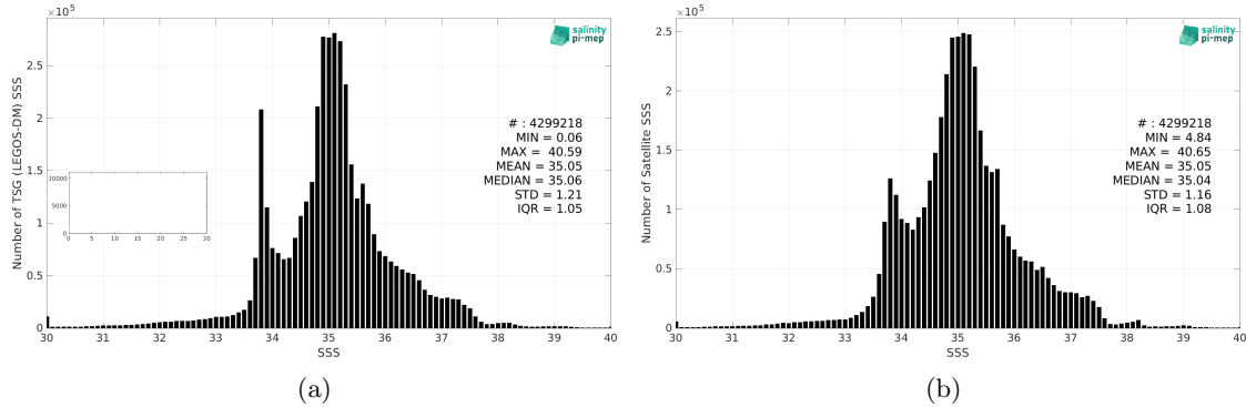
Figure 2: Histograms of SSS from TSG (LEGOS-DM) (a) and CCI SSS L4 Merged-OI v4.4 - 7-day running (ESA) (b) considering all match-up pairs per bins of 0.1 over the Global Ocean Pi-MEP region and for the full satellite product period.
