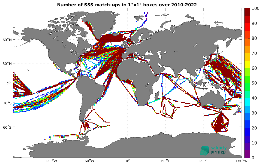
Figure 4: Number of SSS match-ups between TSG (LEGOS-DM) SSS and the CCI SSS L4 Merged-OI v4.4 - 7-day running (ESA) SSS product for the Global Ocean Pi-MEP region over 1^\circ \times 1^\circ boxes and for the full satellite product period.
