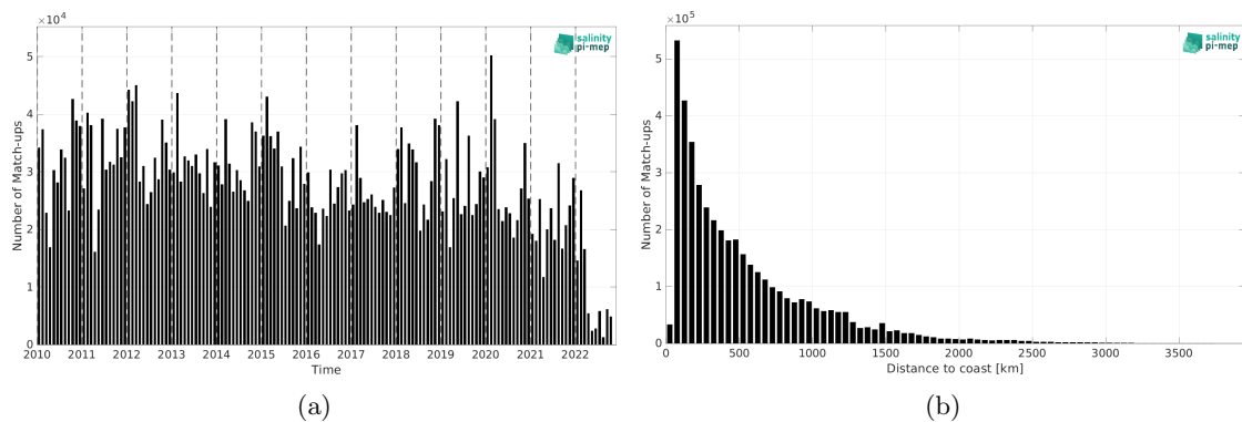
Figure 1: Number of match-ups between TSG (LEGOS-DM) and CCI SSS L4 Merged-OI v4.4 - 7-day running (ESA) SSS as a function of time (a) and as function of the distance to coast (b) over the Global Ocean Pi-MEP region and for the full satellite product period.
