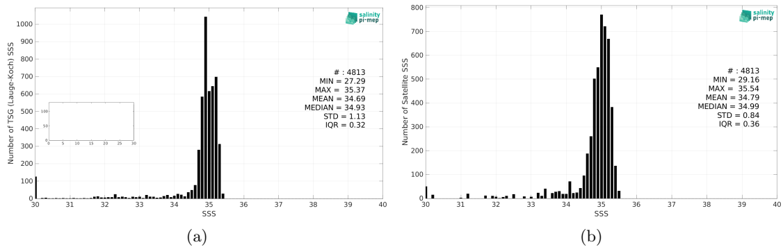
Figure 2: Histograms of SSS from TSG (Lauge-Koch) (a) and CCI SSS L4 Merged-OI v4.4 - 7-day running (ESA) (b) considering all match-up pairs per bins of 0.1 over the Global Ocean Pi-MEP region and for the full satellite product period.
