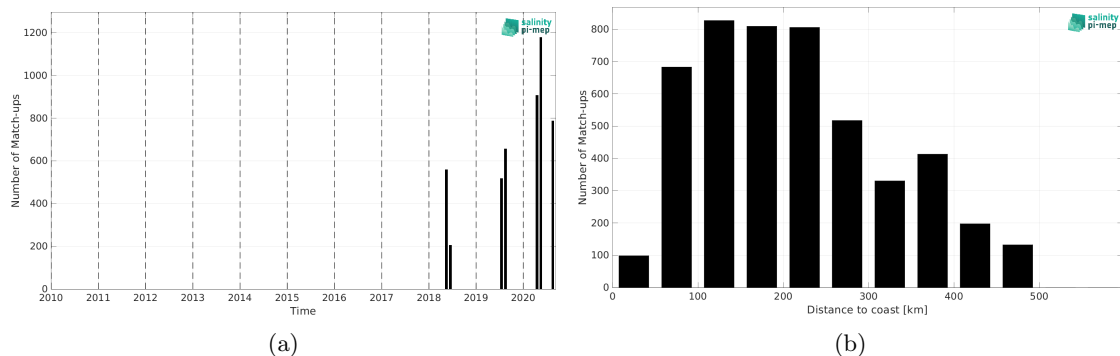
Figure 1: Number of match-ups between TSG (Lauge-Koch) and CCI SSS L4 Merged-OI v4.4 - 7-day running (ESA) SSS as a function of time (a) and as function of the distance to coast (b) over the Global Ocean Pi-MEP region and for the full satellite product period.
