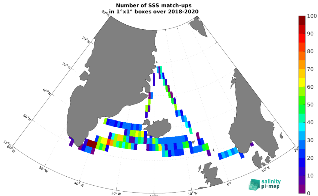
Figure 4: Number of SSS match-ups between TSG (Lauge-Koch) SSS and the CCI SSS L4 Merged-OI v4.4 - 7-day running (ESA) SSS product for the Global Ocean Pi-MEP region over 1^\circ \times 1^\circ boxes and for the full satellite product period.
