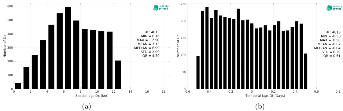
Figure 5: Histograms of the spatial (a) and temporal (b) lags between the location/time of the TSG (Lauge-Koch) measurement and the date of the corresponding CCI SSS L4 Merged-OI v4.4 - 7-day running (ESA) SSS pixel.
