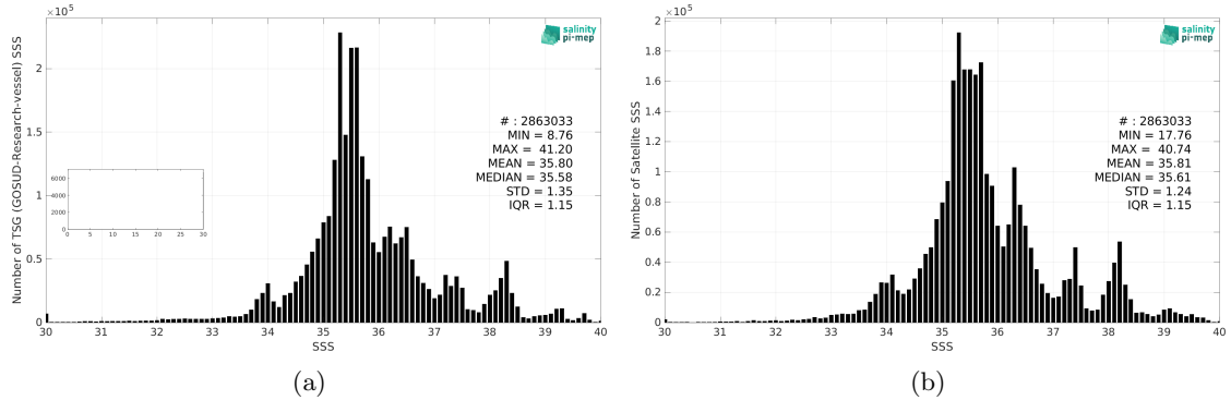
Figure 2: Histograms of SSS from TSG (GOSUD-Research-vessel) (a) and CCI SSS L4 Merged-OI v4.4 - 7-day running (ESA) (b) considering all match-up pairs per bins of 0.1 over the Global Ocean Pi-MEP region and for the full satellite product period.
