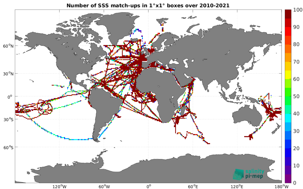
Figure 4: Number of SSS match-ups between TSG (GOSUD-Research-vessel) SSS and the CCI SSS L4 Merged-OI v4.4 - 7-day running (ESA) SSS product for the Global Ocean Pi-MEP region over 1^\circ \times 1^\circ boxes and for the full satellite product period.
