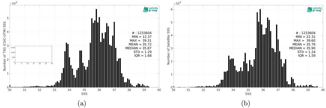
Figure 2: Histograms of SSS from TSG (CSIC-UTM) (a) and CCI SSS L4 Merged-OI v4.4 - 7-day running (ESA) (b) considering all match-up pairs per bins of 0.1 over the Global Ocean Pi-MEP region and for the full satellite product period.
