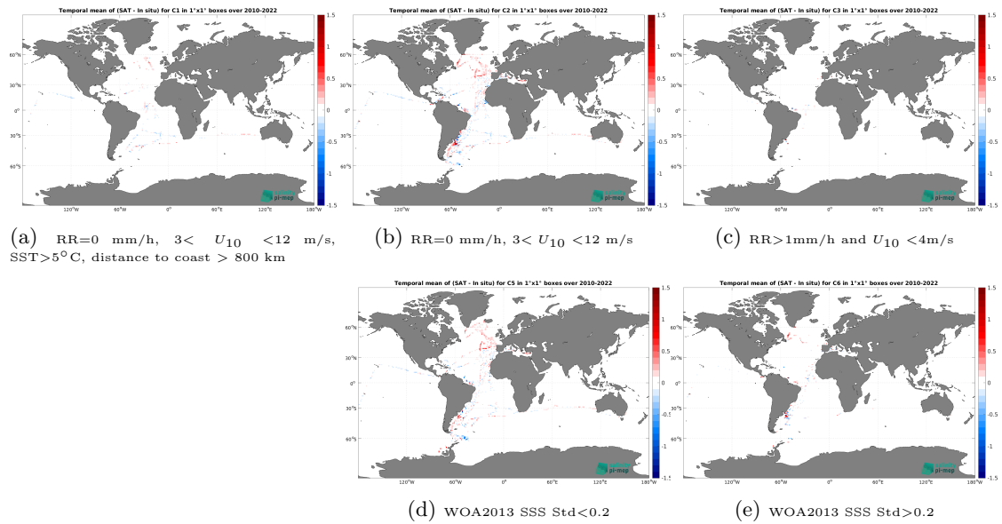
Figure 12: Temporal mean gridded over spatial boxes of size 1^\circ \times 1^\circ of \Delta\text{SSS} (CCI SSS L4 Merged-OI v4.4 - 7-day running (ESA) - TSG (CSIC-UTM)) for 5 different subdatasets corresponding to: RR=0 mm/h, 3 < U_{10} < 12 m/s, SST > 5^\circ\text{C} , distance to coast > 800 km (a), RR=0 mm/h, 3 < U_{10} < 12 m/s (b), RR > 1\text{mm/h} and U_{10} < 4\text{m/s} (c), WOA2013 SSS Std < 0.2 (d), WOA2013 SSS Std > 0.2 (e).
