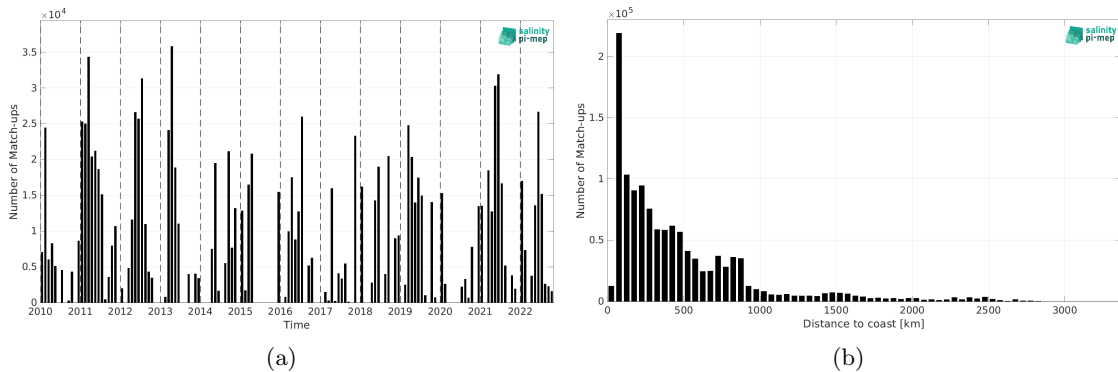
Figure 1: Number of match-ups between TSG (CSIC-UTM) and CCI SSS L4 Merged-OI v4.4 - 7-day running (ESA) SSS as a function of time (a) and as function of the distance to coast (b) over the Global Ocean Pi-MEP region and for the full satellite product period.
