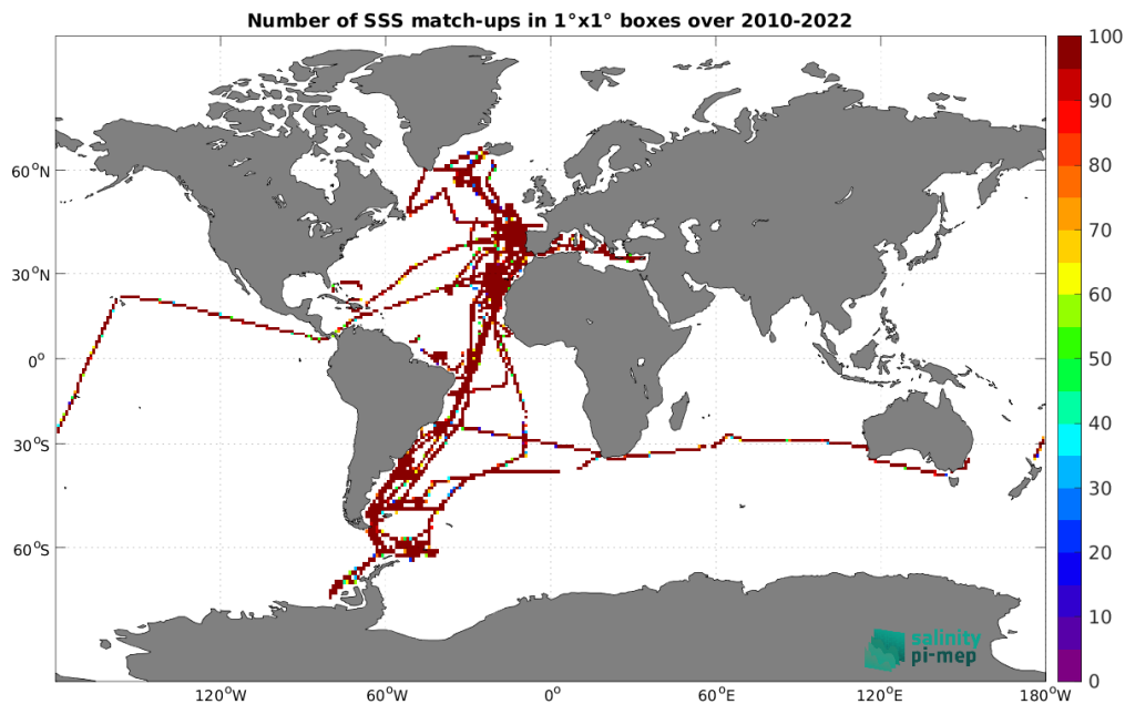
Figure 4: Number of SSS match-ups between TSG (CSIC-UTM) SSS and the CCI SSS L4 Merged-OI v4.4 - 7-day running (ESA) SSS product for the Global Ocean Pi-MEP region over 1^\circ \times 1^\circ boxes and for the full satellite product period.
