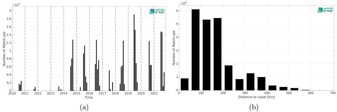
Figure 1: Number of match-ups between TSG (Amundsen) and CCI SSS L4 Merged-OI v4.4 - 7-day running (ESA) SSS as a function of time (a) and as function of the distance to coast (b) over the Global Ocean Pi-MEP region and for the full satellite product period.
