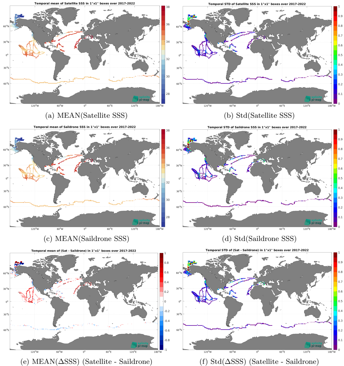
Figure 6: Temporal mean (left) and Std (right) of SSS from CCI SSS L4 Merged-OI v4.4 - 7-day running (ESA) (top), Saildrone (middle), and of \Delta SSS (Satellite - Saildrone). Only match-up pairs are used to generate these maps.
