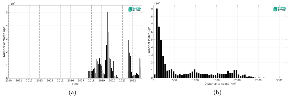
Figure 1: Number of match-ups between Saildrone and CCI SSS L4 Merged-OI v4.4 - 7-day running (ESA) SSS as a function of time (a) and as function of the distance to coast (b) over the Global Ocean Pi-MEP region and for the full satellite product period.
