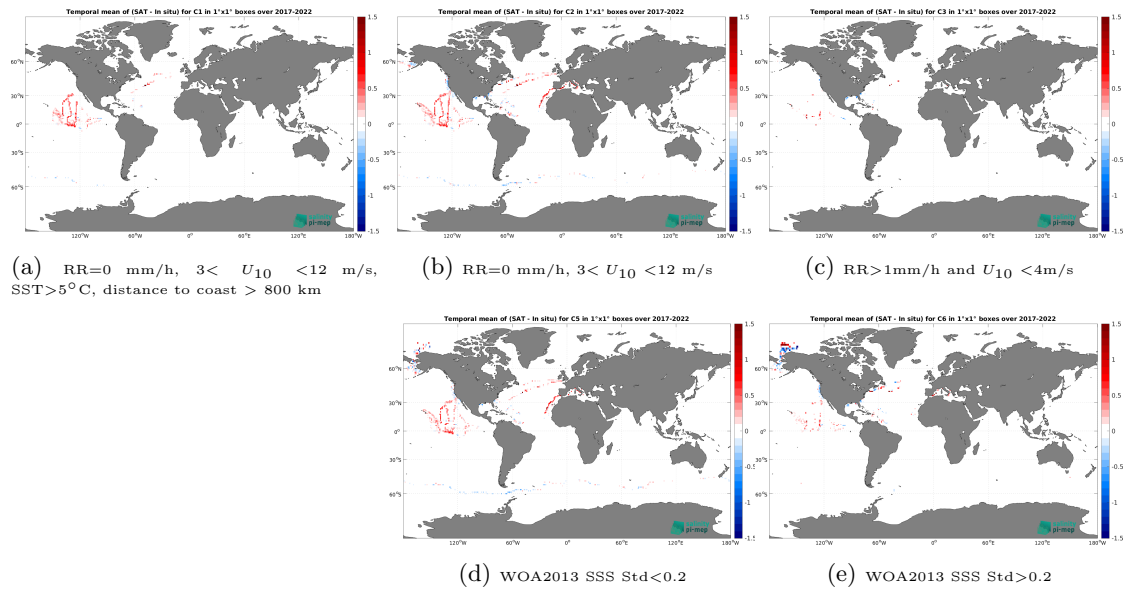
Figure 12: Temporal mean gridded over spatial boxes of size 1^\circ \times 1^\circ of \Delta\text{SSS} (CCI SSS L4 Merged-OI v4.4 - 7-day running (ESA) - Sailldrone) for 5 different subdatasets corresponding to:RR=0 mm/h, 3 < U_{10} < 12 m/s, SST > 5^\circ\text{C} , distance to coast > 800 km (a), RR=0 mm/h, 3 < U_{10} < 12 m/s (b), RR > 1\text{mm/h} and U_{10} < 4\text{m/s} (c), WOA2013 SSS Std < 0.2 (d), WOA2013 SSS Std > 0.2 (e).
