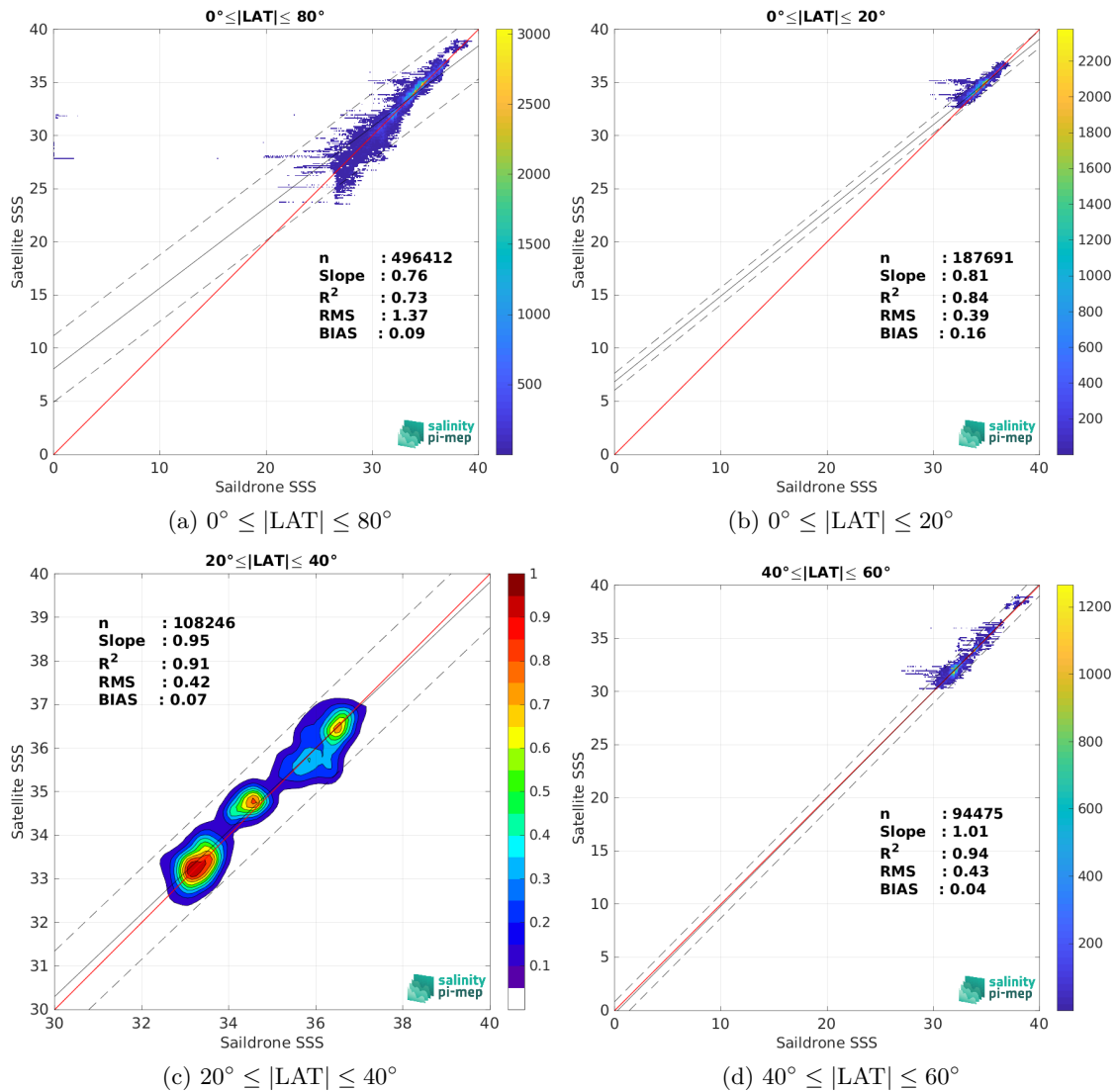
Figure 9: Contour maps of the concentration of CCI SSS L4 Merged-OI v4.4 - 7-day running (ESA) SSS (y-axis) versus Saildrone SSS (x-axis) at match-up pairs for different latitude bands. For each plot, the red line shows x=y . The black thin and dashed lines indicate a linear fit through the data cloud and the \pm 95\% confidence levels, respectively. The number match-up pairs n , the slope and R^2 coefficient of the linear fit, the root mean square (RMS) and the mean bias between satellite and in situ data are indicated for each latitude band in each plots.
