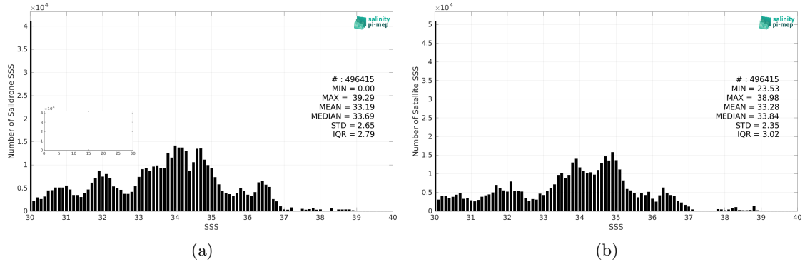
Figure 2: Histograms of SSS from Saildrone (a) and CCI SSS L4 Merged-OI v4.4 - 7-day running (ESA) (b) considering all match-up pairs per bins of 0.1 over the Global Ocean Pi-MEP region and for the full satellite product period.
