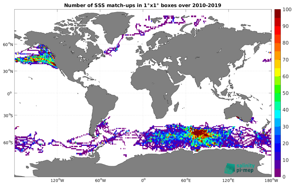
Figure 4: Number of SSS match-ups between Marine mammals SSS and the CCI SSS L4 Merged-OI v4.4 - 7-day running (ESA) SSS product for the Global Ocean Pi-MEP region over 1^\circ \times 1^\circ boxes and for the full satellite product period.
