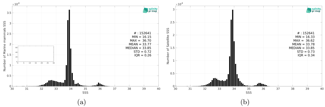
Figure 2: Histograms of SSS from Marine mammals (a) and CCI SSS L4 Merged-OI v4.4 - 7-day running (ESA) (b) considering all match-up pairs per bins of 0.1 over the Global Ocean Pi-MEP region and for the full satellite product period.
