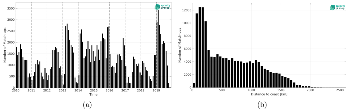
Figure 1: Number of match-ups between Marine mammals and CCI SSS L4 Merged-OI v4.4 - 7-day running (ESA) SSS as a function of time (a) and as function of the distance to coast (b) over the Global Ocean Pi-MEP region and for the full satellite product period.
