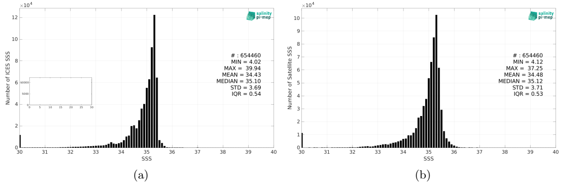
Figure 2: Histograms of SSS from ICES (a) and CCI SSS L4 Merged-OI v4.4 - 7-day running (ESA) (b) considering all match-up pairs per bins of 0.1 over the Global Ocean Pi-MEP region and for the full satellite product period.
