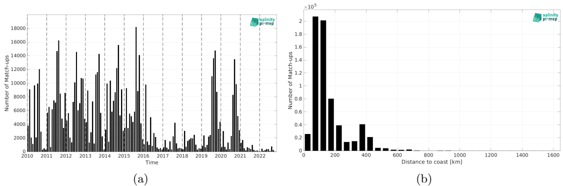
Figure 1: Number of match-ups between ICES and CCI SSS L4 Merged-OI v4.4 - 7-day running (ESA) SSS as a function of time (a) and as function of the distance to coast (b) over the Global Ocean Pi-MEP region and for the full satellite product period.
