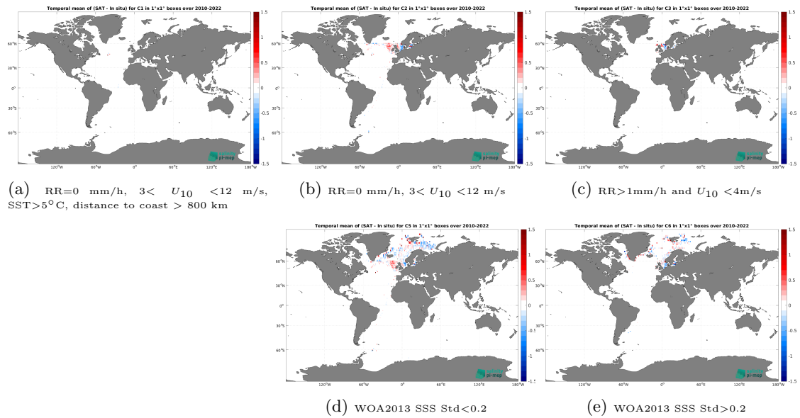
Figure 12: Temporal mean gridded over spatial boxes of size 1^\circ \times 1^\circ of \Delta SSS (CCI SSS L4 Merged-OI v4.4 - 7-day running (ESA) - ICES) for 5 different subdatasets corresponding to:RR=0 mm/h, 3 < U_{10} < 12 m/s, SST >5^\circ C, distance to coast > 800 km (a), RR=0 mm/h, 3 < U_{10} < 12 m/s (b), RR >1 mm/h and U_{10} < 4 m/s (c), WOA2013 SSS Std <0.2 (d), WOA2013 SSS Std >0.2 (e).
