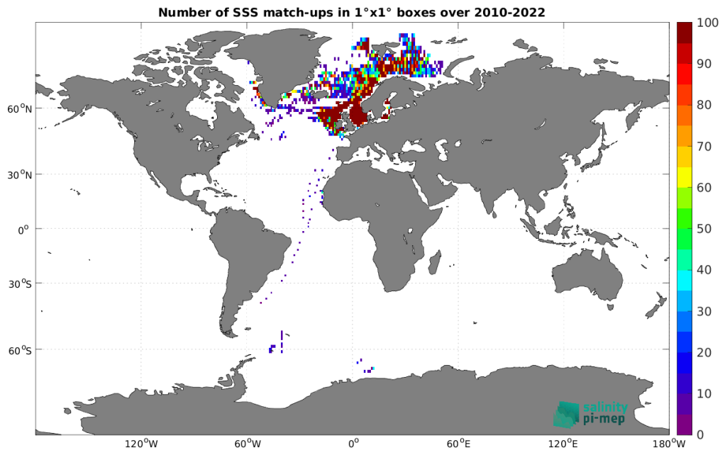
Figure 4: Number of SSS match-ups between ICES SSS and the CCI SSS L4 Merged-OI v4.4 - 7-day running (ESA) SSS product for the Global Ocean Pi-MEP region over 1^\circ \times 1^\circ boxes and for the full satellite product period.
