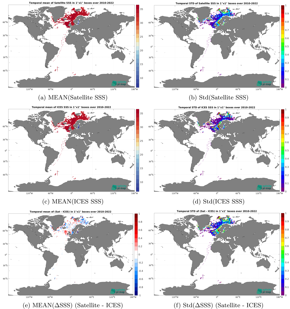
Figure 6: Temporal mean (left) and Std (right) of SSS from CCI SSS L4 Merged-OI v4.4 - 7-day running (ESA) (top), ICES (middle), and of \Delta SSS (Satellite - ICES). Only match-up pairs are used to generate these maps.
